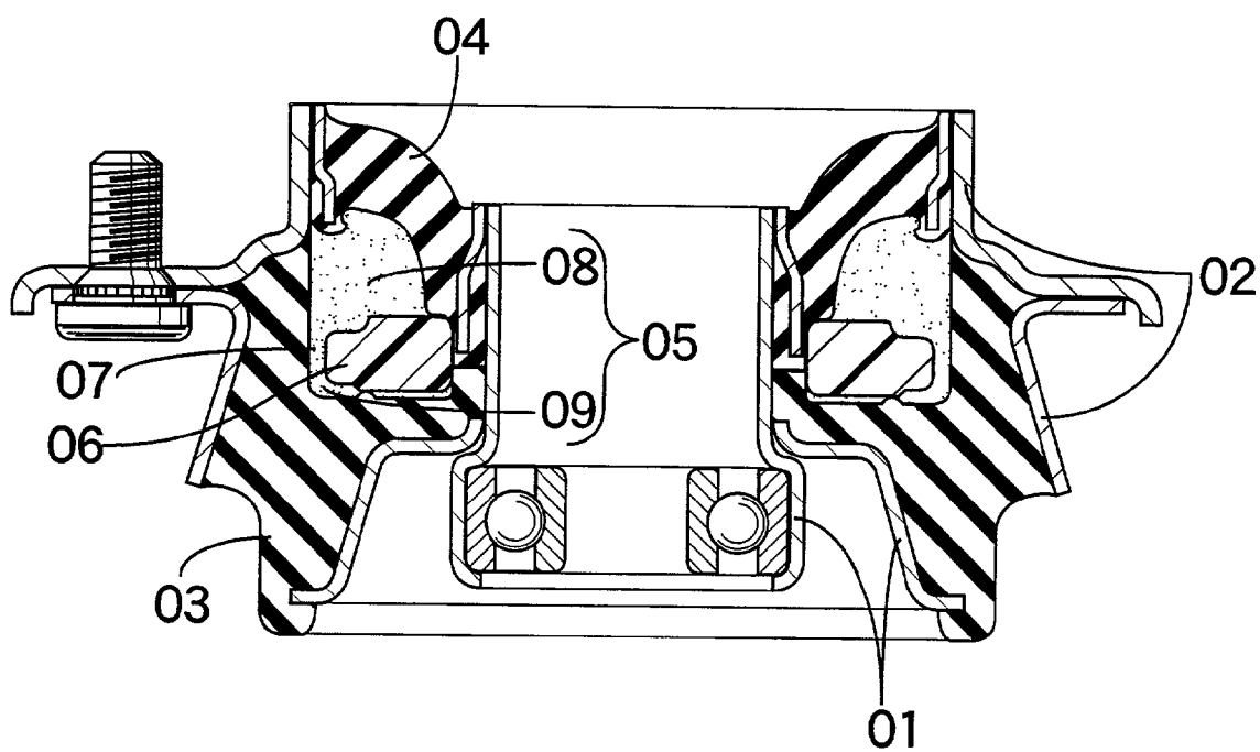
FIG.14 PRIOR ART
