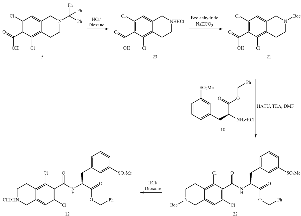
Scheme 6
