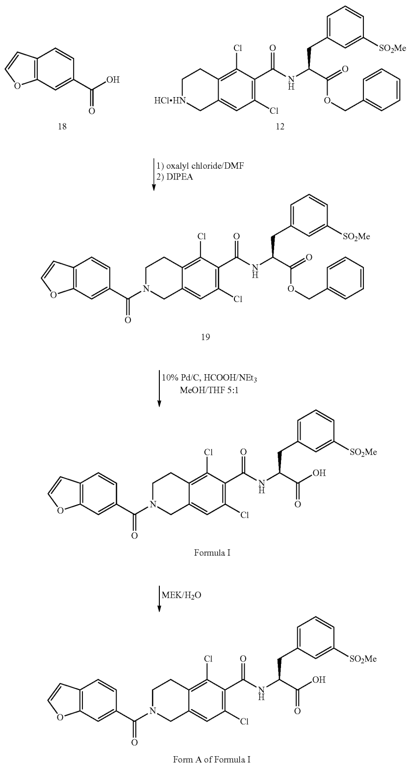
Scheme 5
