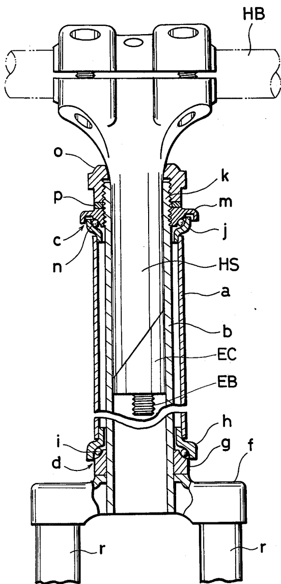
FIG. 6 PRIOR ART
