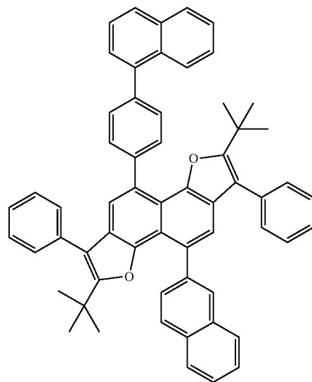
Compound 19
