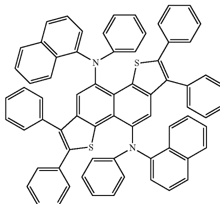
Compound 29
