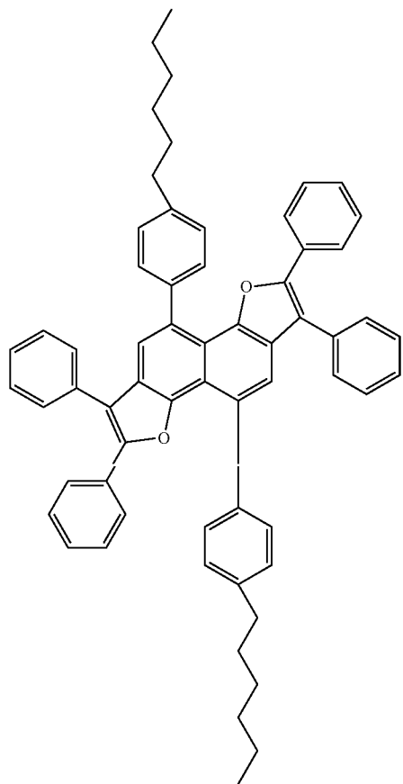
Compound 17
