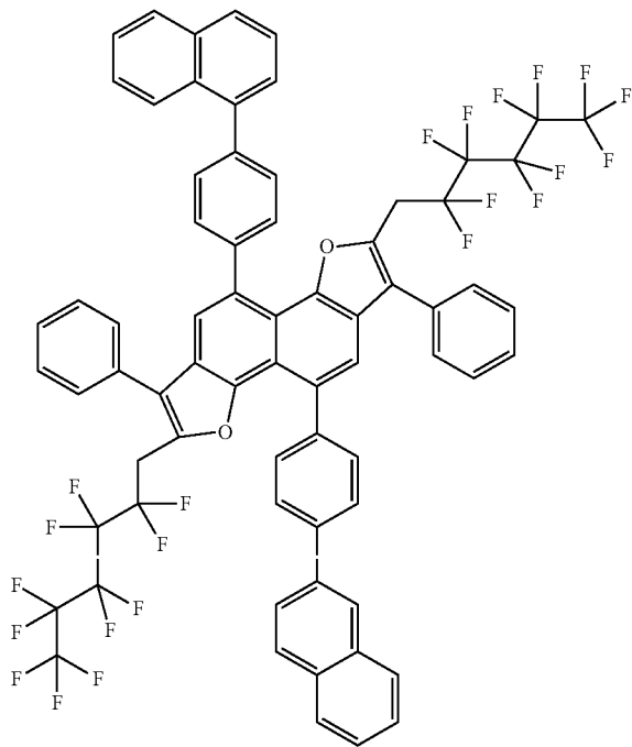
Compound 16
