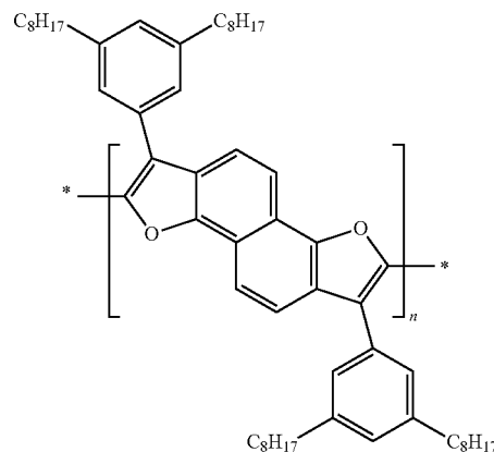
Compound 39
