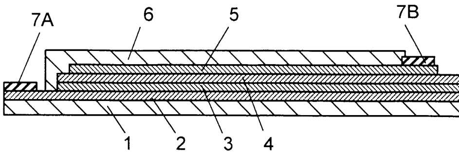
FIG. 9 PRIOR ART
