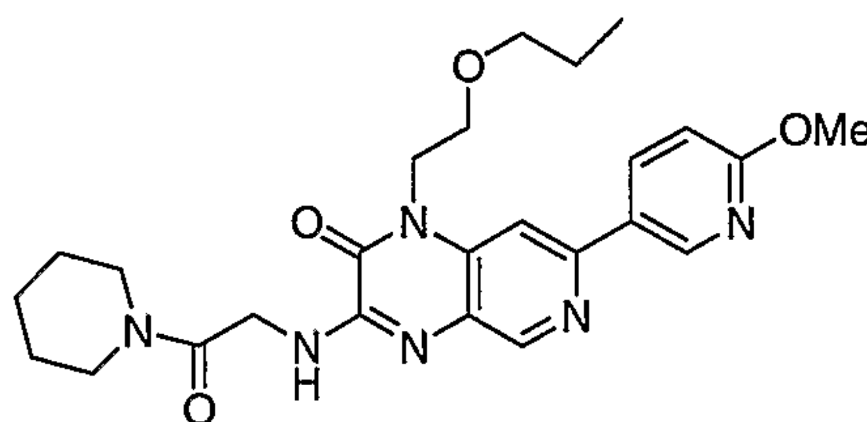
3-(2-oxo-2-(piperidin-1-yl)ethylamino)-7-(6-methoxypyridin-3-yl)-1-(2-propoxyethyl)pyrido[3,4-b]pyrazin-2(1H)-one
