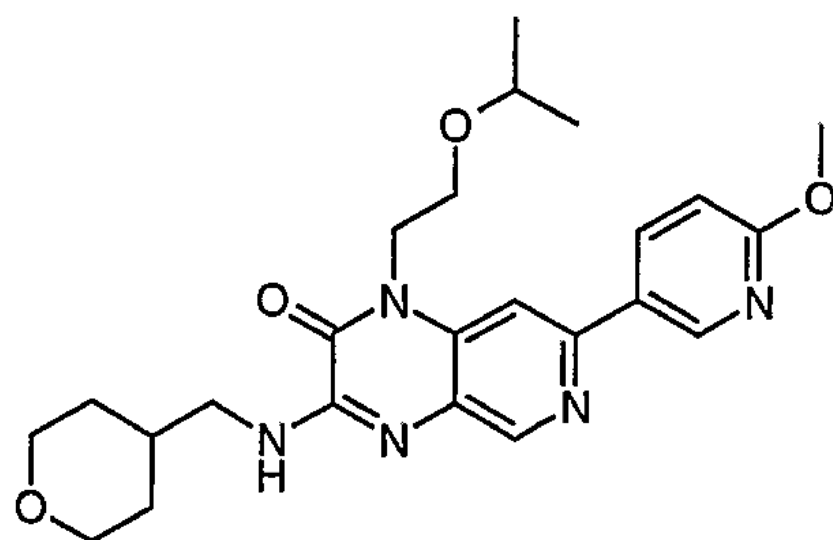
1-(2-isopropoxyethyl)-7-(6-methoxypyridin-3-yl)-3-[(tetrahydro-2H-pyran-4-yl)methyl]amino]pyrido[3,4-b]pyrazin-2(1H)-one.
