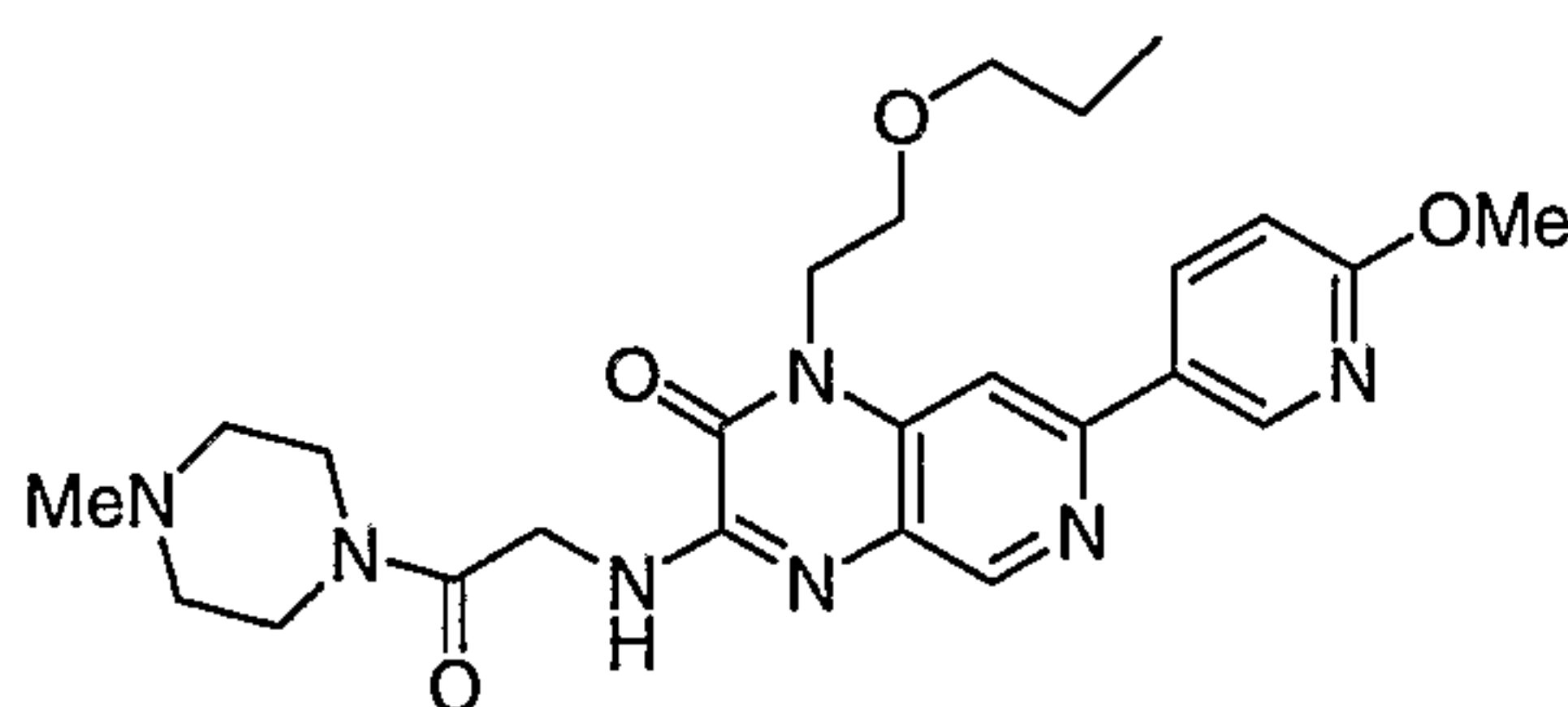
3-(2-(4-methylpiperazin-1-yl)-2-oxoethylamino)-7-(6-methoxypyridin-3-yl)-1-(2-propoxyethyl)pyrido[3,4-b]pyrazin-2(1H)-one
