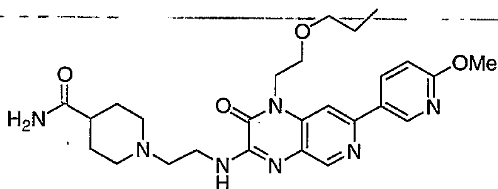
1-(2-(1,2-dihydro-7-(6-methoxypyridin-3-yl)-2-oxo-1-(2-propoxyethyl)pyrido[3,4-b]pyrazin-3-ylamino)ethyl)piperidine-4-carboxamide
