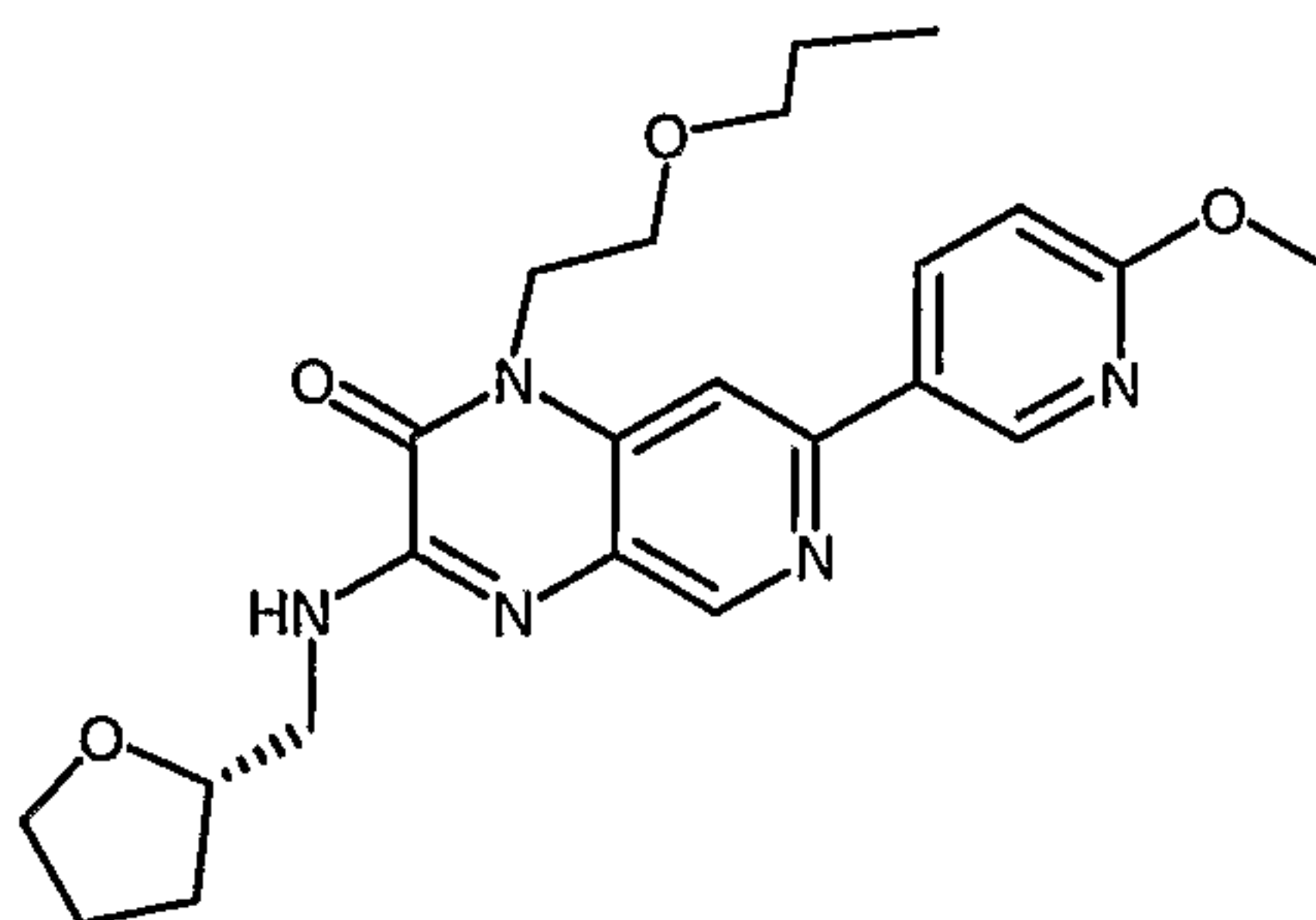
7-(6-methoxypyridin-3-yl)-1-(2-propoxyethyl)-3-[(2S)-tetrahydrofuran-2-ylmethyl]amino}pyrido[3,4-b]pyrazin-2(1H)-one
