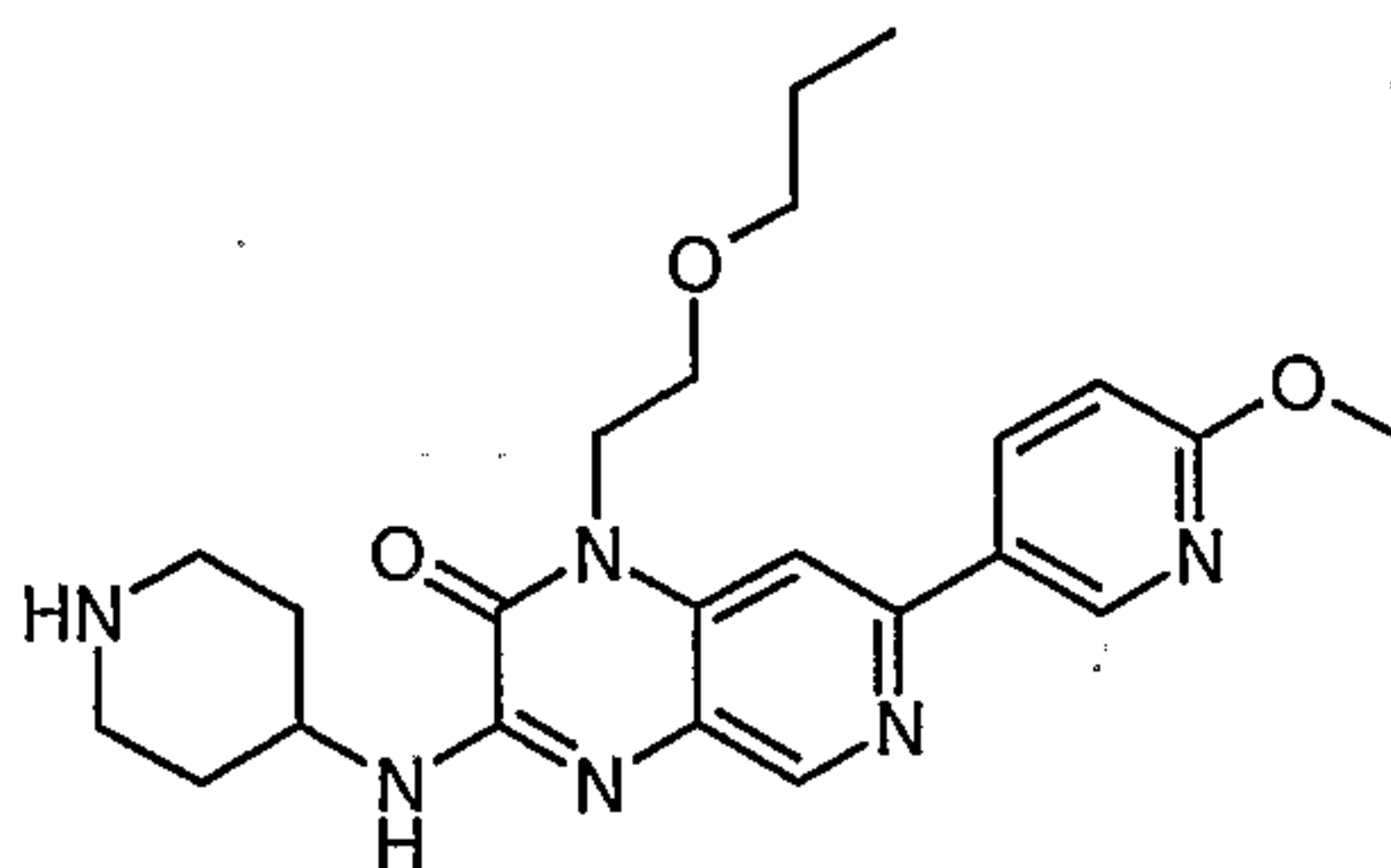
7-(6-methoxypyridin-3-yl)-3-(piperidin-4-ylamino)-1-(2-propoxyethyl)pyrido[3,4-b]pyrazin-2(1H)-one.
