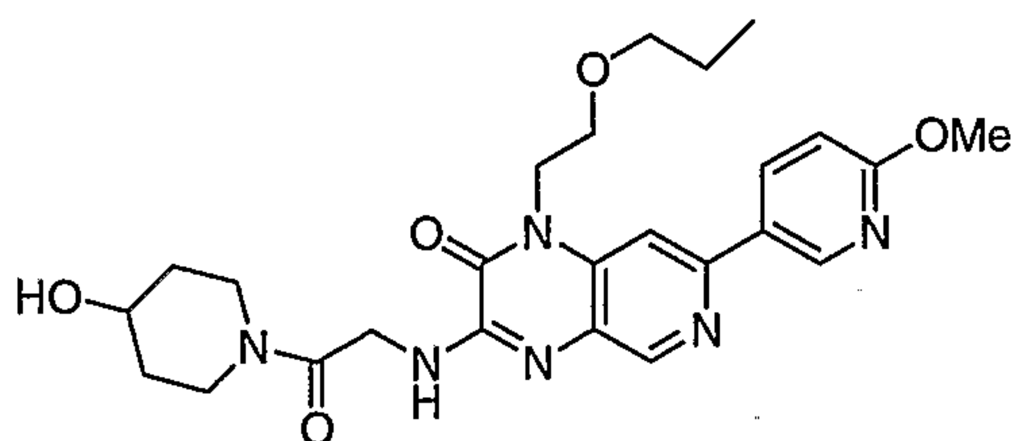
3-(2-(4-hydroxypiperidin-1-yl)-2-oxoethylamino)-7-(6-methoxypyridin-3-yl)-1-(2-propoxyethyl)pyrido[3,4-b]pyrazin-2(1H)-one
