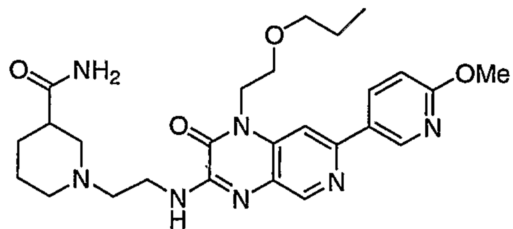
1-(2-(1,2-dihydro-7-(6-methoxypyridin-3-yl)-2-oxo-1-(2-propoxyethyl)pyrido[3,4-b]pyrazin-3-ylamino)ethyl)piperidine-3-carboxamide
