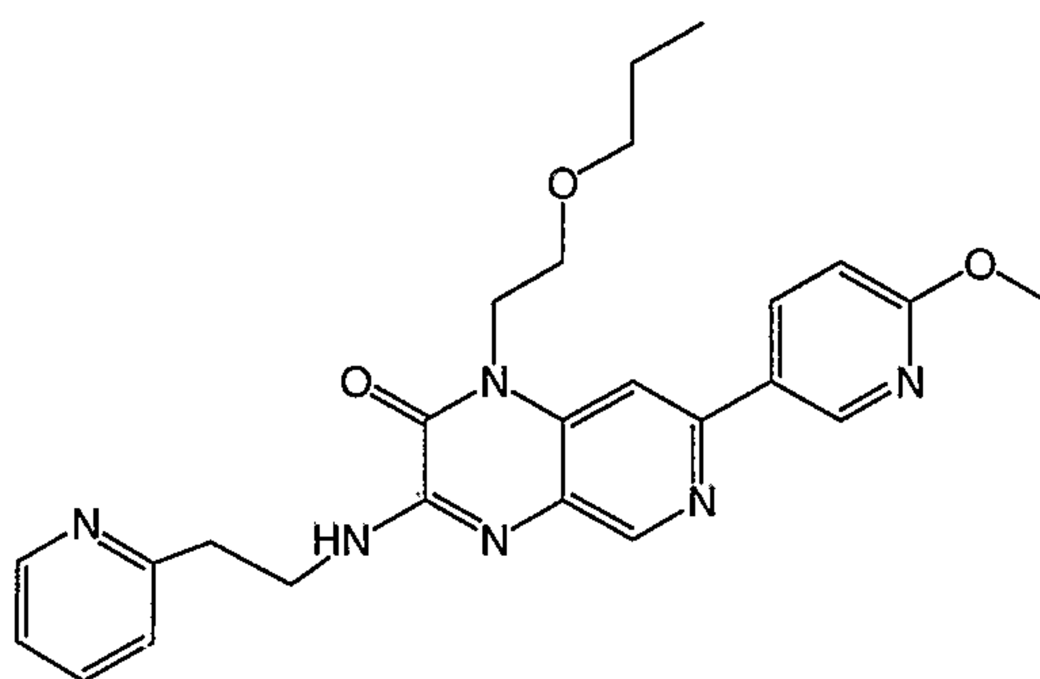
7-(6-methoxypyridin-3-yl)-1-(2-propoxyethyl)-3-[(2-pyridin-2-ylethyl)amino]pyrido[3,4-b]pyrazin-2(1H)-one.
