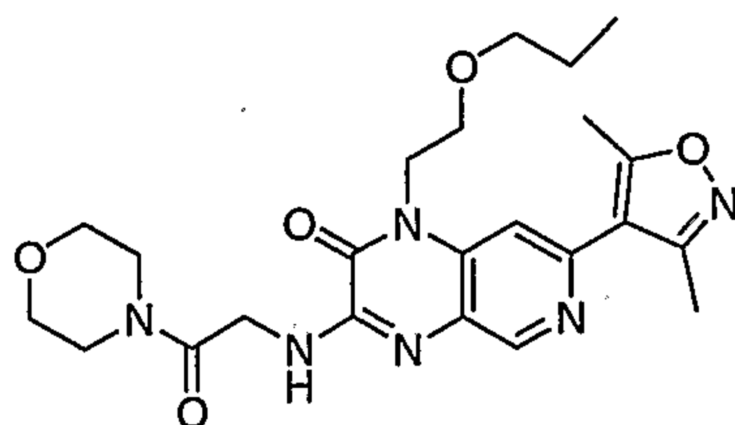
3-(2-morpholino-2-oxoethylamino)-7-(3,5-dimethylisoxazol-4-yl)-1-(2-propoxyethyl)pyrido[3,4-b]pyrazin-2(1H)-one
