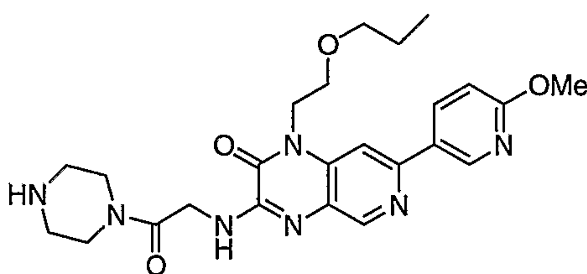
3-(2-oxo-2-(piperazin-1-yl)ethylamino)-7-(6-methoxypyridin-3-yl)-1-(2-propoxyethyl)pyrido[3,4-b]pyrazin-2(1H)-one
