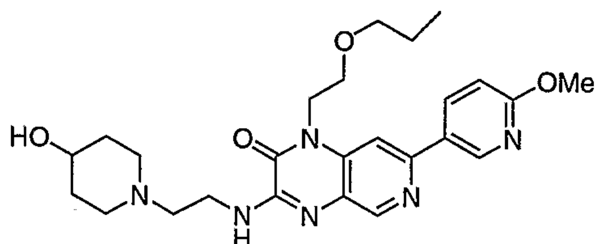
3-(2-(4-hydroxypiperidin-1-yl)ethylamino)-7-(6-methoxypyridin-3-yl)-1-(2-propoxyethyl)pyrido[3,4-b]pyrazin-2(1H)-one
