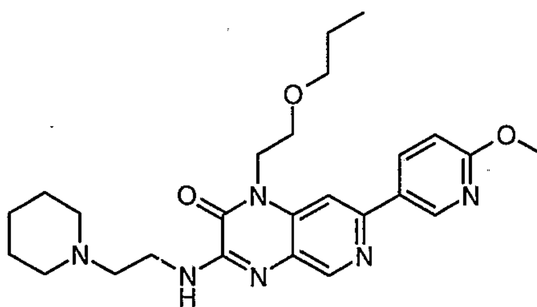
7-(6-methoxypyridin-3-yl)-3-[(2-piperidin-1-ylethyl)amino]-1-(2-propoxyethyl)pyrido[3,4-b]pyrazin-2(1H)-one.
