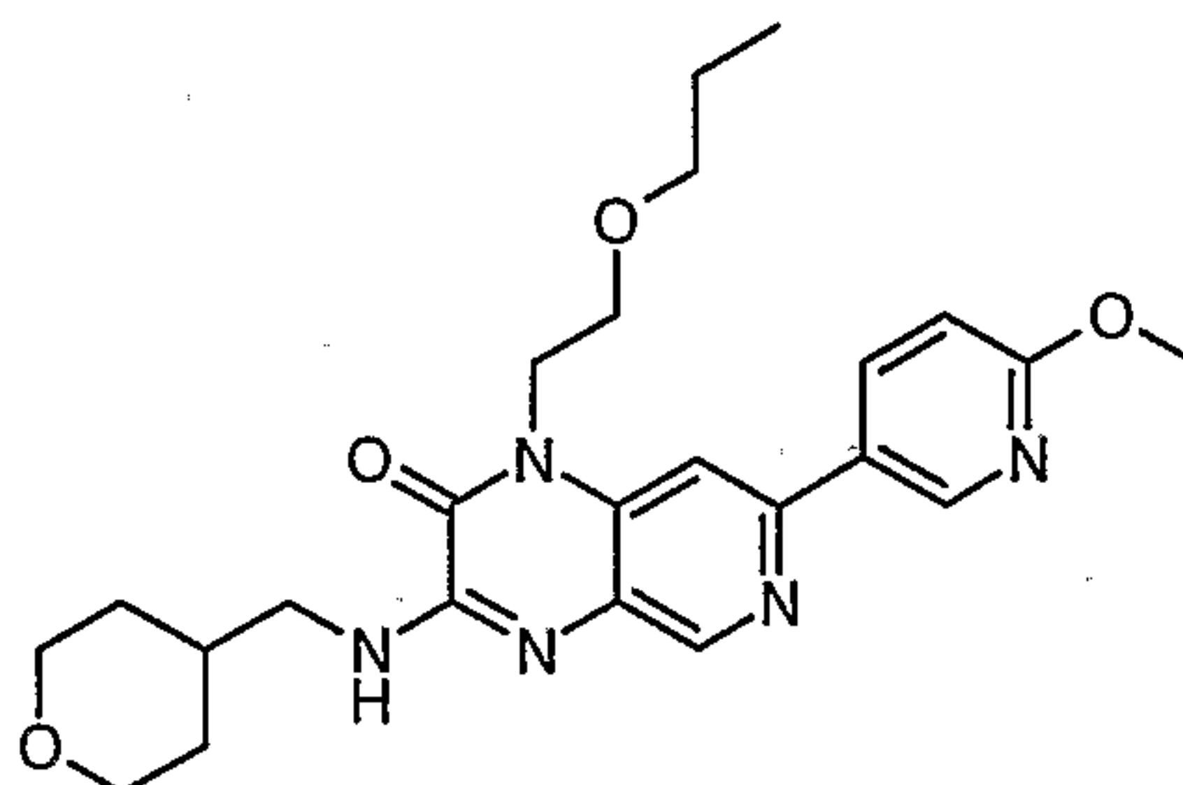
7-(6-methoxypyridin-3-yl)-1-(2-propoxyethyl)-3-[(tetrahydro-2H-pyran-4-ylmethyl)amino]pyrido[3,4-b]pyrazin-2(1H)-one.
