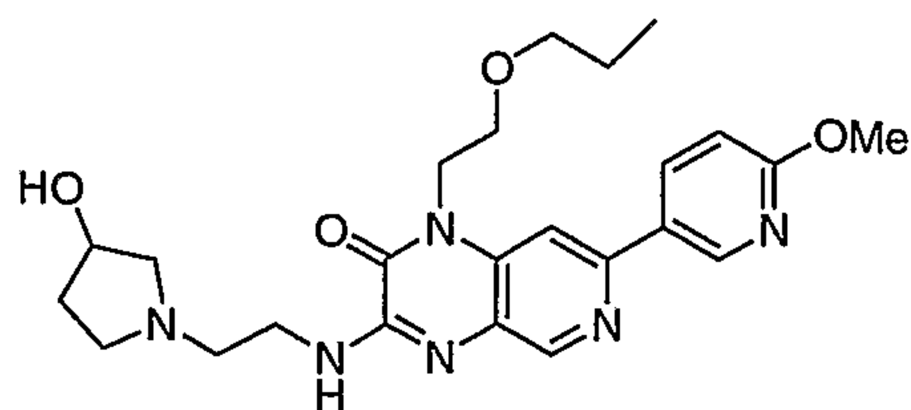
3-(2-(3-hydroxypyrrolidin-1-yl)ethylamino)-7-(6-methoxypyridin-3-yl)-1-(2-propoxyethyl)pyrido[3,4-b]pyrazin-2(1H)-one
