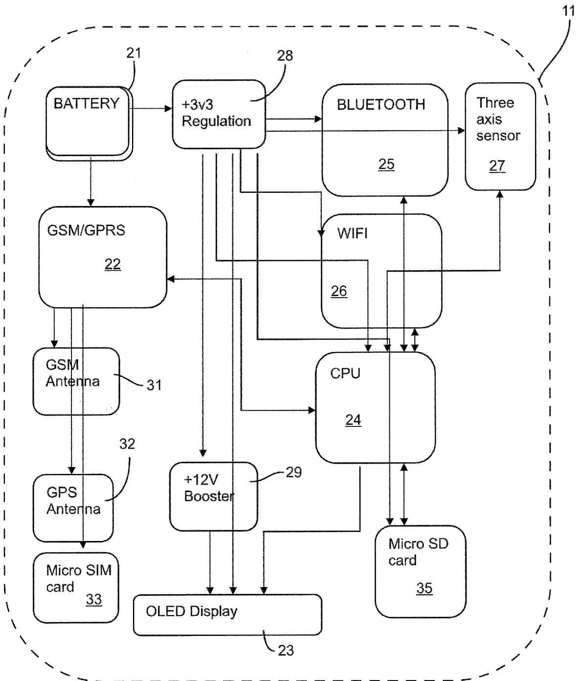
Picture 3.1. Shows internal block diagram of CCBM and interconnections between modules
