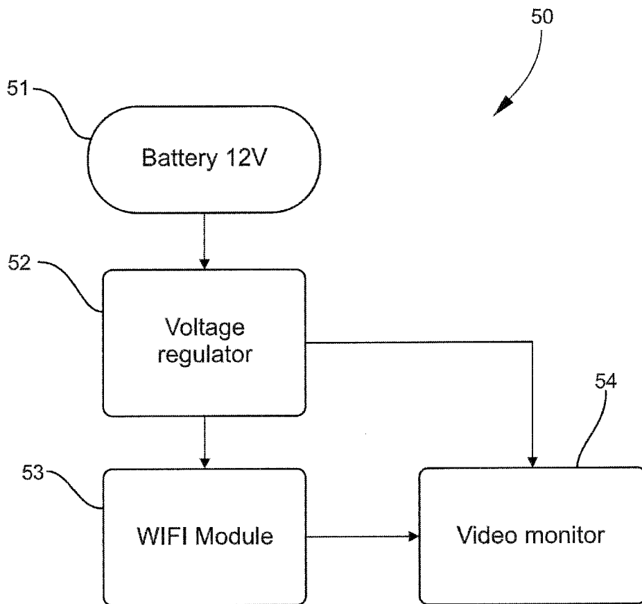
Picture 4 Video monitor model
