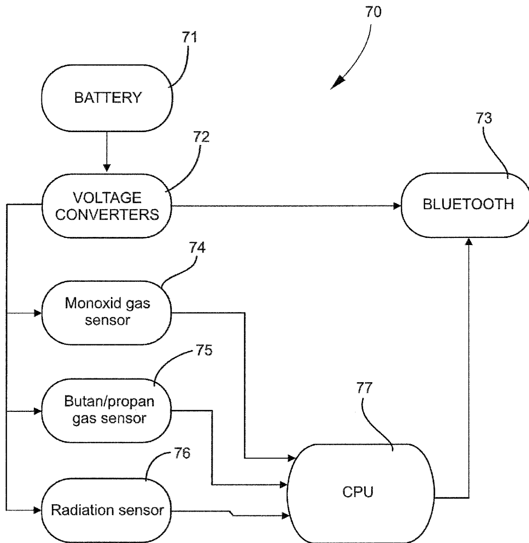
Picture 2 Hazardous sensor board
