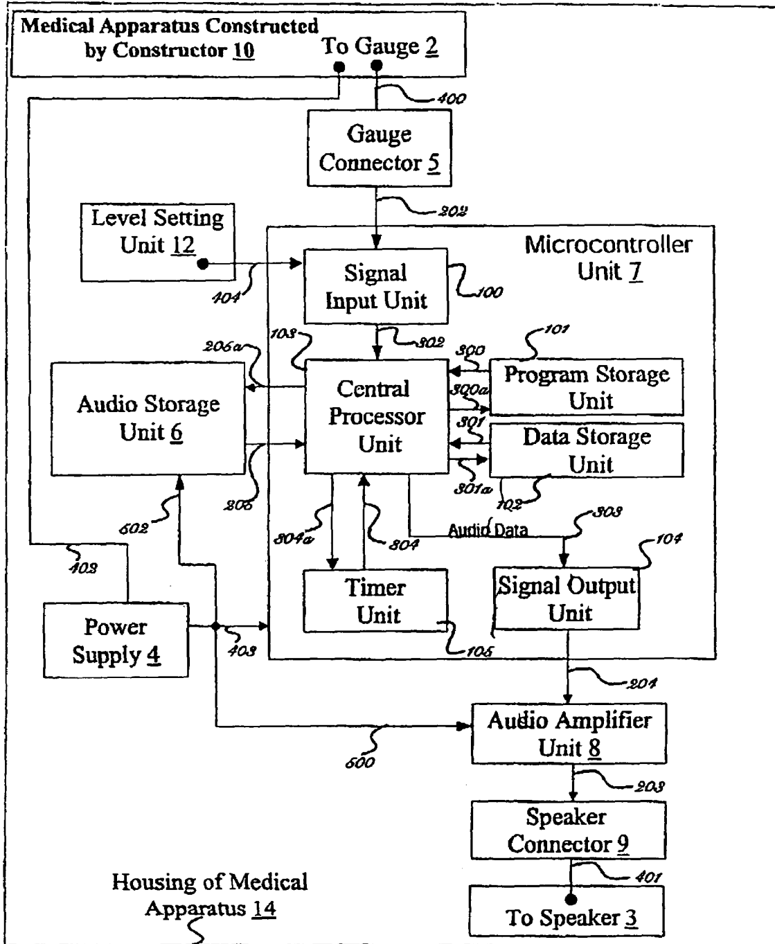
Fig. 2 Present Invention Within Housing of Medical Apparatus
