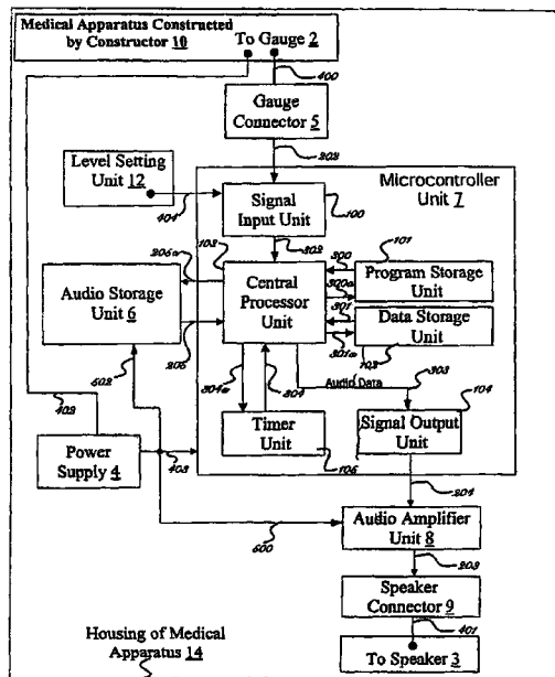
Present Invention Within Housing of Medical Apparatus
