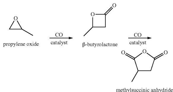
Scheme 6 Carbonylation of propylene oxide
