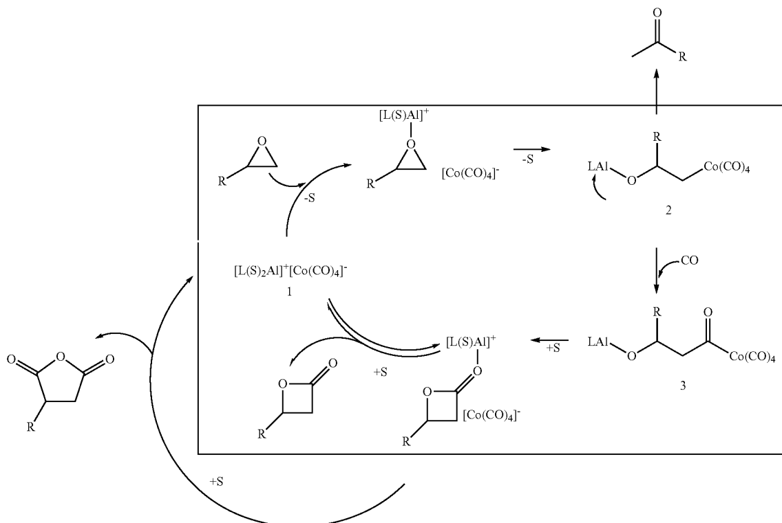
Scheme 8 Carbonylation of epoxides with [(\text{CITPP})\text{Al}]^+[\text{Co}(\text{CO})_4]^- .
