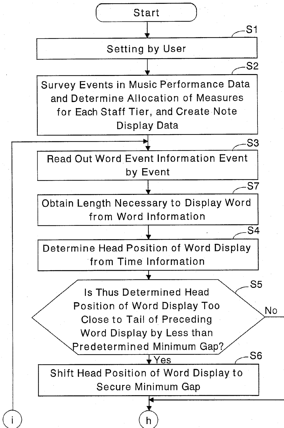
Fig. 4a Processing for Creating Word Display Data (Part 1)
