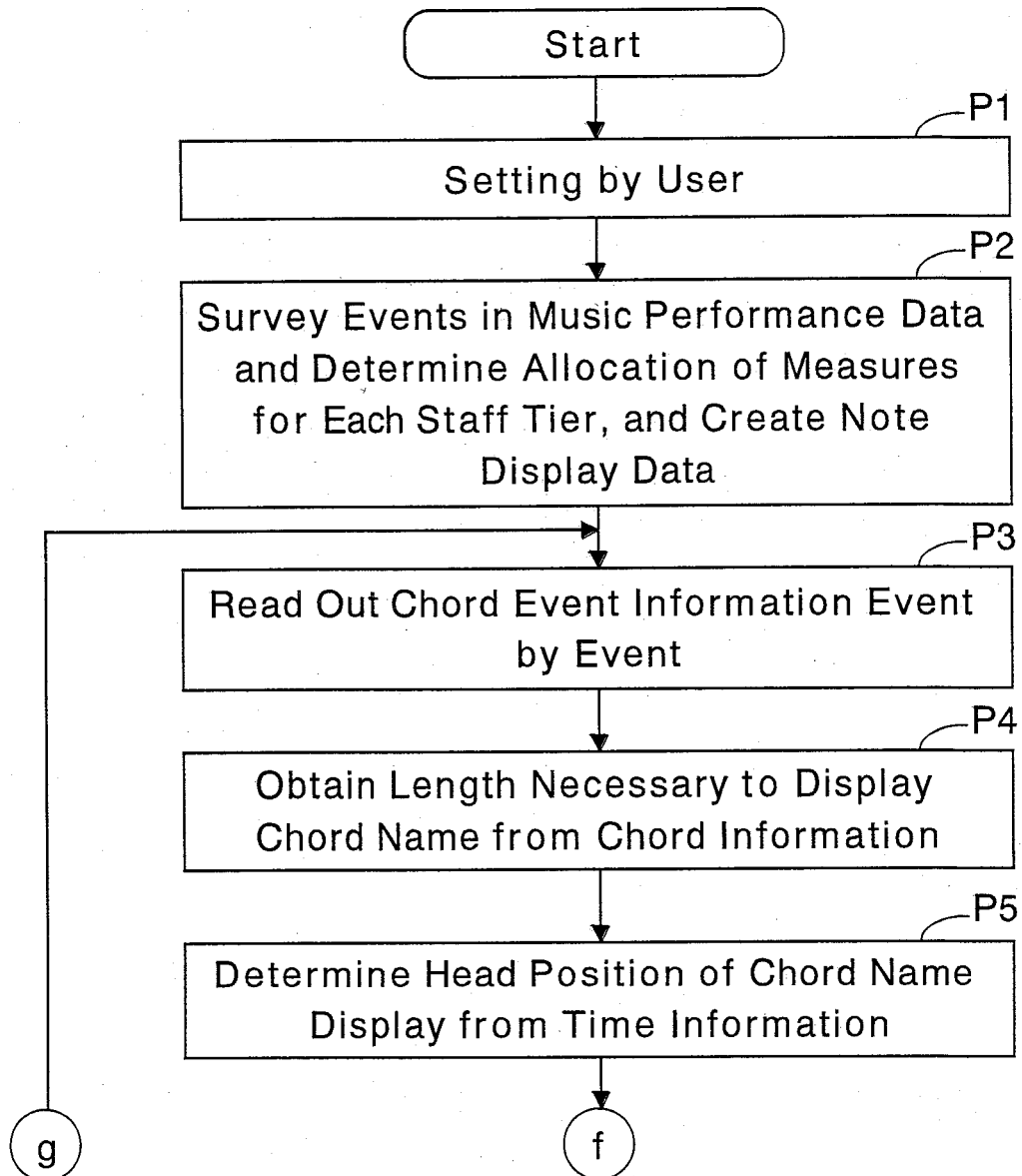
Fig. 3a Processing for Creating Chord Display Data (Part 1)
