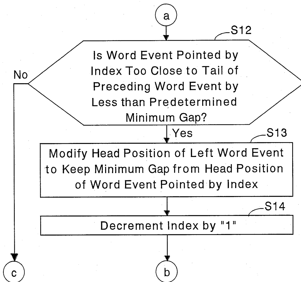
Fig. 4c Processing for Creating Word Display Data (Part 3)
