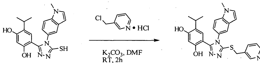
Compound 7
