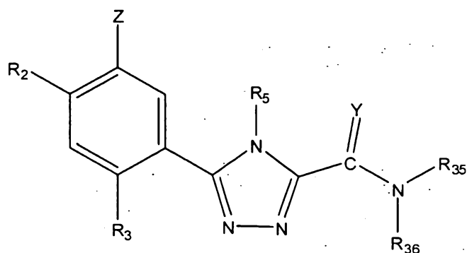
(X)
