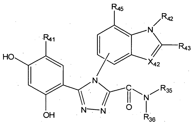
(XII)
