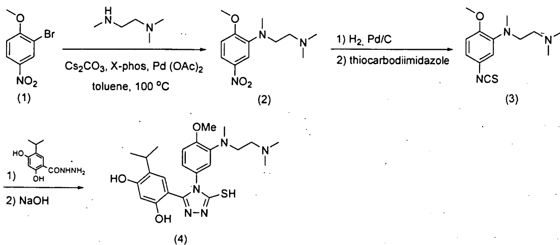
Scheme V
