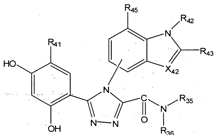
(XII)
