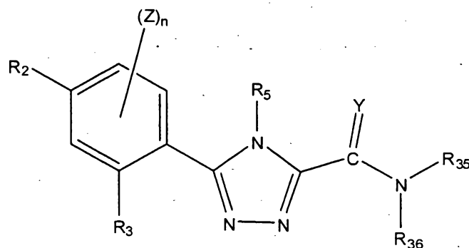
(IX)
