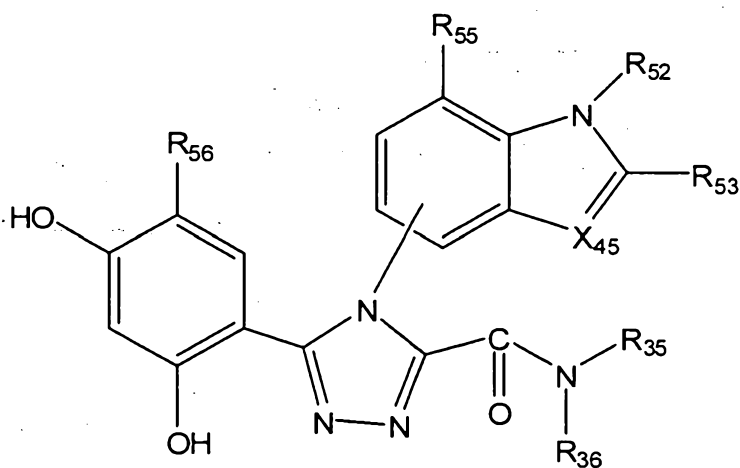
(XIII)
