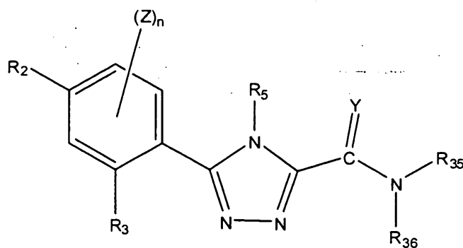
(IX)
