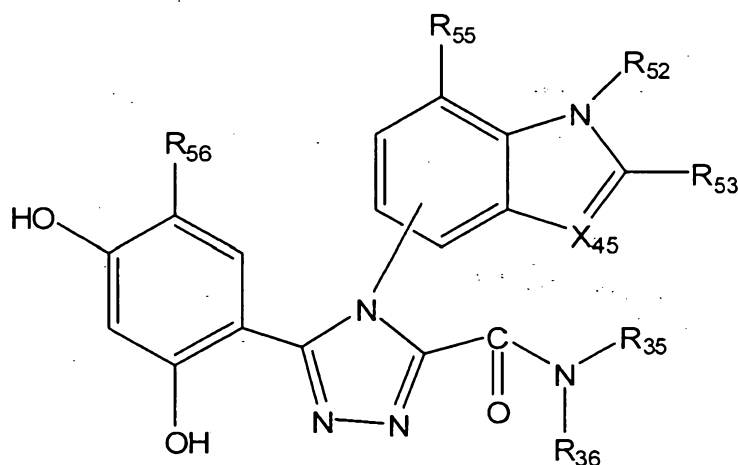
(XIII)
