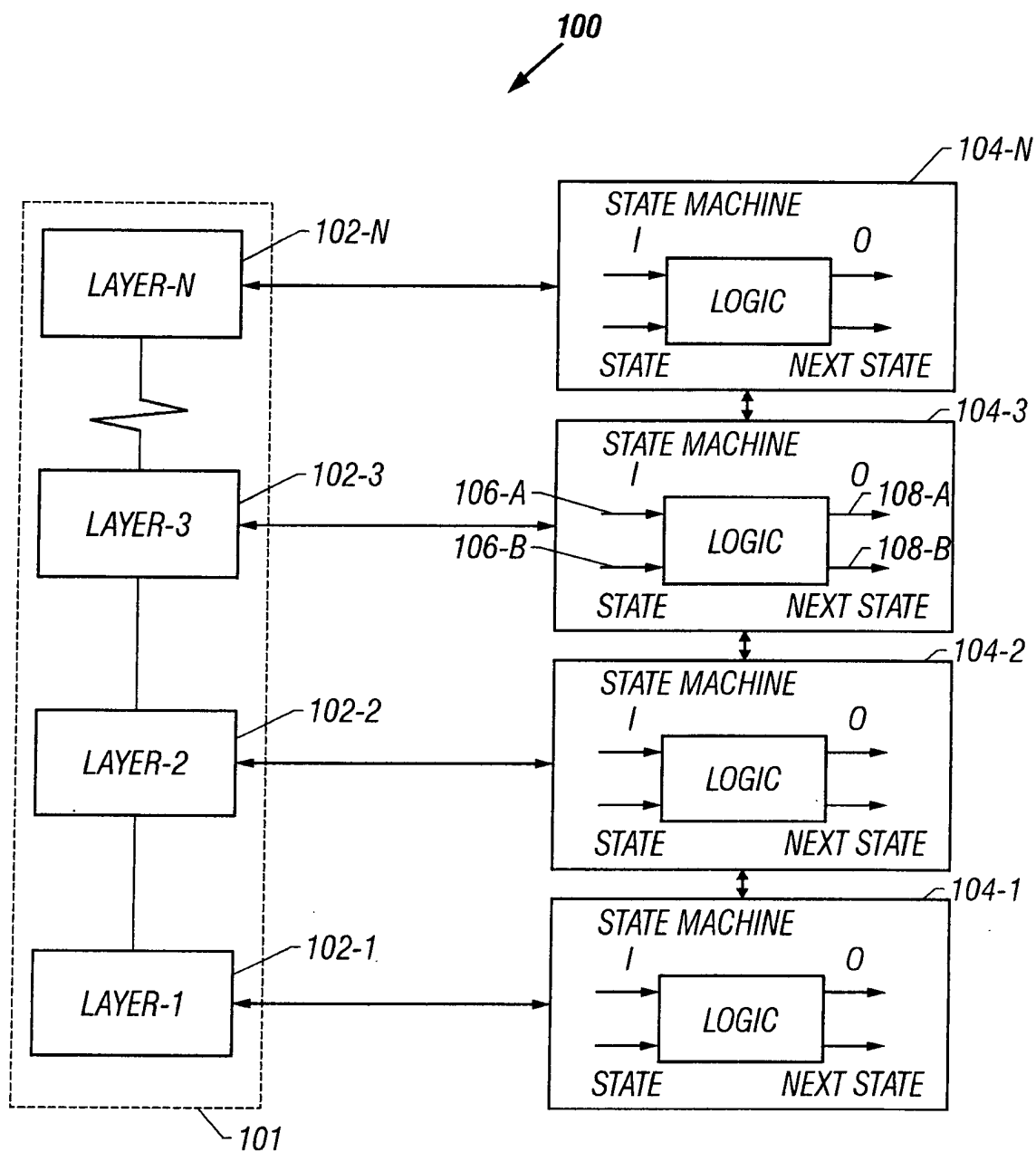
FIG. 1 (PRIOR ART)
