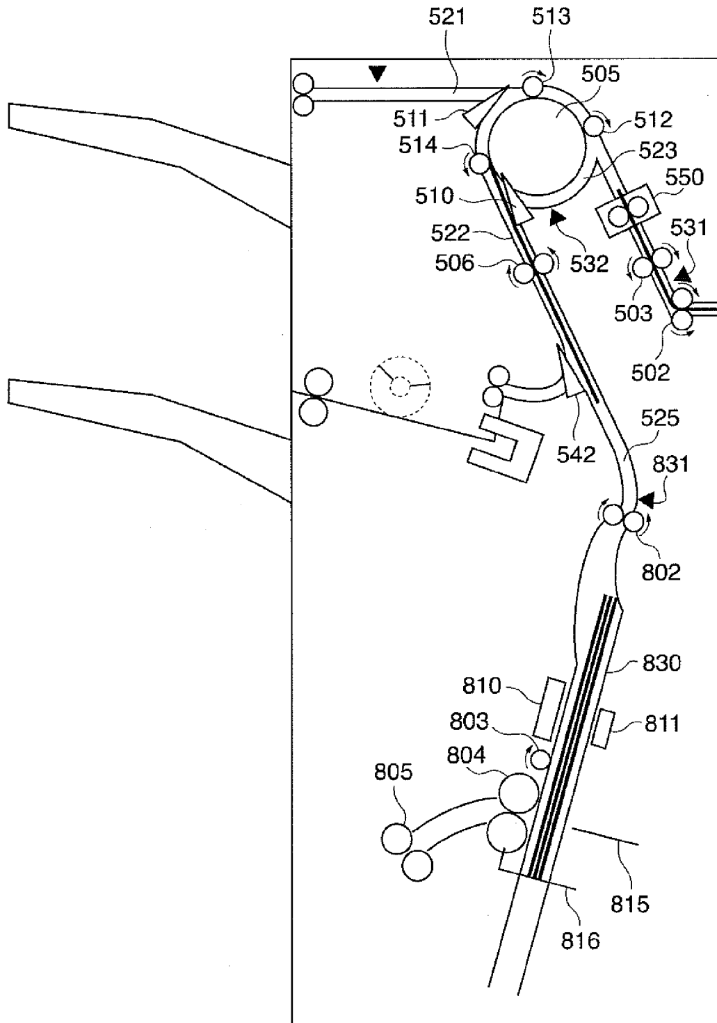
FIG. 28 BOOKBINDING MODE OPERATION
