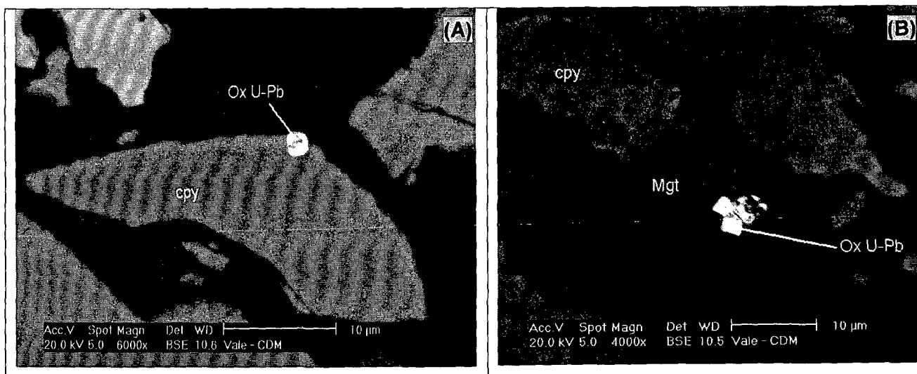
Figure 13 - Micrograph showing the features of uraninite associations in magnetic separation products - (A) non-magnetic product and (B) magnetic product
