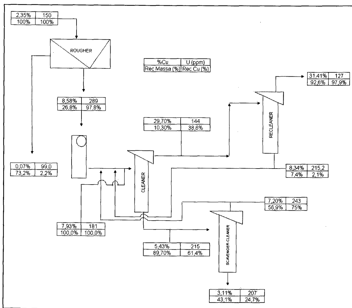
Figure 9 - Flotation flowchart of closed cleaner circuit from sample II
