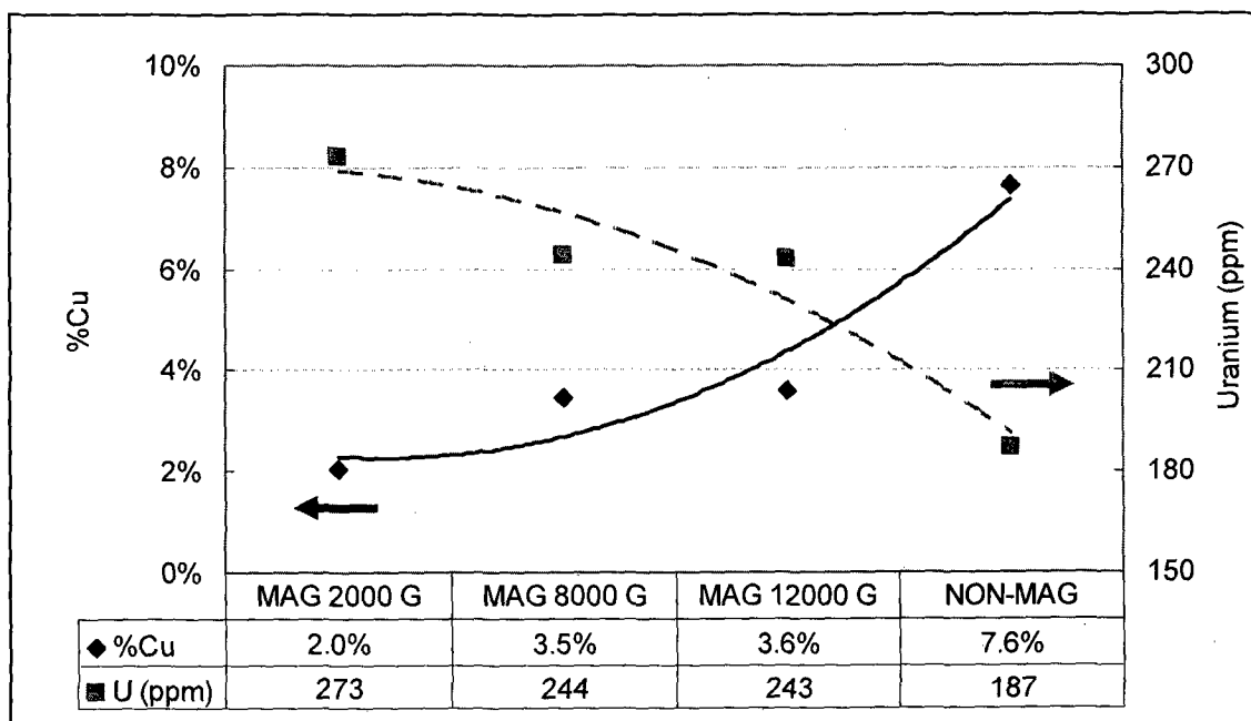
Figure 12 - Copper and uranium grade in the magnetic separation of scavenger-cleaner flotation concentrate (closed circuit cleaner)
