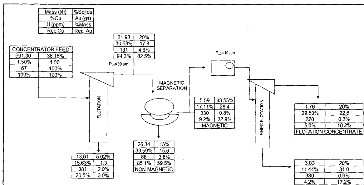
Figure 15 - Mass balance of concentrator with flotation from the magnetic separation
