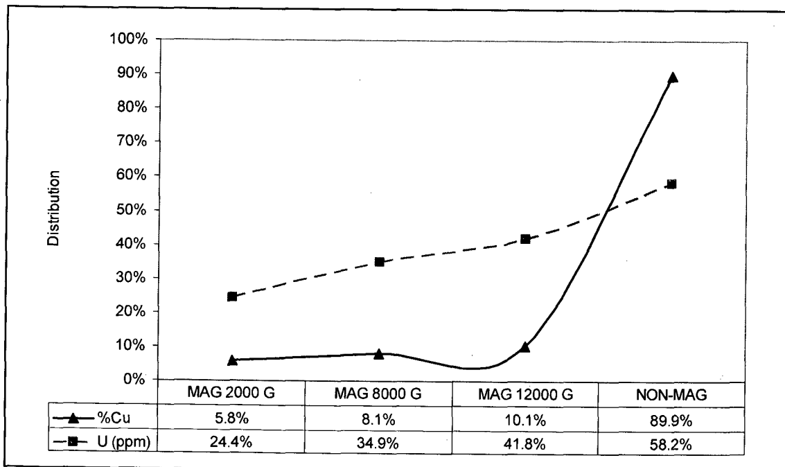
Figure 11 - Copper and uranium distribution in the magnetic separation of recleaner flotation concentrate (closed cleaner circuit - sample II)
