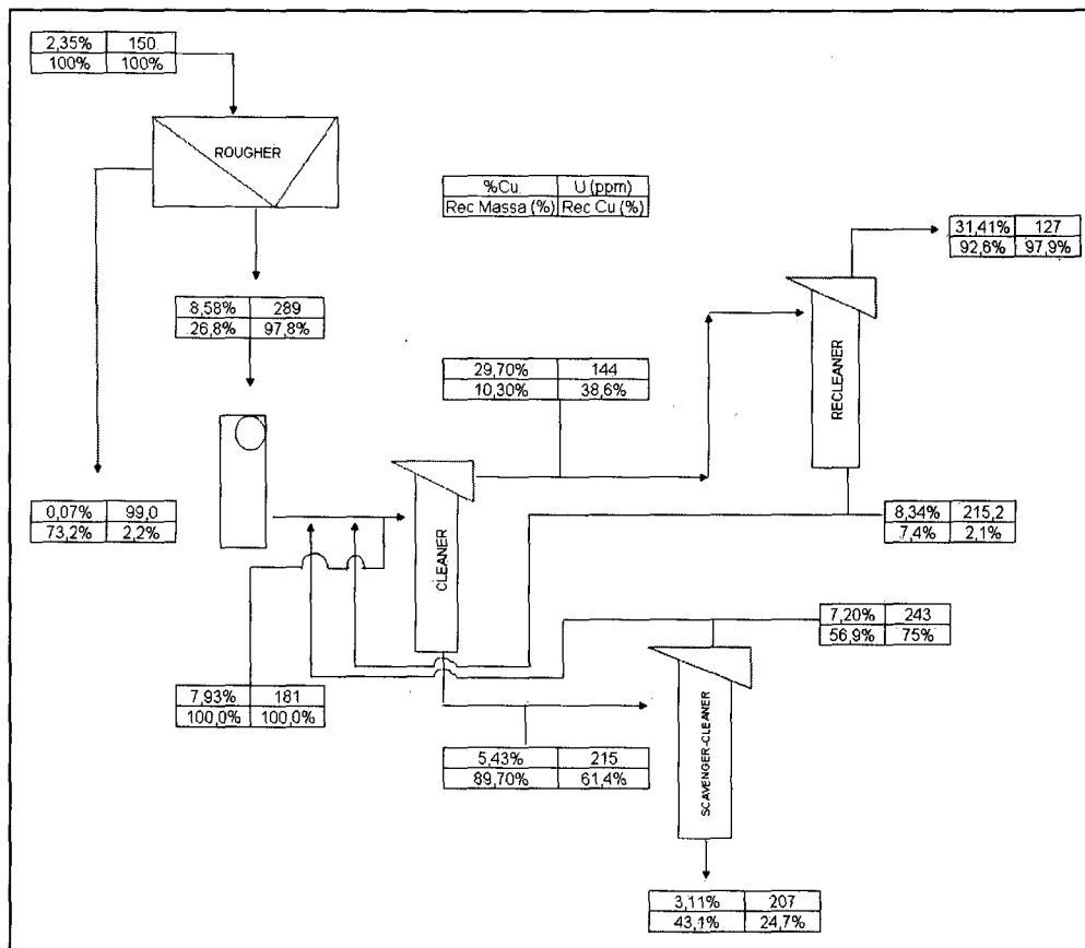
Figure 8 - Shows average values of grade and distribution for copper and uranium in the flotation runs.
