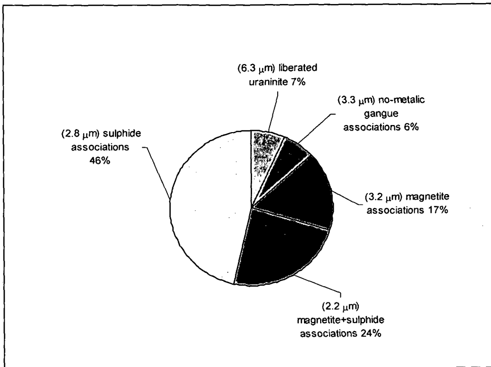
Figure 4 - Distribution of the U-Pb oxides in re-cleaner concentrate (run 2—closed circuit)
