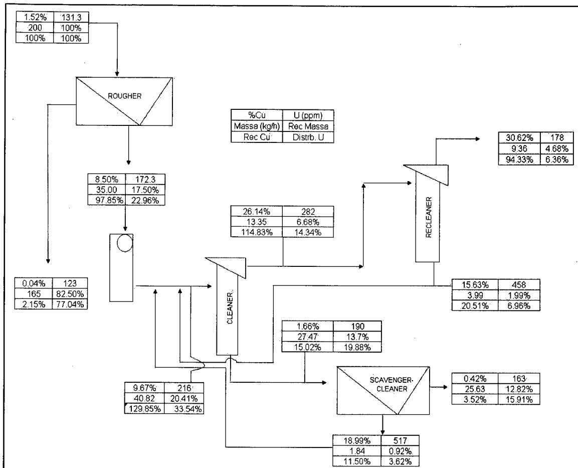
Figure 3 - Flotation flowchart of the run 2
