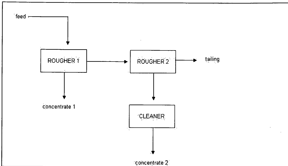
Figure 1 - Fine flotation of the cleaner flotation circulating load
