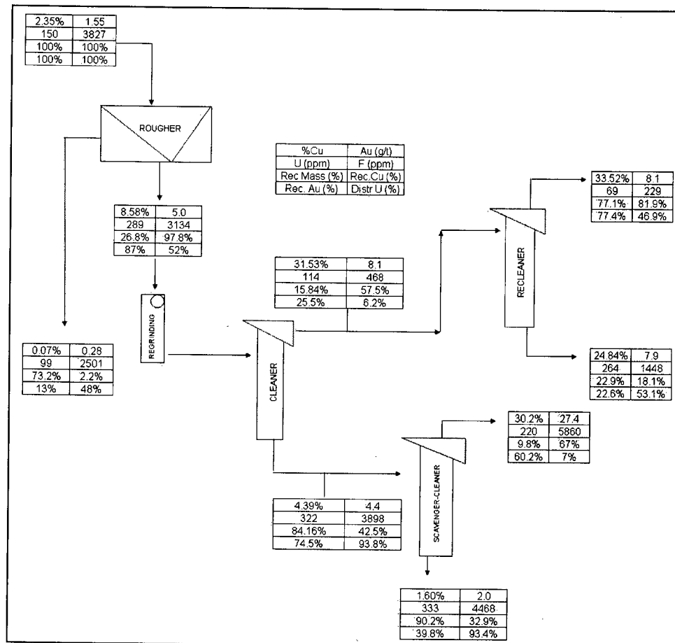
Figure 7 - Flotation flowchart of runs 1 and 2.
