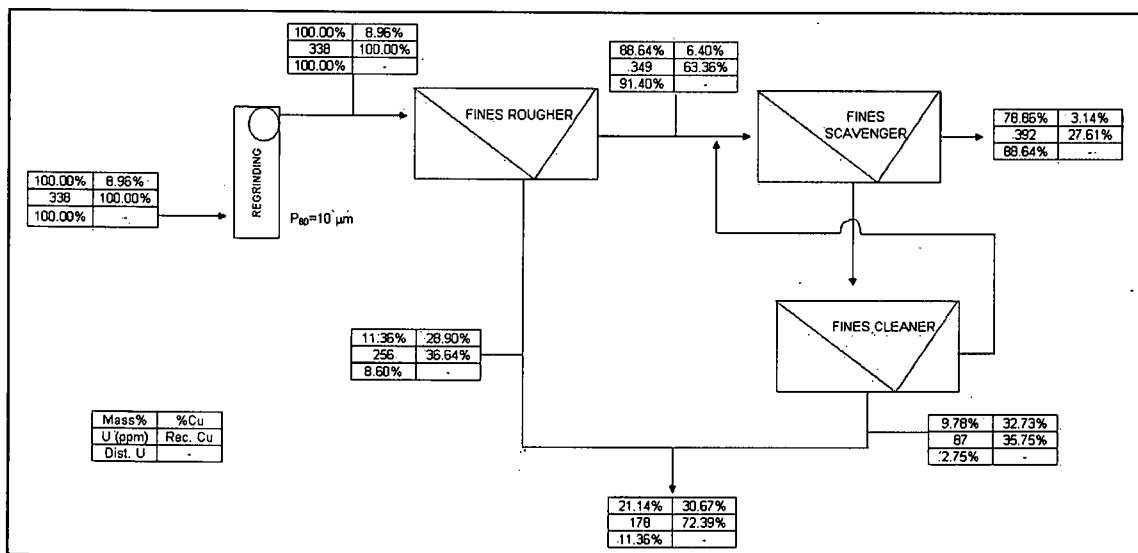
Figure 2 - Flowchart of the concentration of the circulating load from cleaner flotation
