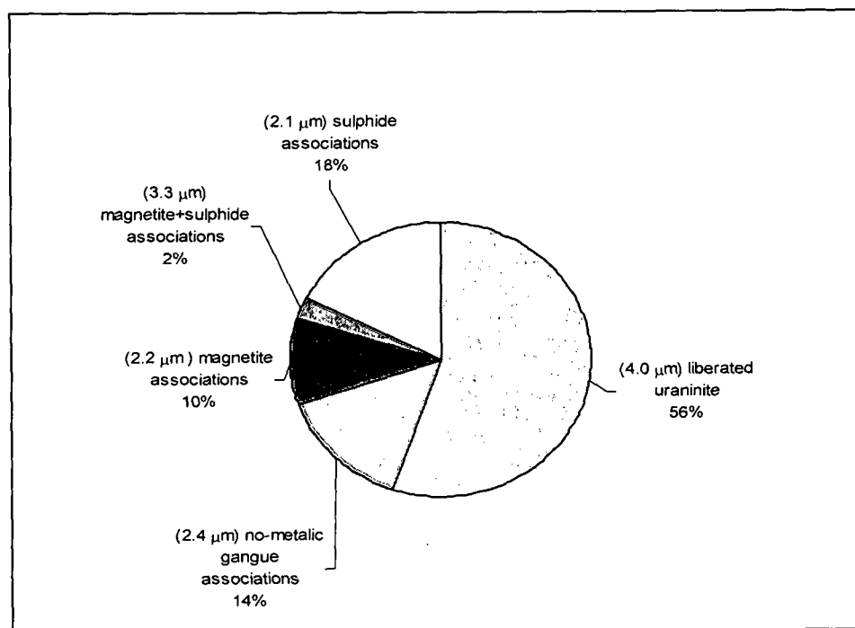
Figure 6 - Distribution of the U-Pb oxides in scavenger-cleaner concentrate (run 3—open circuit)
