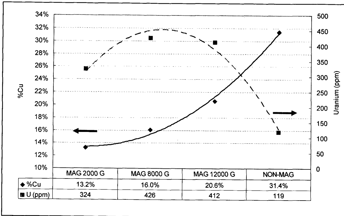
Figure10 - Copper and uranium grade in the magnetic separation of recleaner flotation concentrate (closed cleaner circuit - sample II)
