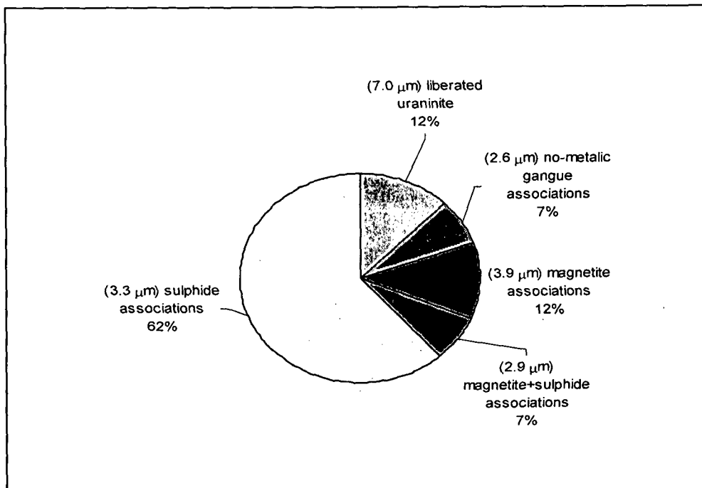
Figure 5 - Distribution of the U-Pb oxides in re-cleaner concentrate (run 3—open circuit)
