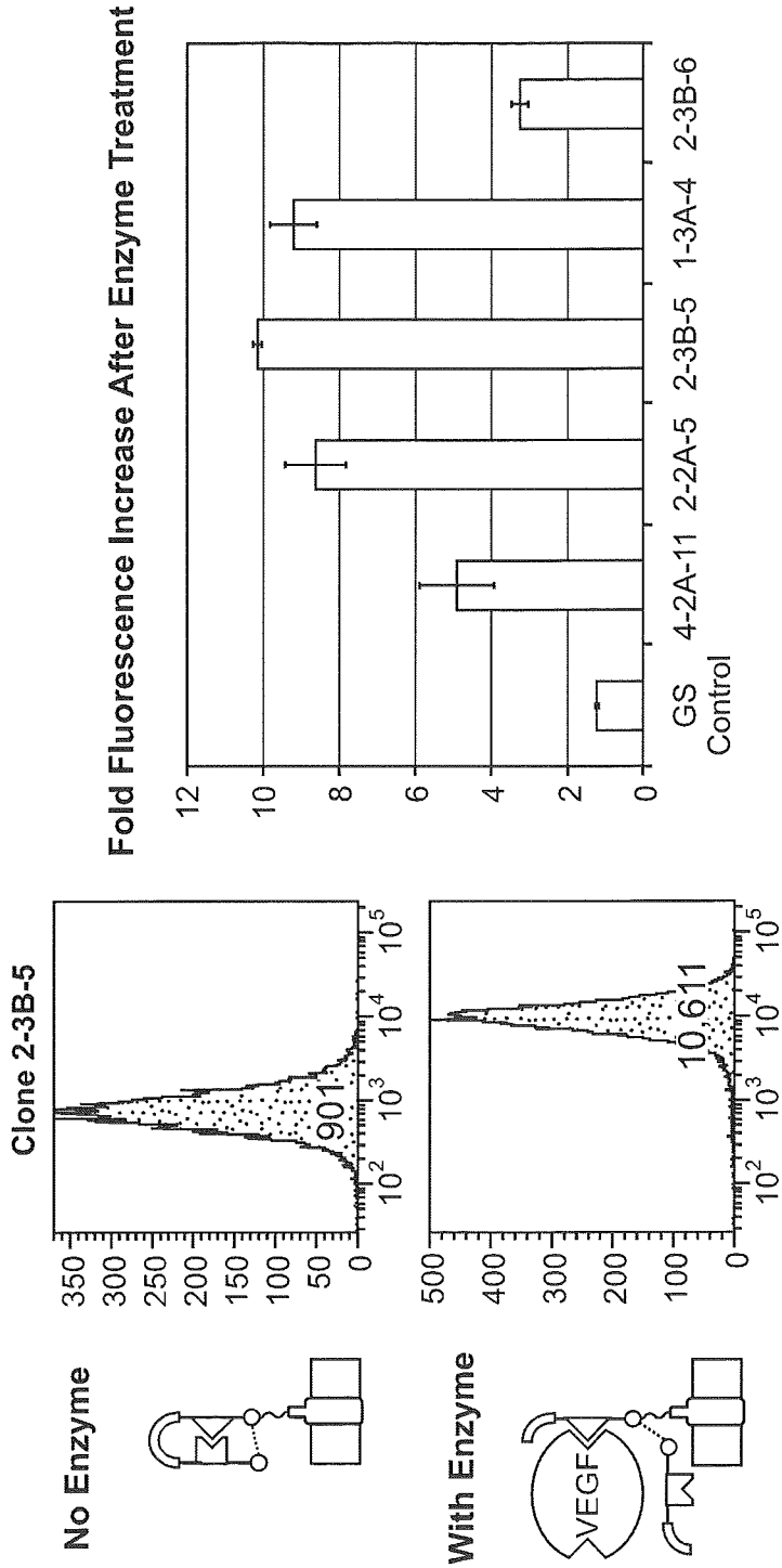
Switching activity for selected clones
