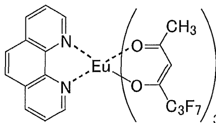
[Eu(FPD) 3 ]phen
