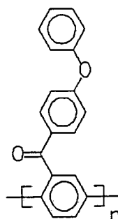
Poly-1,4-(4'-phenoxybenzoylphenylene), 2
