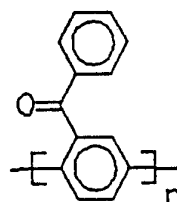
Poly-1,4-(benzoylphenylene), 1
