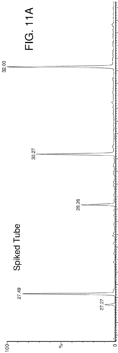
Sum of PAH chromatograms masses 142+153+166+178
