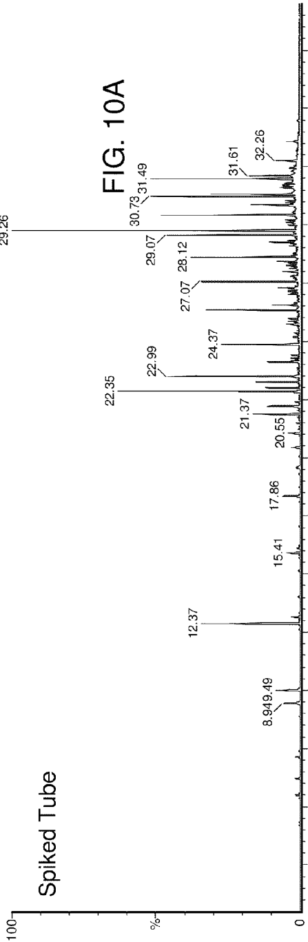
Mass ion 57 Chromatogram Representing diesel
