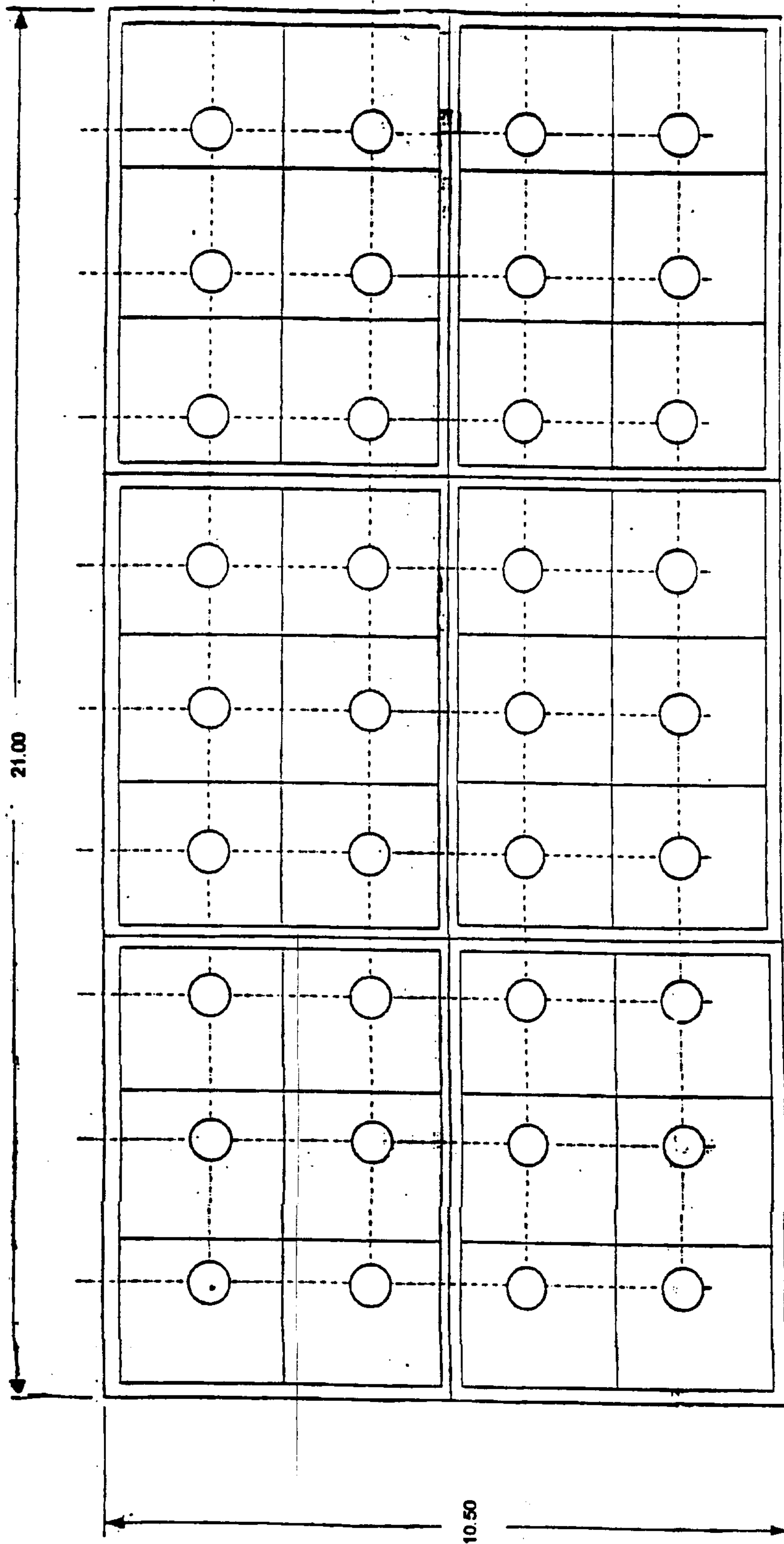
Example 9 432 / 6-06S (10.5x21) Plug Positions 9-1 4x3 pattern, no rows remain in plug tray Punch Plate p/n D303A0072
