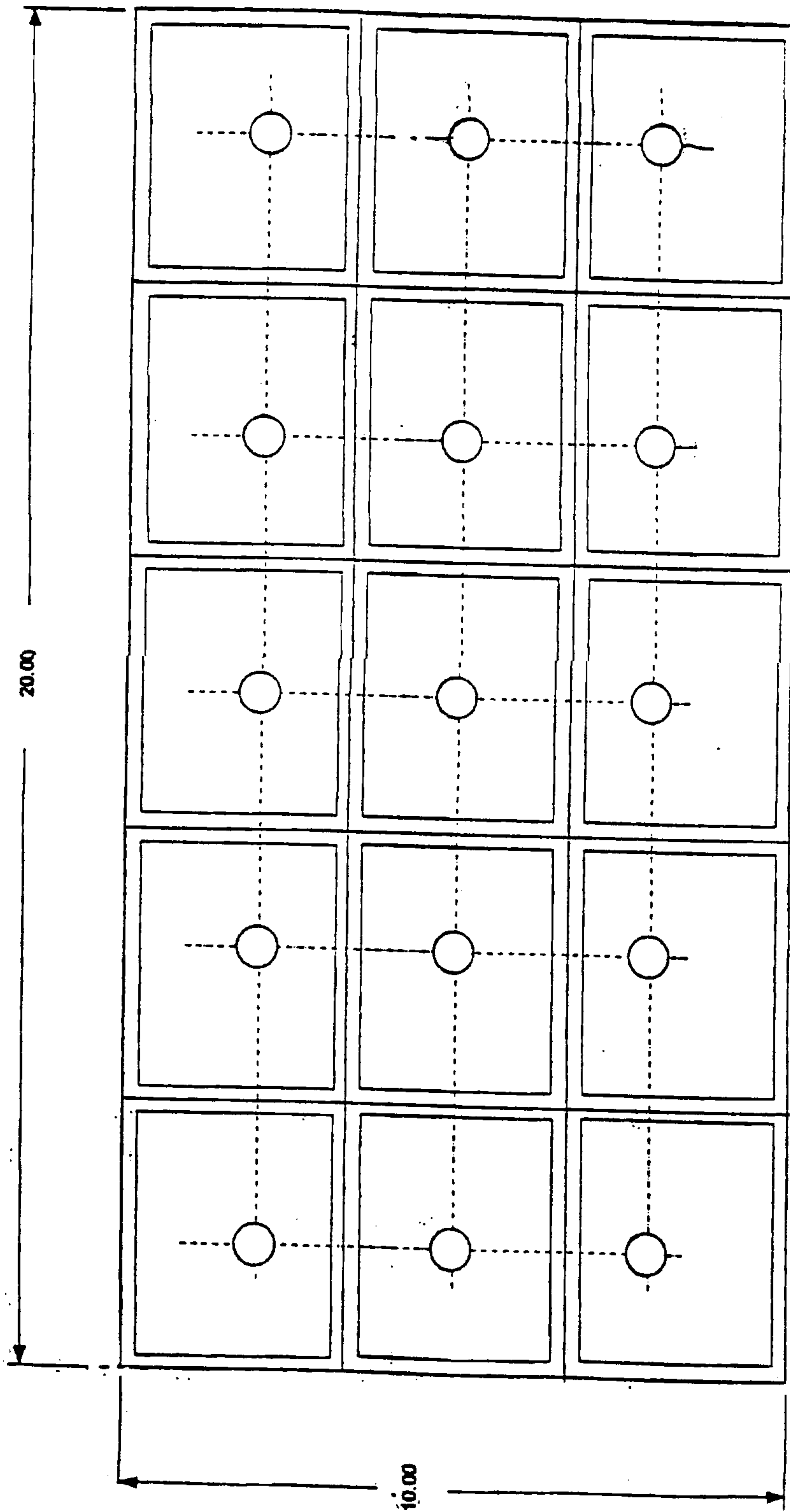
Example 7 324/15-01T (10x20) Plug Positions 8/1/01 7-18 Six pattern, 2 rows remain in plug tray Must have 5 notch plug tray handle Punch Plate pin D363A0042
