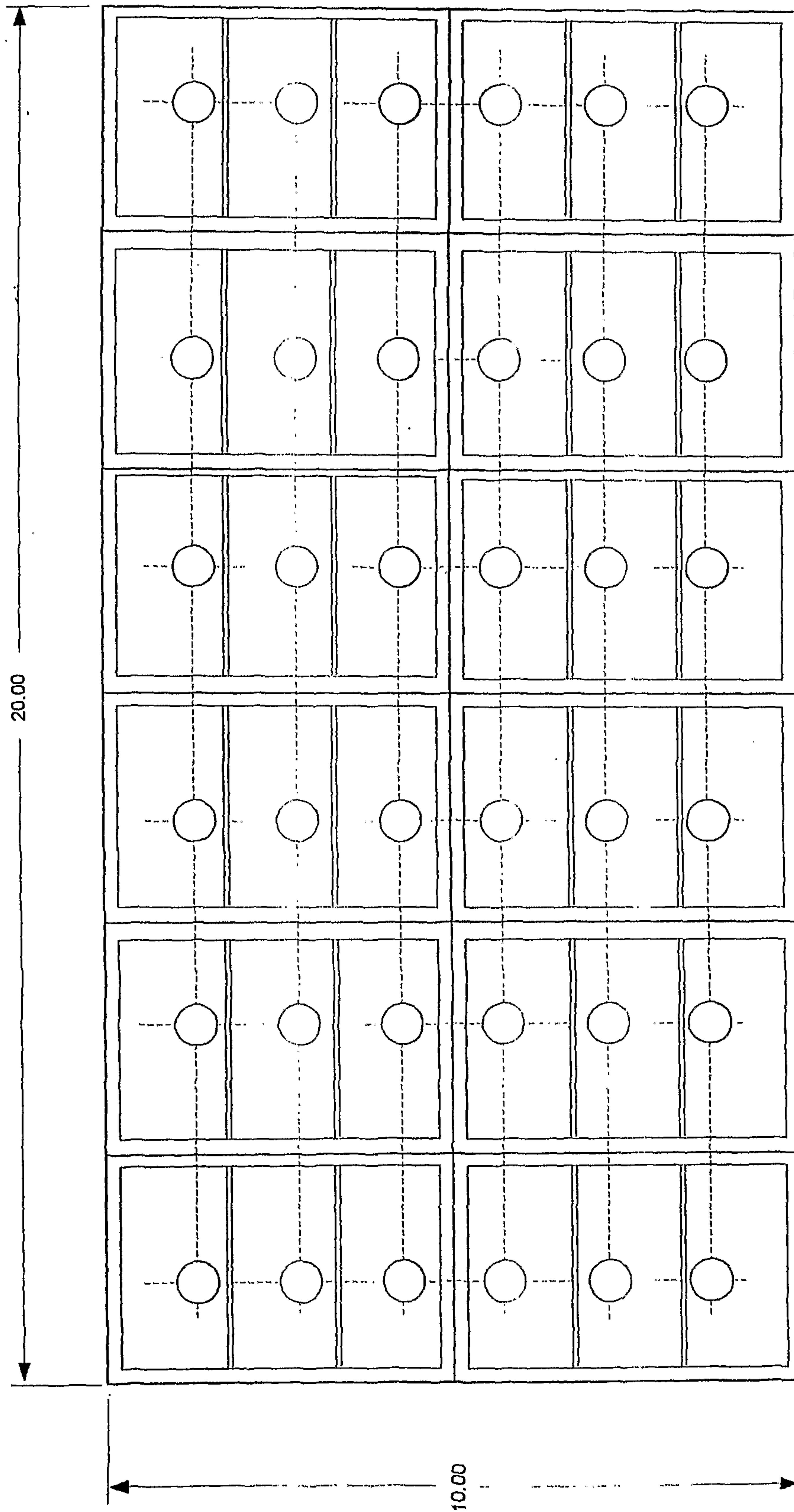
Example 7 324/12-03T (10x20) Plug Positions a/10: 4x2 pattern 3 rows remain in plug tray Punch Plate p/n D303A0032 7-12
