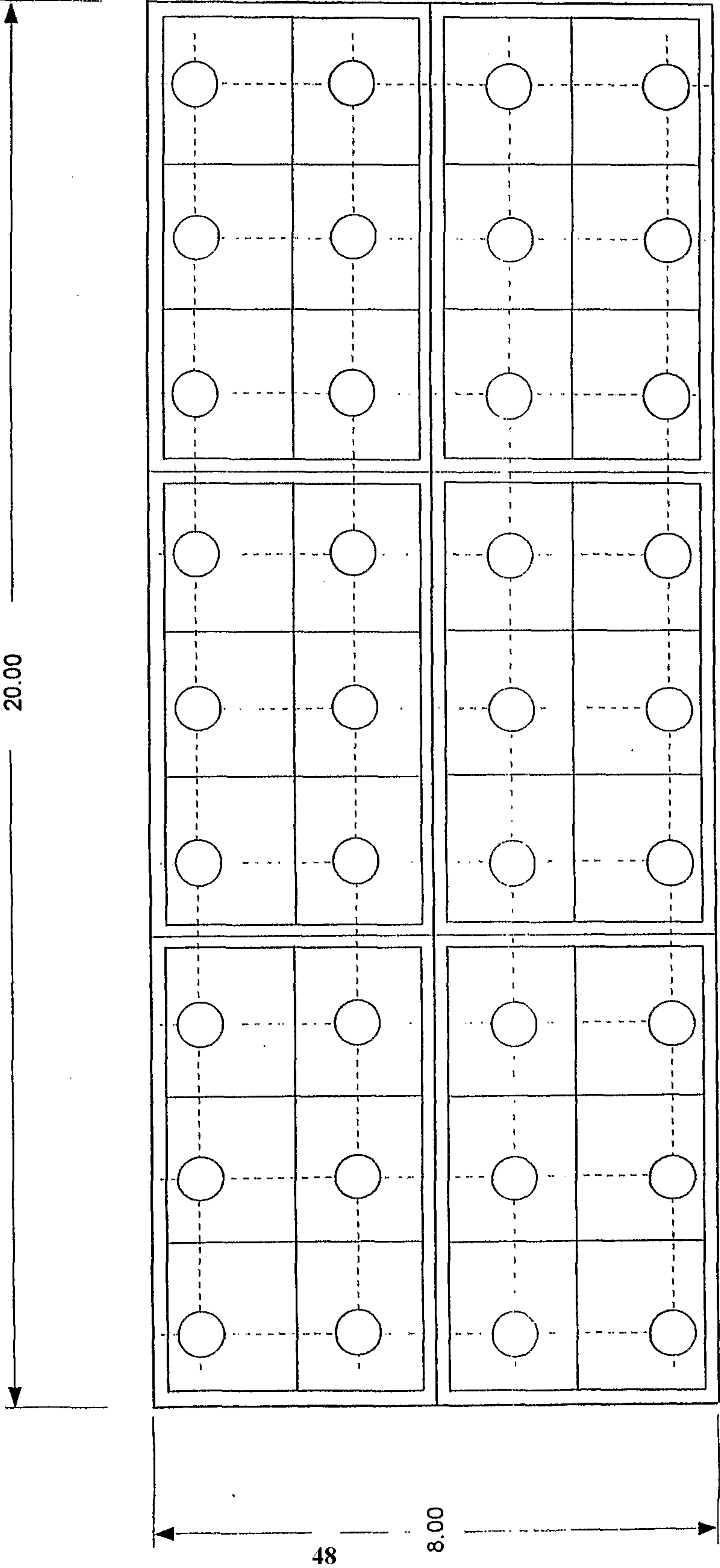
Example 7 7-2 324/6-06NS (8x20) Plug Positions 8/1/01 3x3 pattern, no rows remain in plug tray Punch Plate p/n D303A0036
