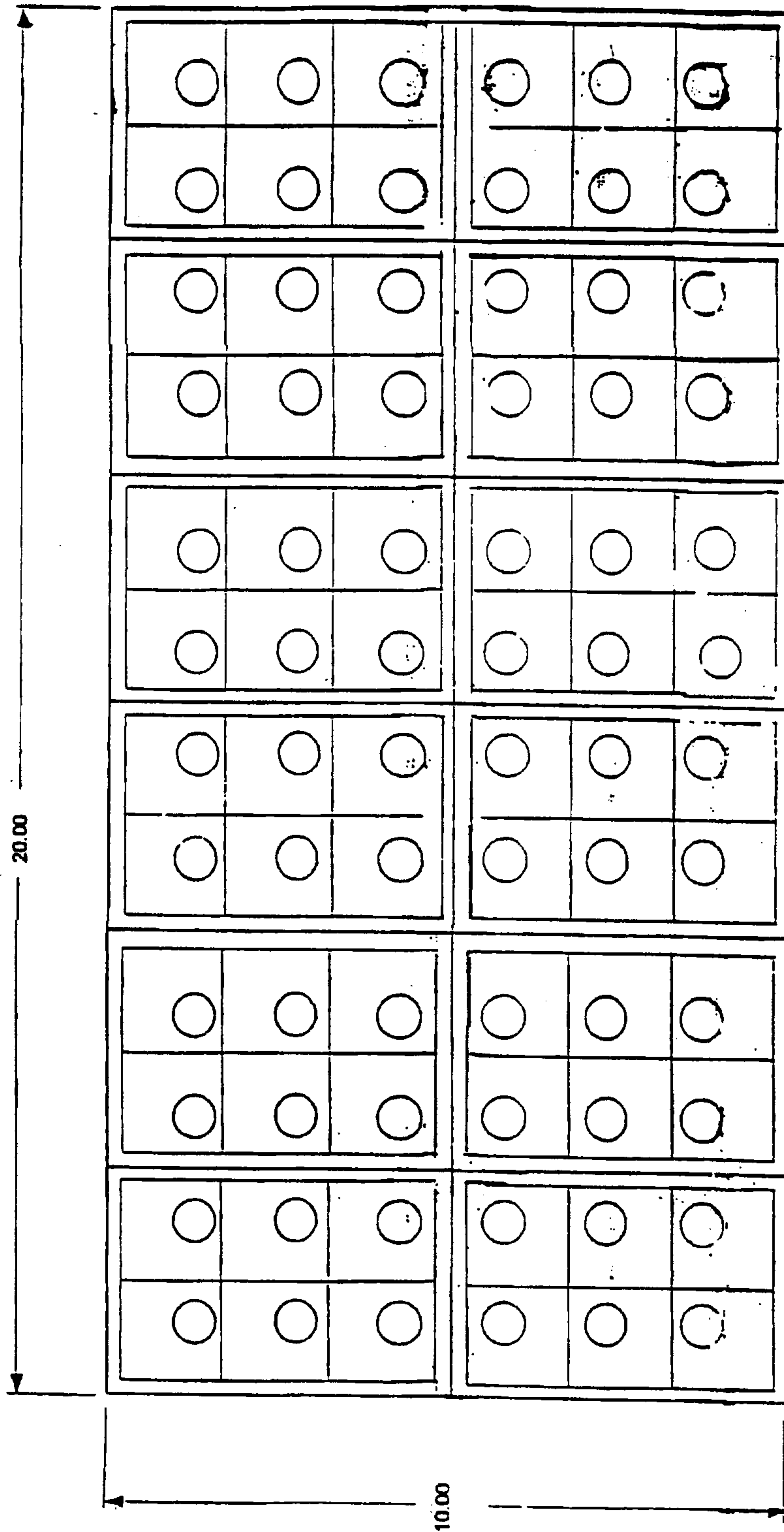
Example 7 324/12-06T (10x20) Plug Positions 8/1/01 7-17 2x2 pattern, 3 rows remain in plug tray Punch Plate pin D303A0038
