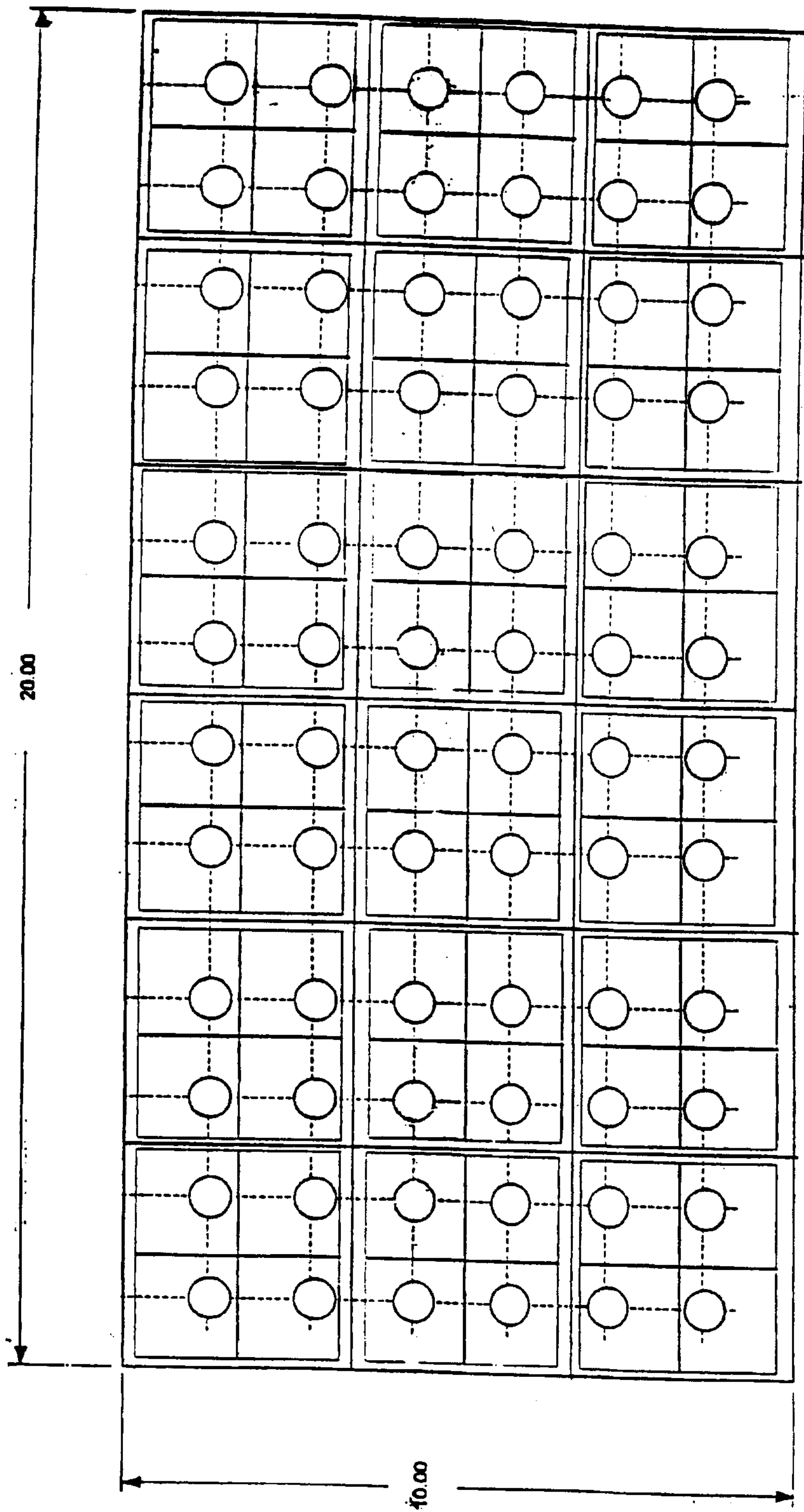
Example 7 324/18-04T (10x20) Plug Positions 31/01 7-24 2x2 pattern, 3 rows remain in plug tray Punch Plate p/n D303A0043
