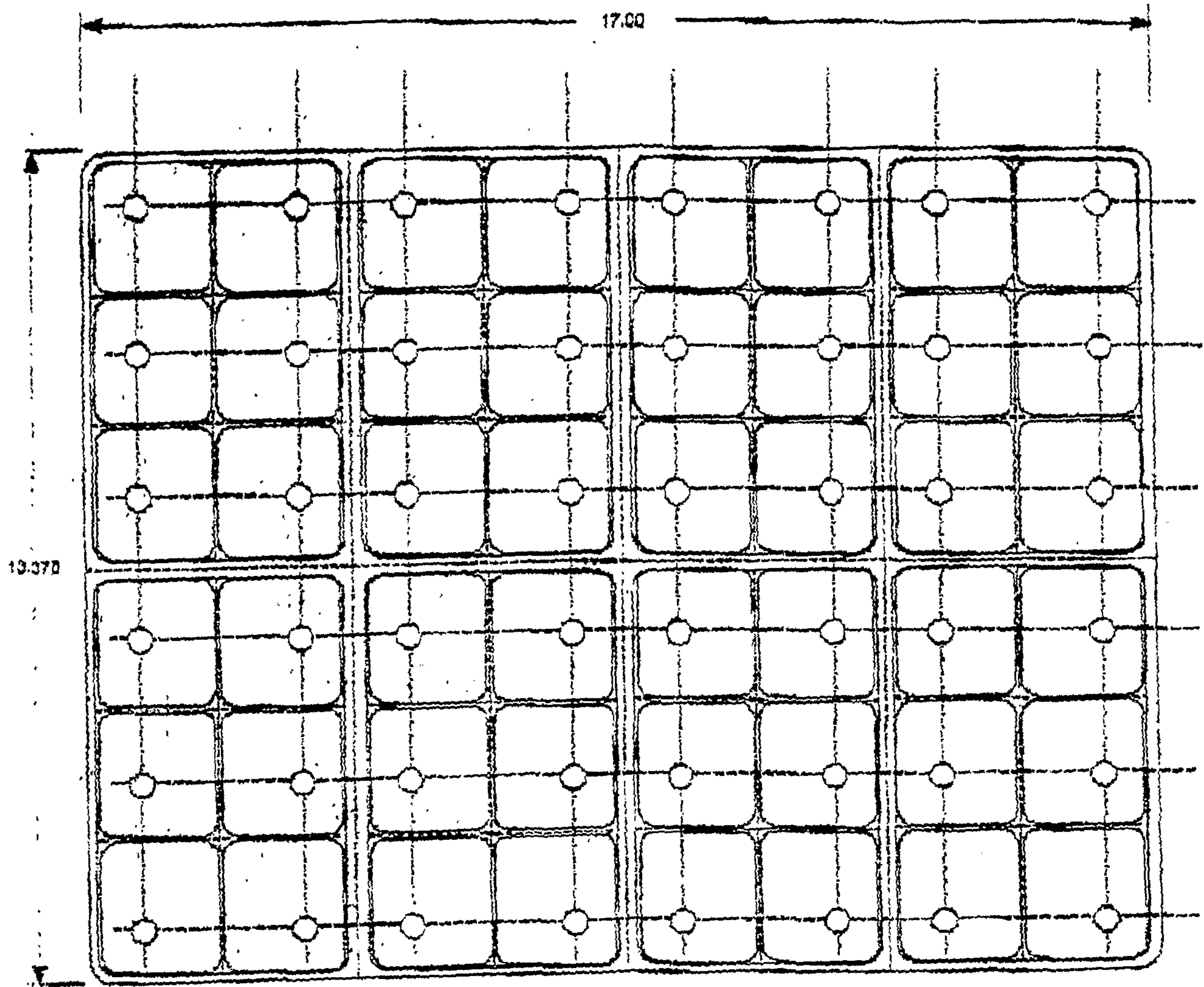
8-06 (14"x17") Plug Positions 2x3 pattern, 4 rows remain in plug way (3, 8, 13, 18) Scale: 1"=2.5'
