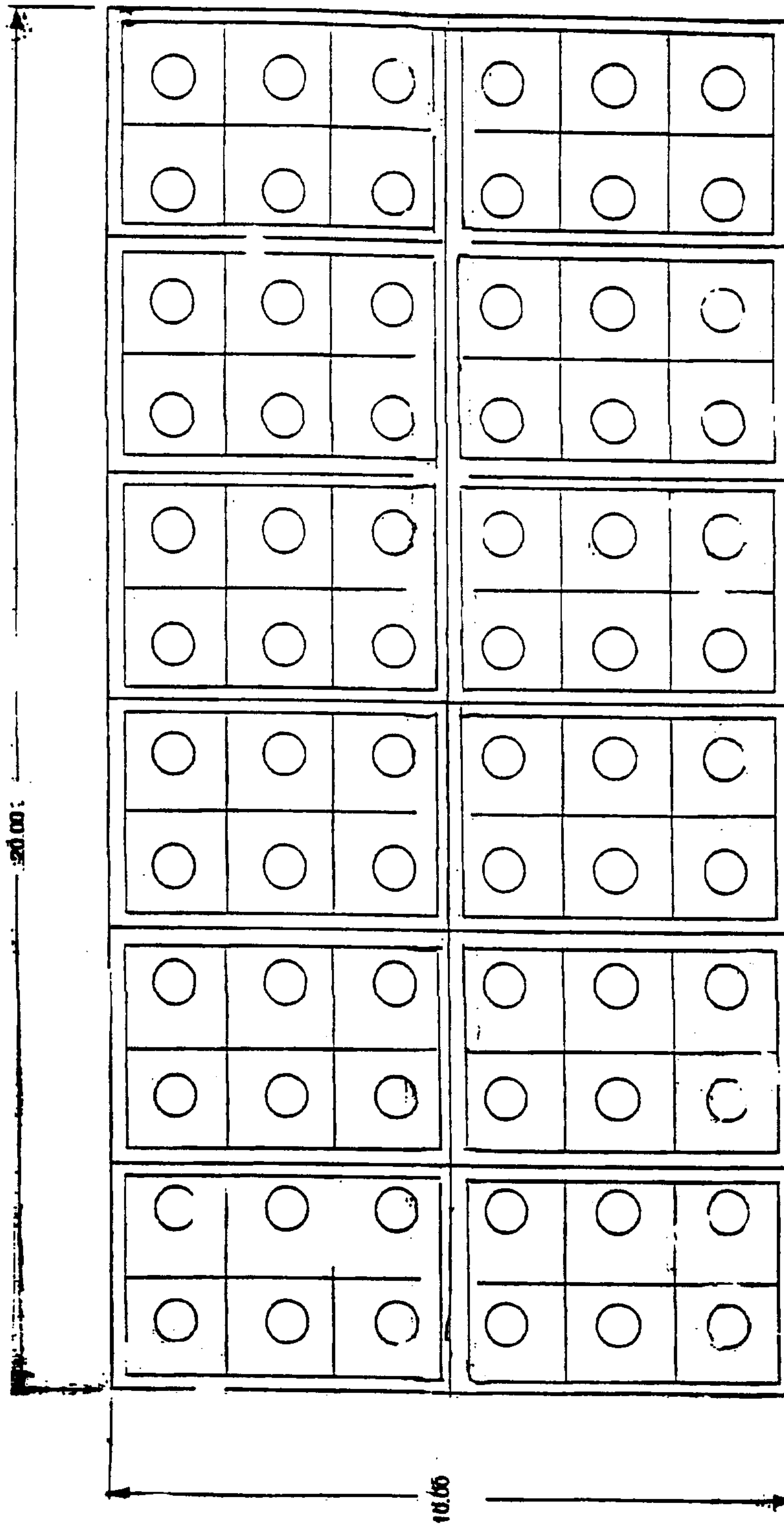
432 / 12-06T (10x20) Plug Positions 3x2 pattern, no rows remain in plug tray Punch Plate p/n D303A0074
