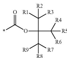
Boc Skeleton
