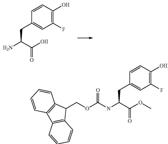
Compound 12
