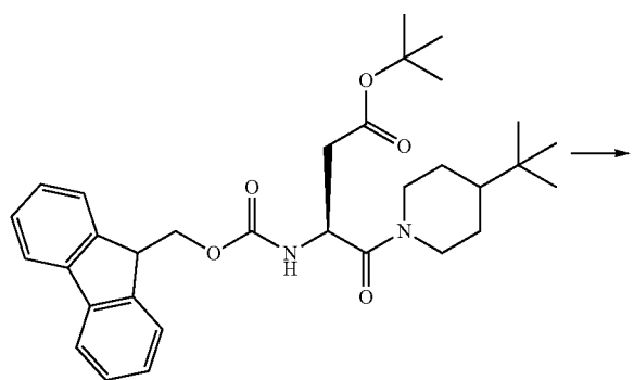
Compound 53
