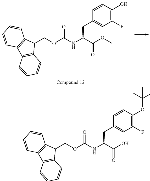
Compound 13
