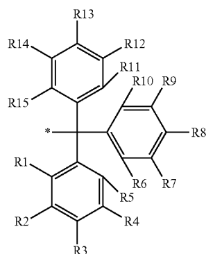
Trt Skeleton
