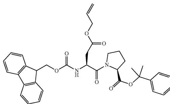
Compound 59
