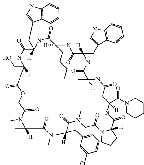
Compound 135
