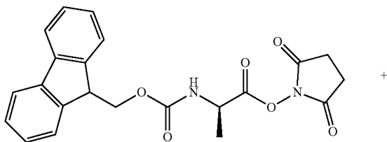
Compound 152
