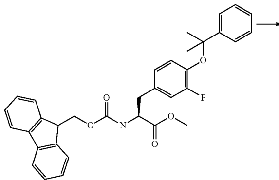
Compound 21
