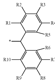
Dpm Skeleton
