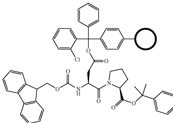
Compound 58
