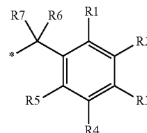
Bn Skeleton
