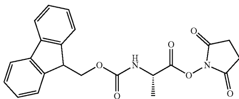
Compound 152
