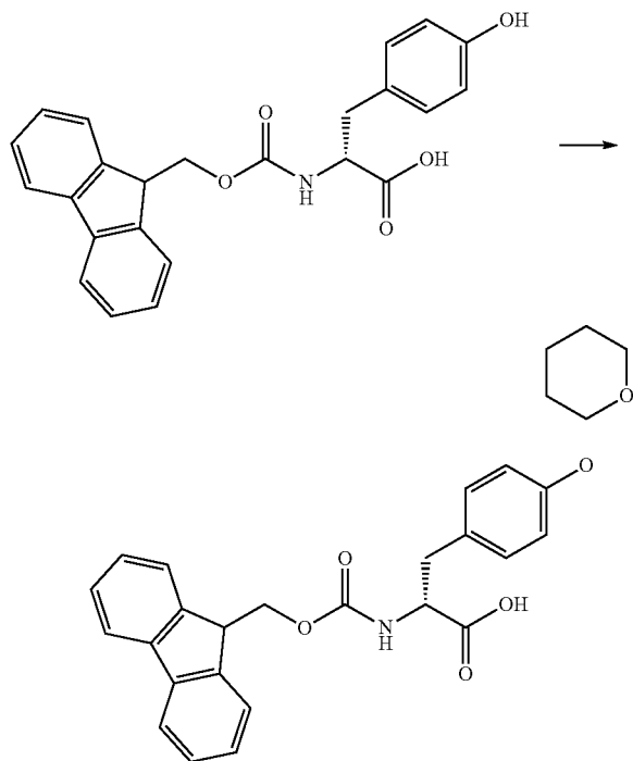
Compound 8
