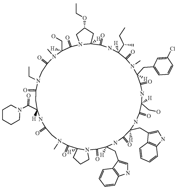
Compound 133
