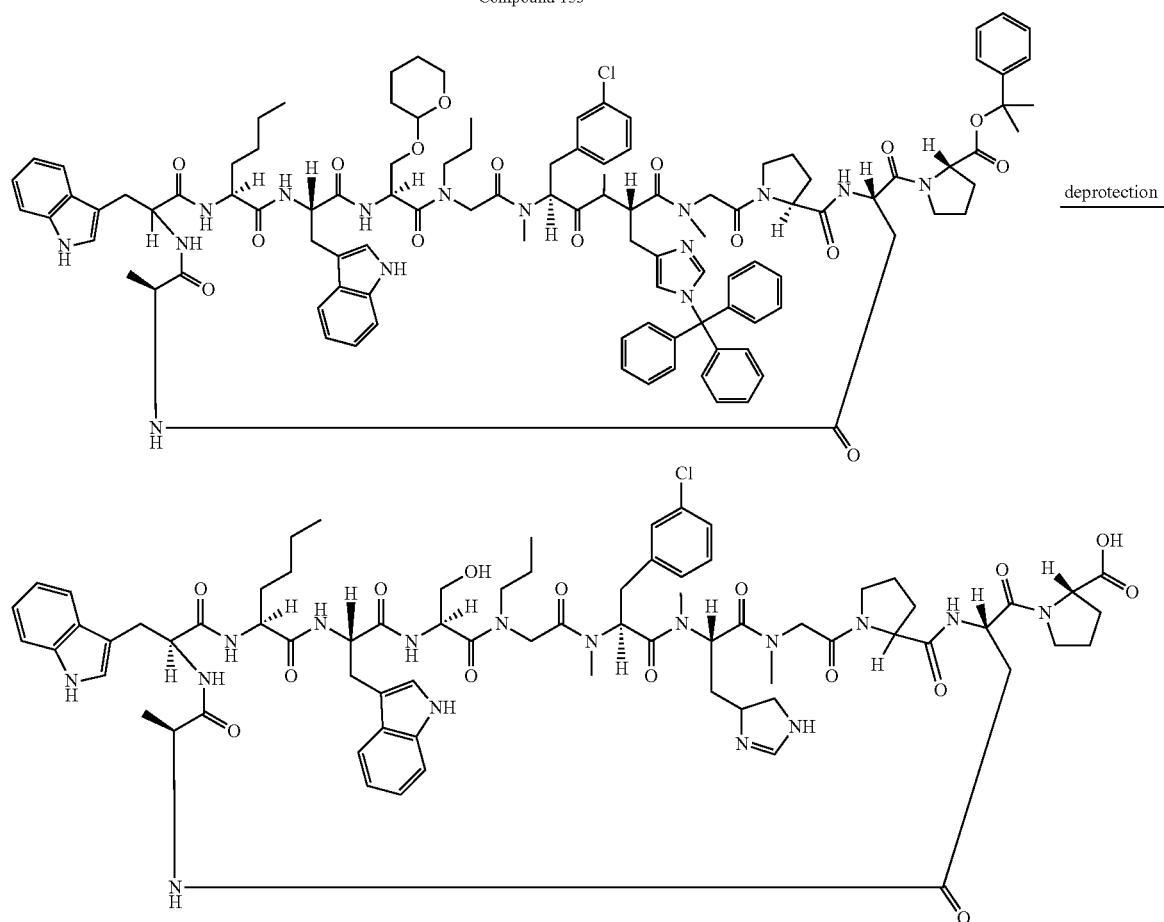
Compound 154
