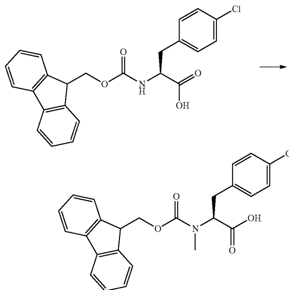
Compound 16
