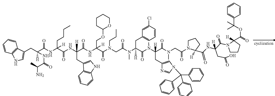
Compound 153
