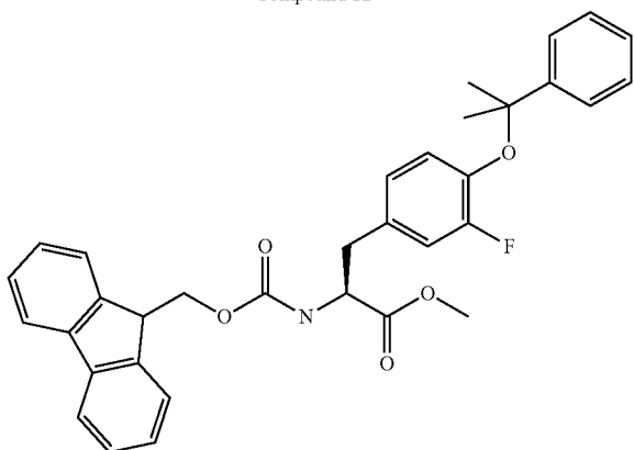
Compound 21
