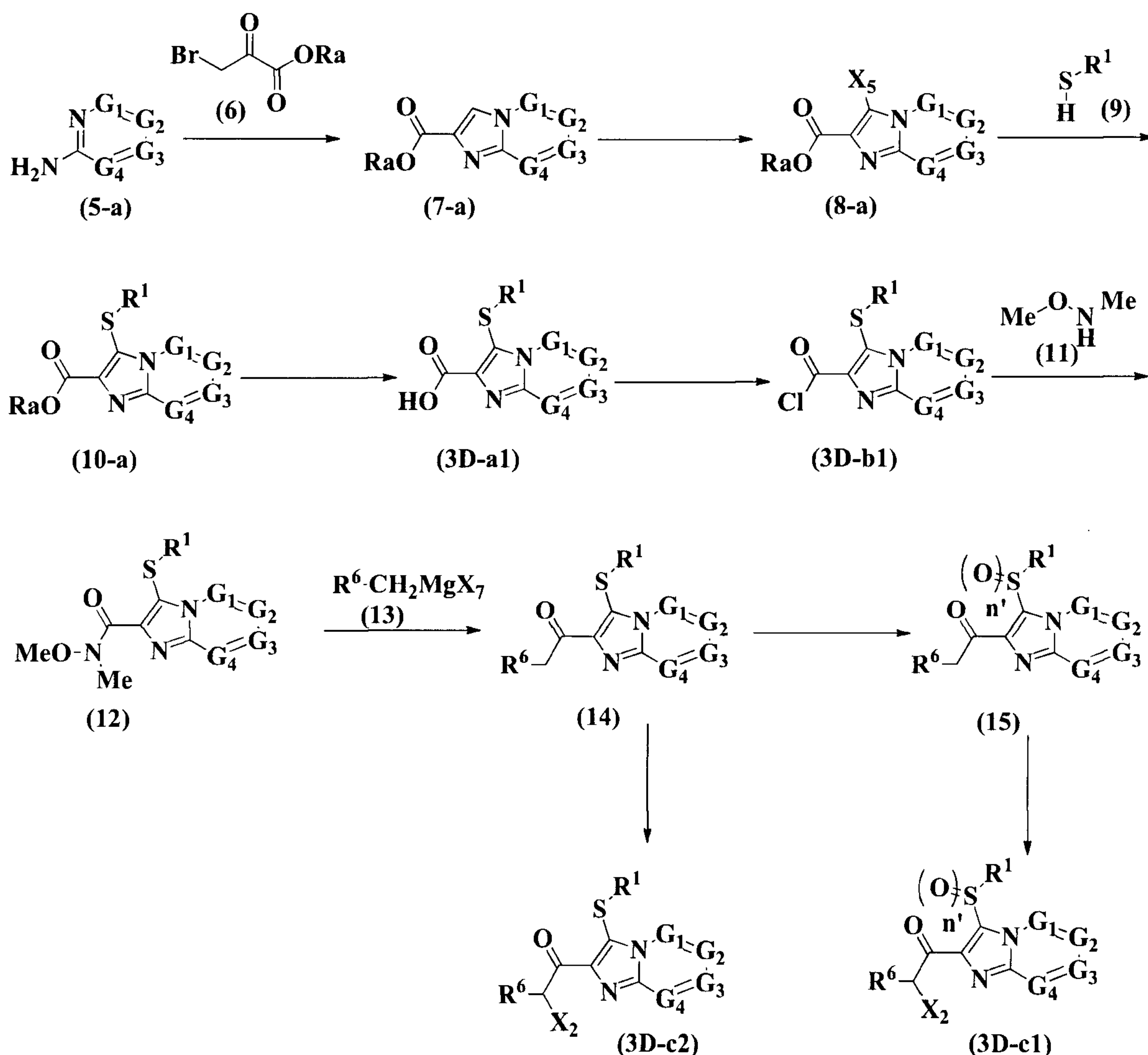
Reaction Scheme 1
