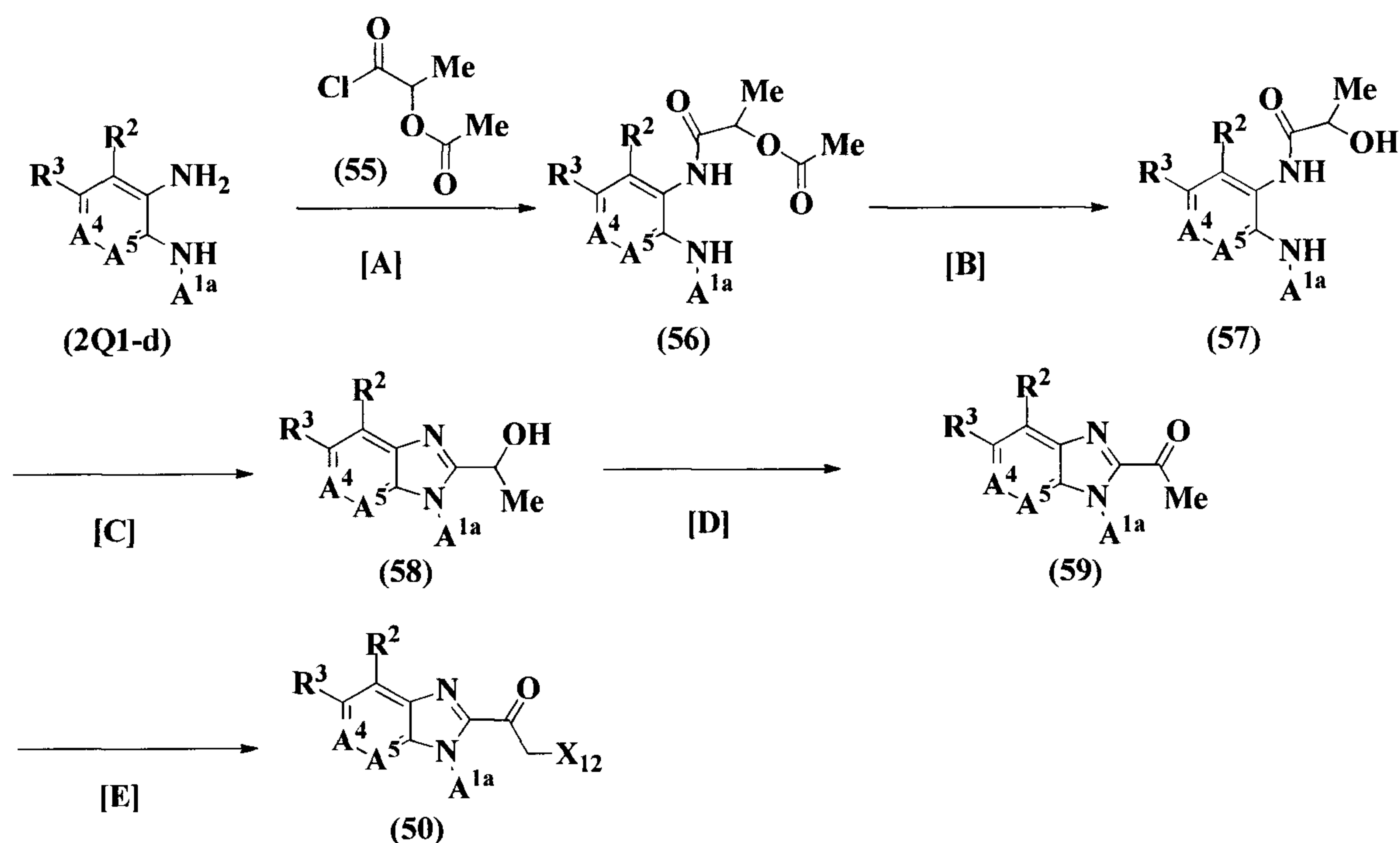
Reaction Scheme 9
