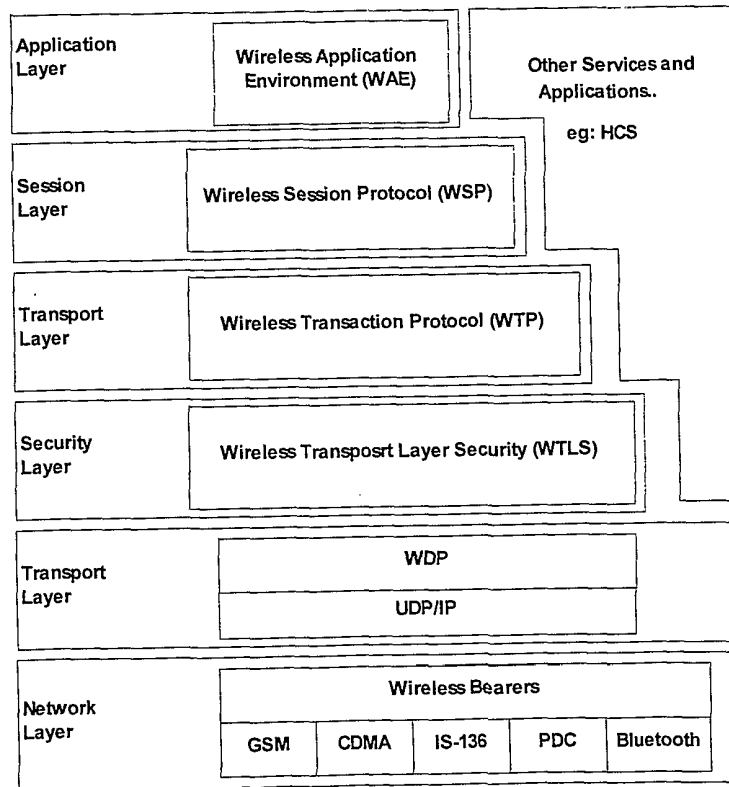
The Wireless Application Protocol Stack
