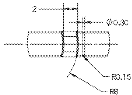
DETAIL VIEW D SCALE 4:1
