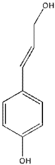
\beta coumaryl alcohol
