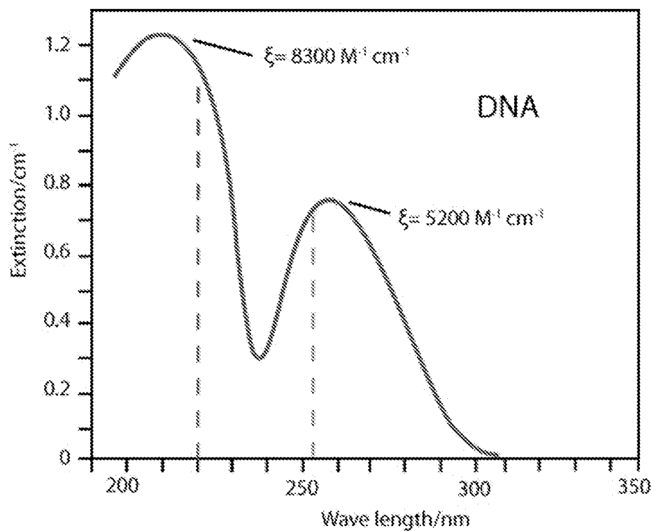
Figure 9: UV Absorption of DNA
