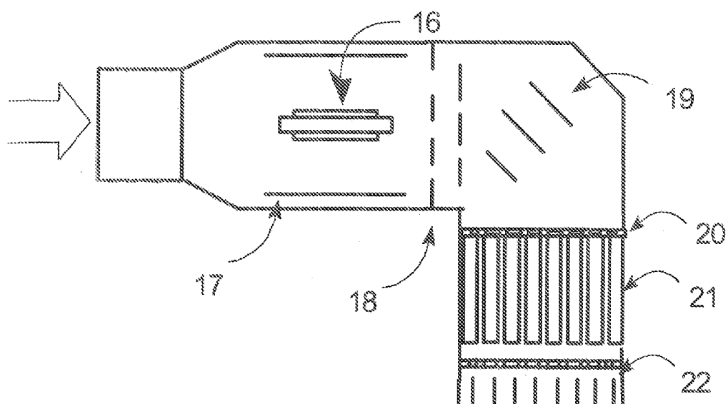
Figure 5: Zone Air Purifier & Sterilizer
