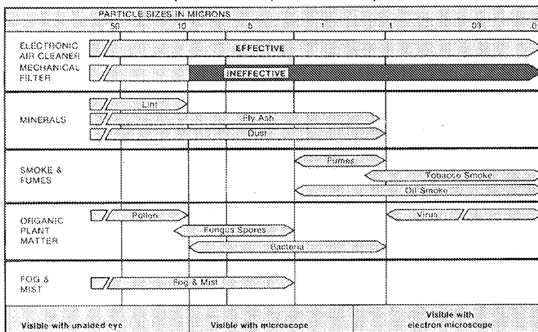
Figure 13: ESP range of effectiveness
