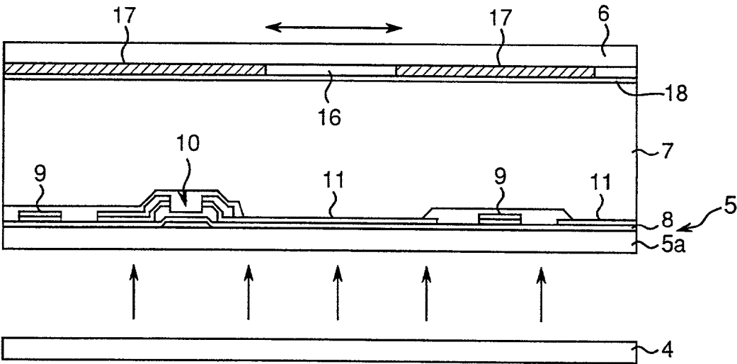
Fig.25 PRIOR ART
