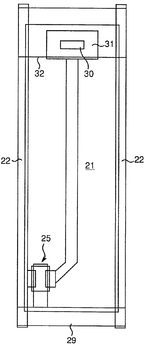
Fig.28 PRIOR ART
