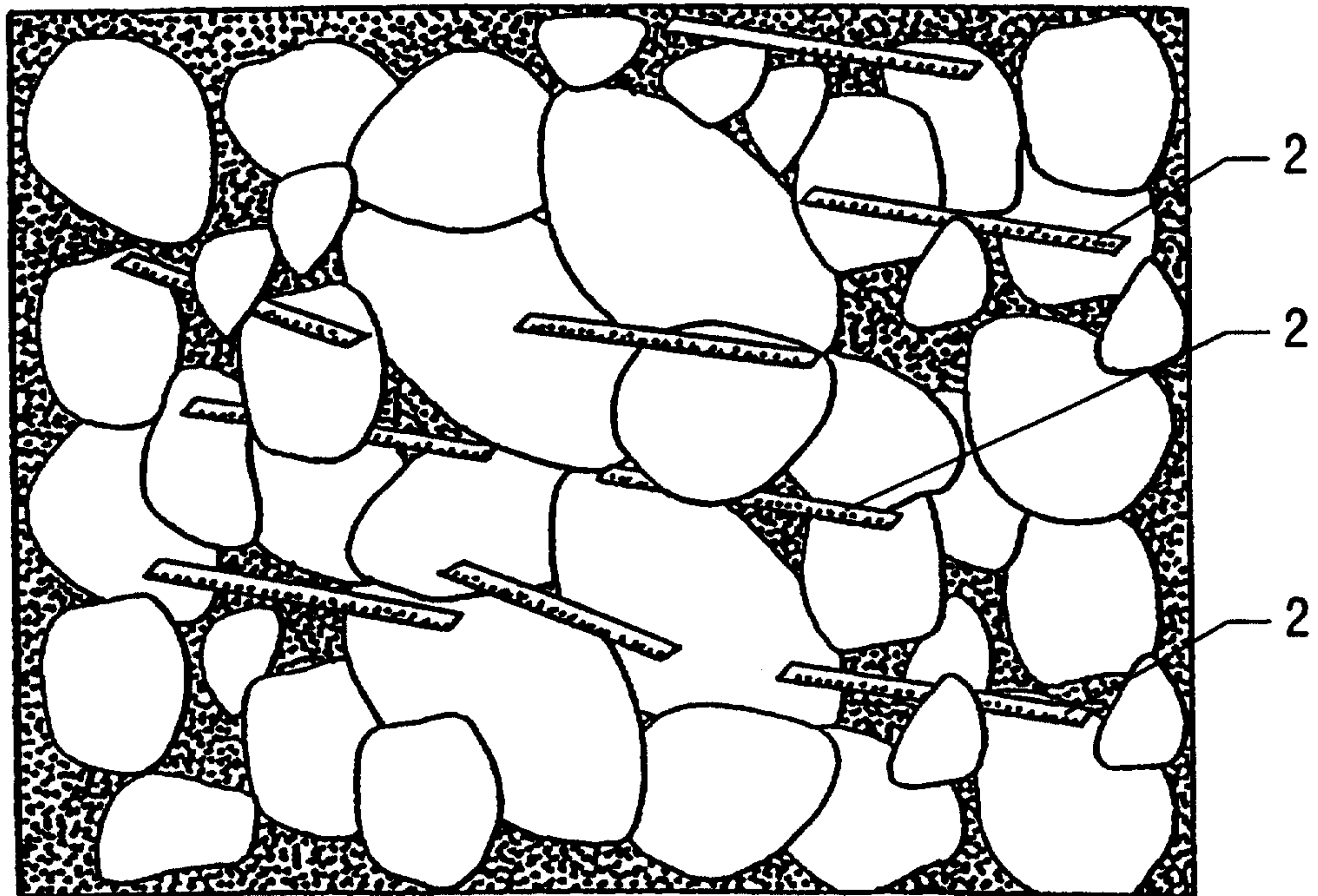
FIG. 1 (prior art)
