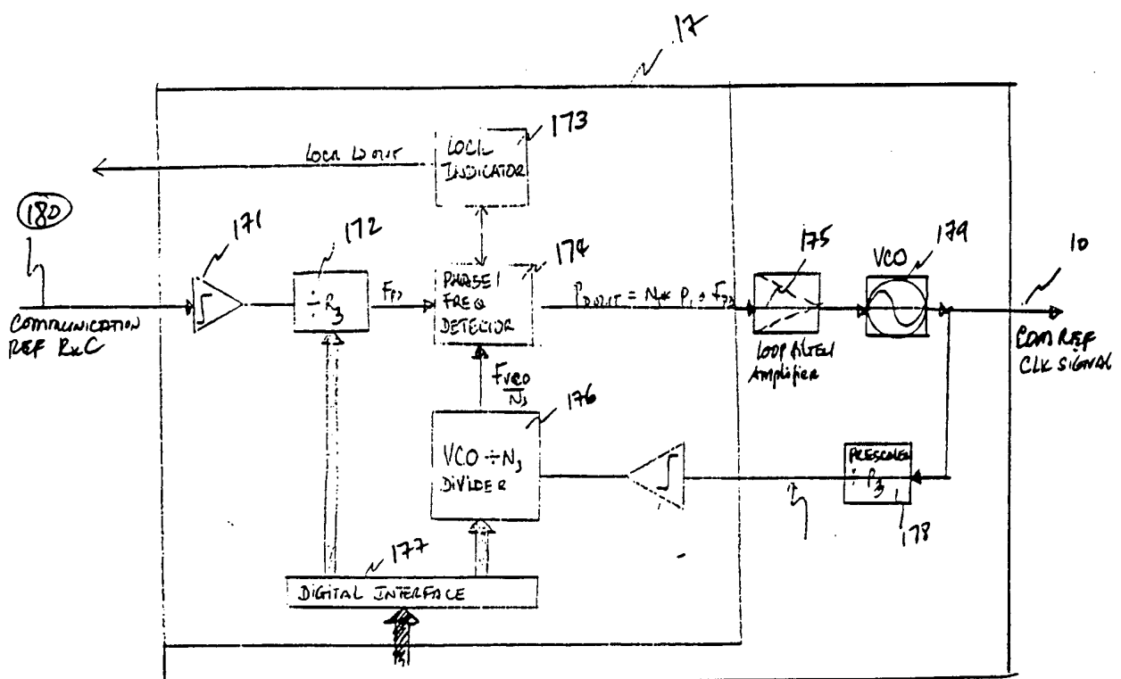
Com Ref Clock Generator (FIGURE 17)
