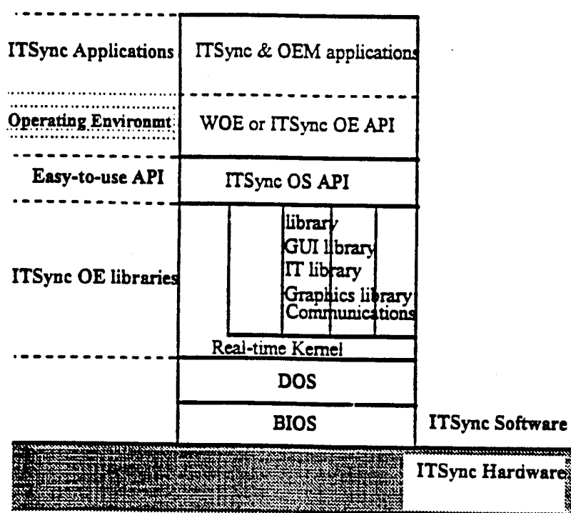
Figure/E - ITSync Software Architecture
