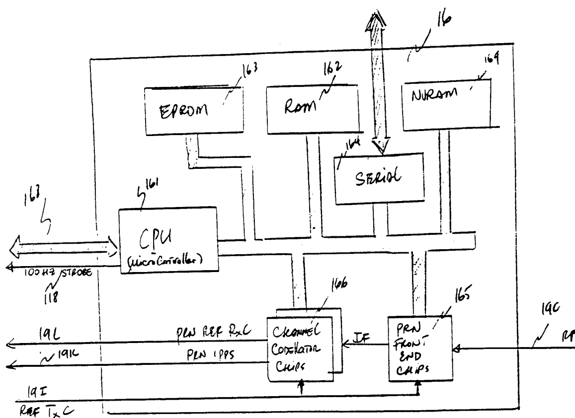
THE PRN RECEIVER (FIGURE 16)
