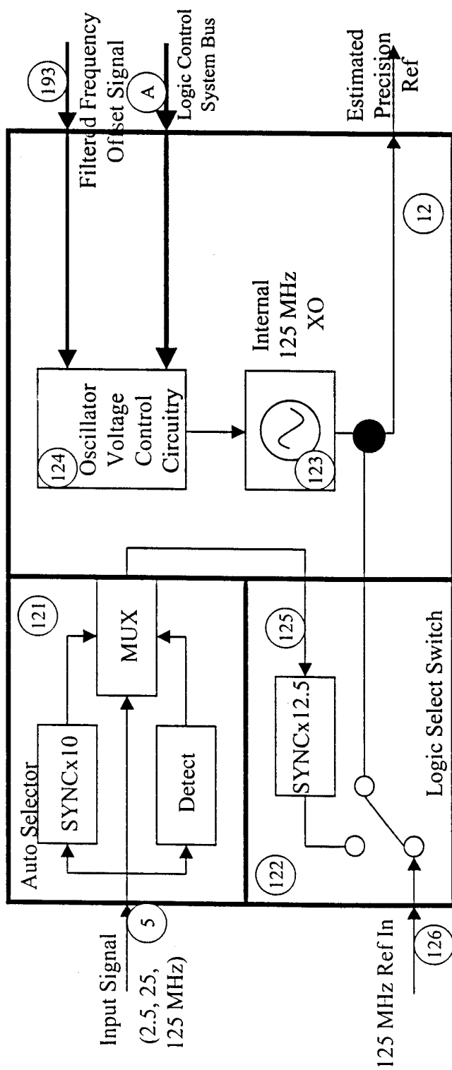
Oscillator Reference Clock Generator
