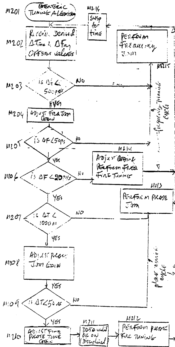
MODE 2 GENERIC TUNING ALGORITHM (FIGURE 9a)
