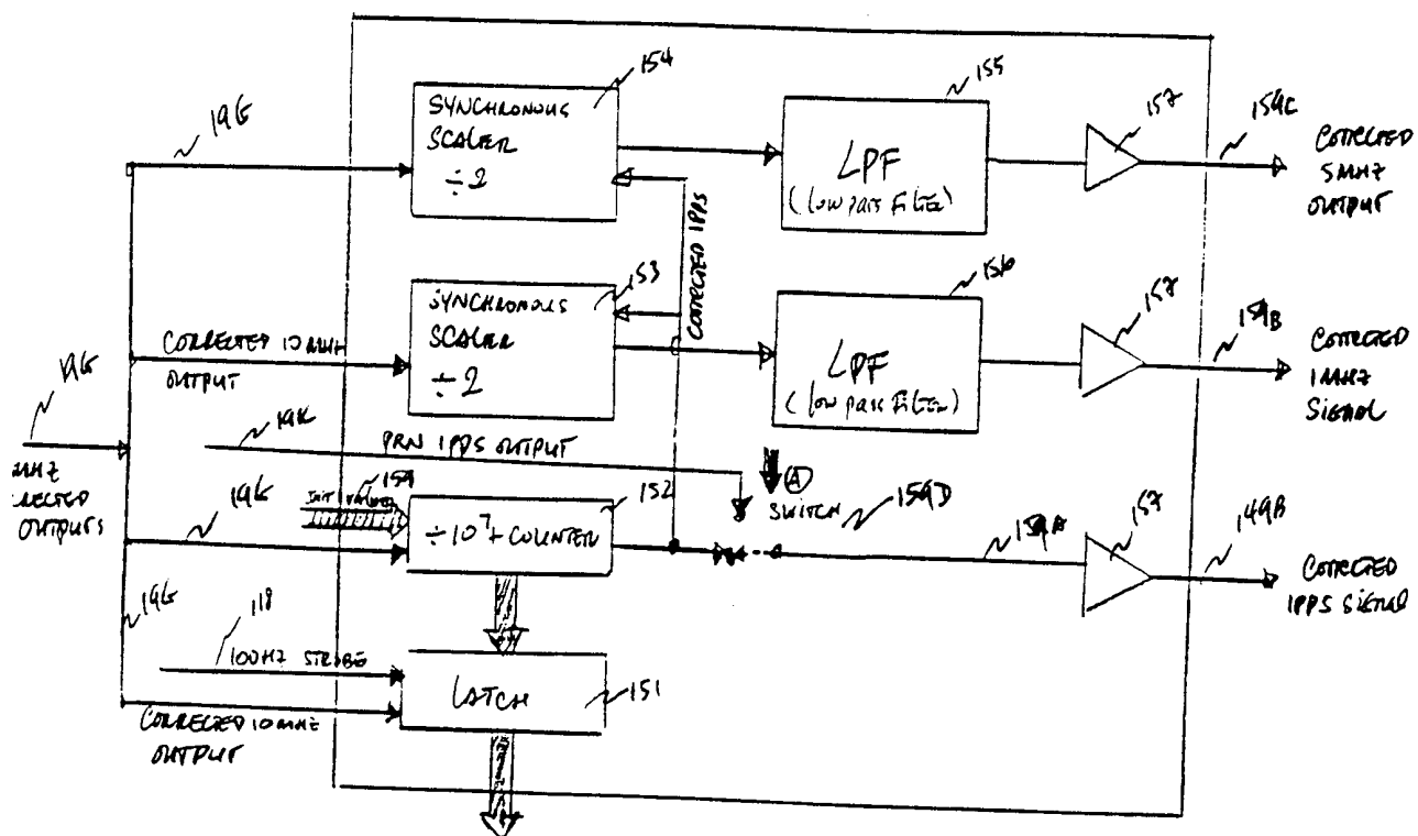
CORRECTED OUTPUT GENERATOR (FIGURE 15)
