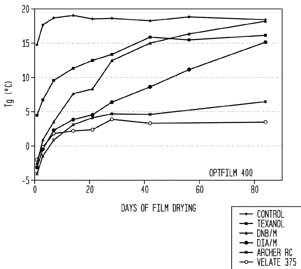
FIG. 11 RESIDUAL COALESCENT IN PAINT FILM - DSC ANALYSIS
