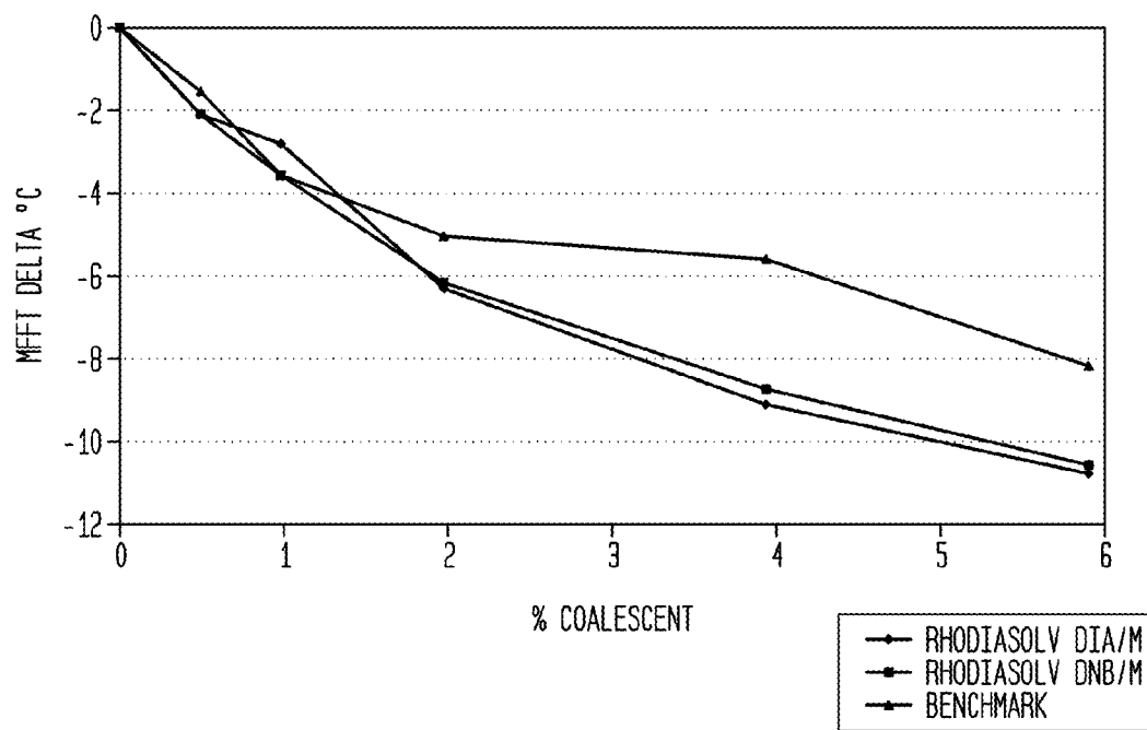
FIG. 7 MFFT RESULTS FOR VINYL-ACRYLIC RESIN
