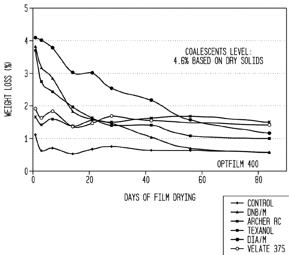
FIG. 10 RESIDUAL COALESCENT IN PAINT FILM - TGA ANALYSIS
