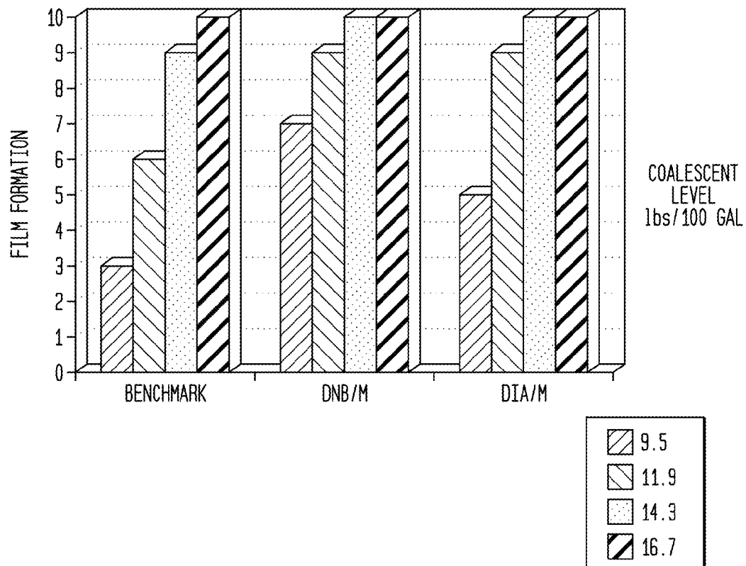
FIG. 8 LOW TEMPERATURE FILM FORMATION - SEMI-GLOSS PAINT
