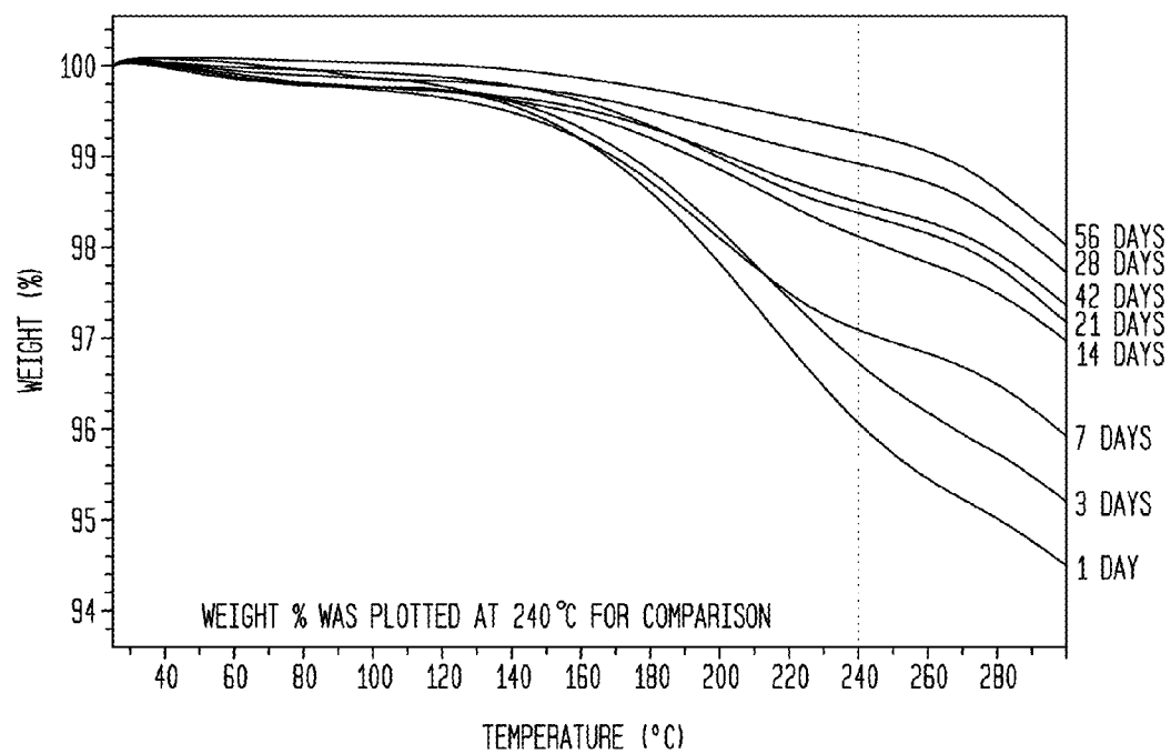
FIG. 9 RESIDUAL COALESCENTS IN DRIED PAINT FILM
