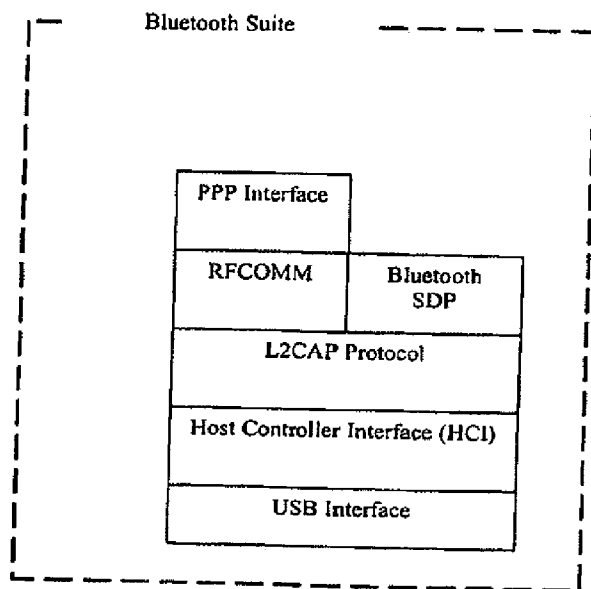
FIG. 4 BLUETOOTH SUITE
