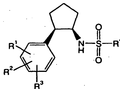
cis configuration formula I'
