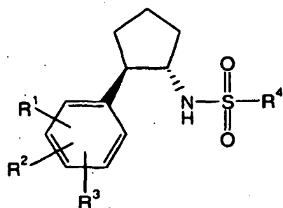
trans configuration formula I'
