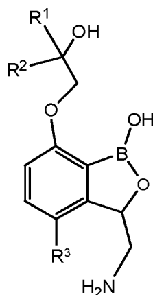
Formula III
