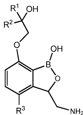
Formula III
