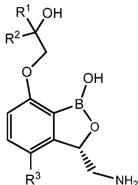
Formula IIIa
