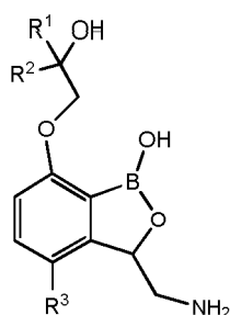
Formula III
