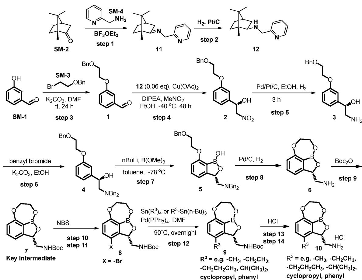
Scheme 1
