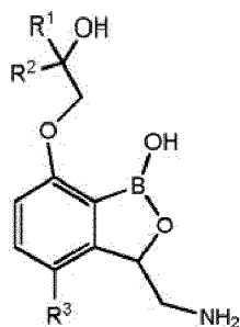
Formel III
