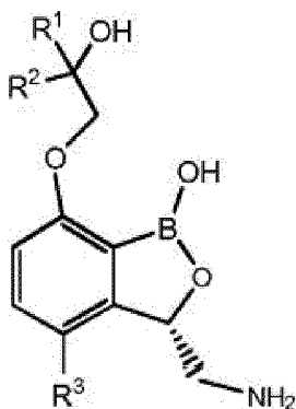
Formel IIIa
