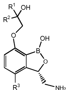
Formula IIIa
