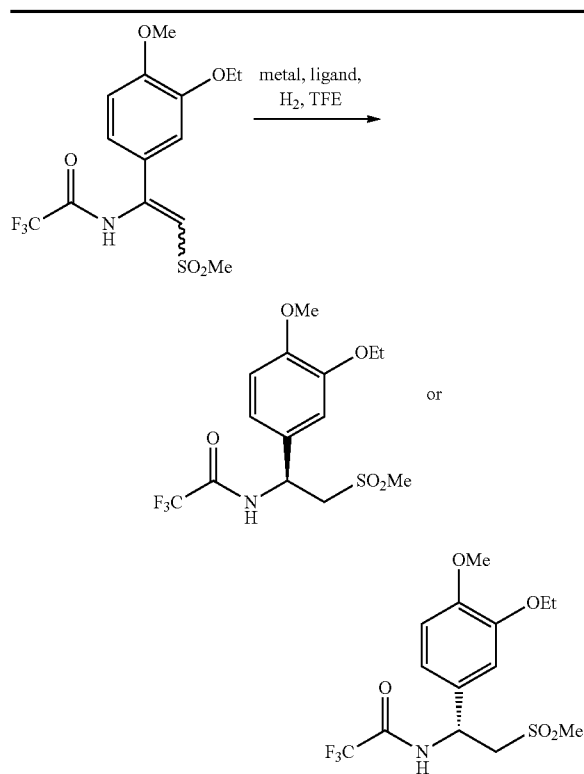
Asymmetric Hydrogenation of N-Trifluoroacetyl Enamine substrate a
