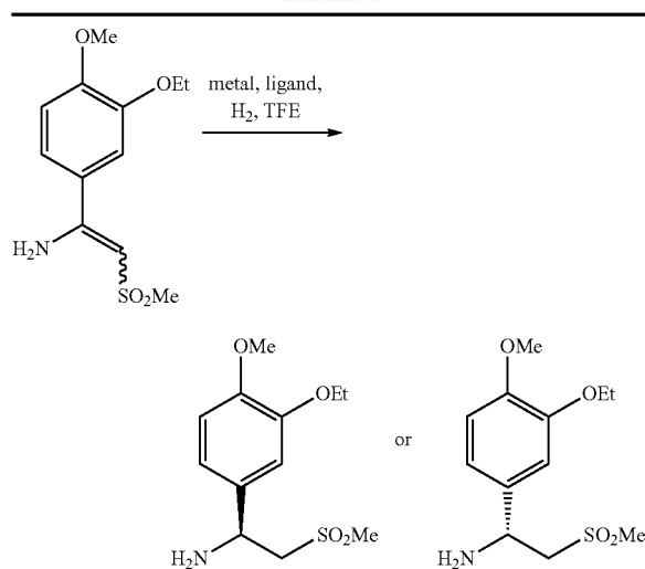
Asymmetric Hydrogenation of Enamine substrate a
