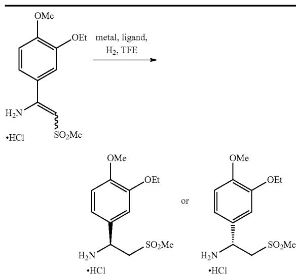
Asymmetric hydrogenation of enamine hydrochloride a
