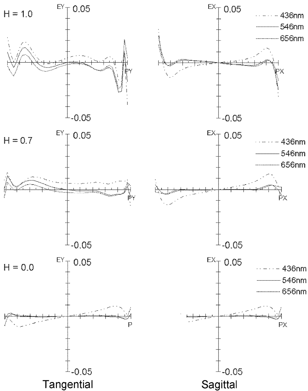
Lateral aberration (mm)
