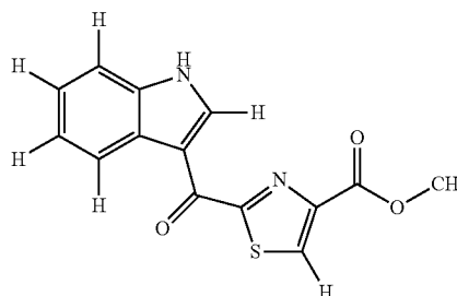
Structural Formula 1
