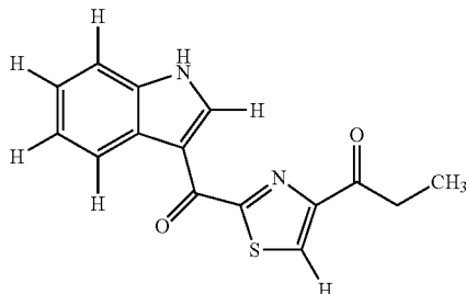
Structural Formula 2 5
