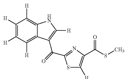
Structural Formula 3
