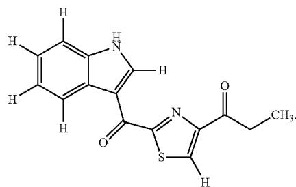
Structural Formula 2
