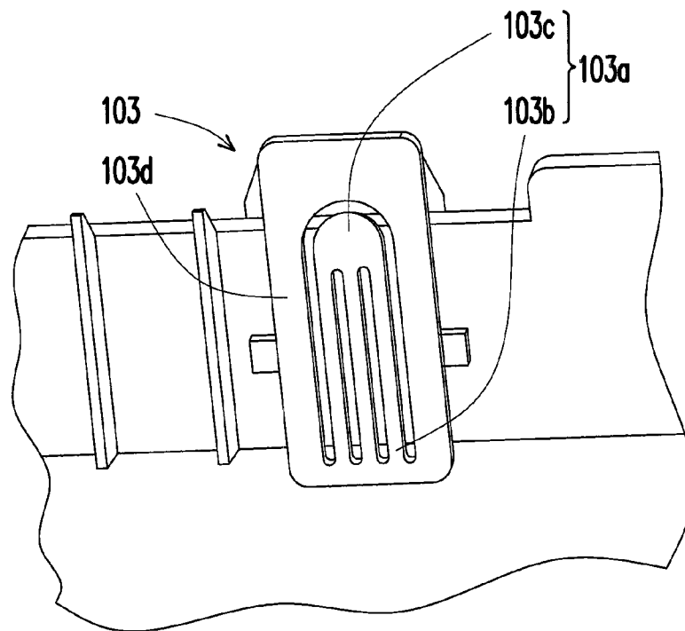
FIG. 2 (RELATED ART)
