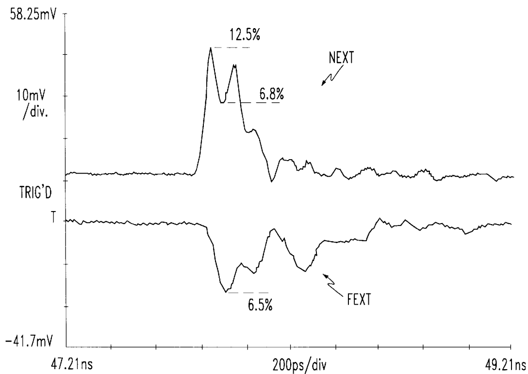
MEASURED CROSSTALK AT 35 PSEC.
