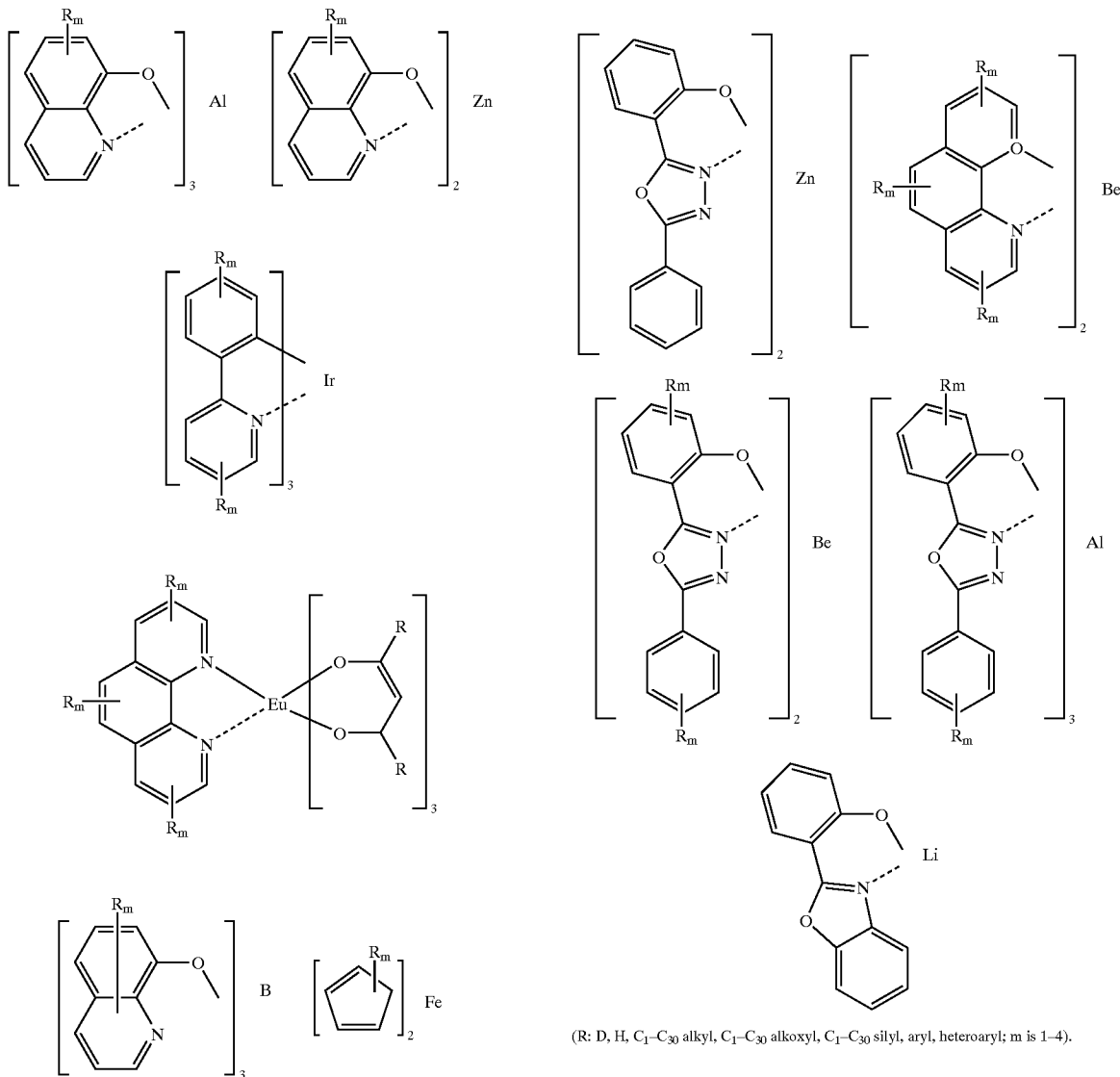
Scheme 4. Metal complexed organo-metallic compounds.
