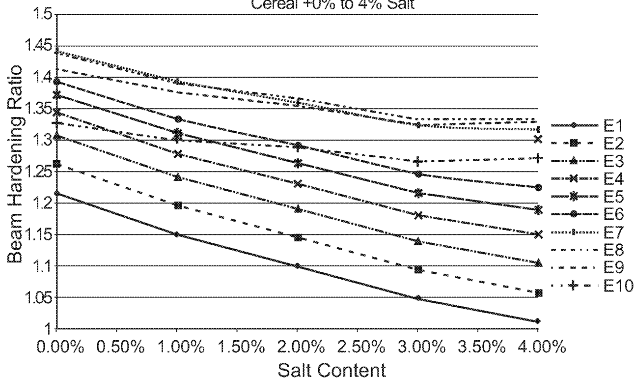
Fig. 3B Multi Energy Beam Hardening Curves for X-ray energies E1...E7 Cereal +0% to 4% Salt
