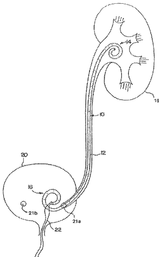
Fig. 2 (Prior Art)
