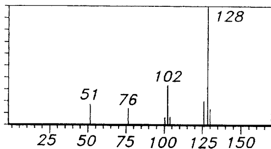
(4.2.2) PROPELLA- 2,4,7,9-TETRAENE
