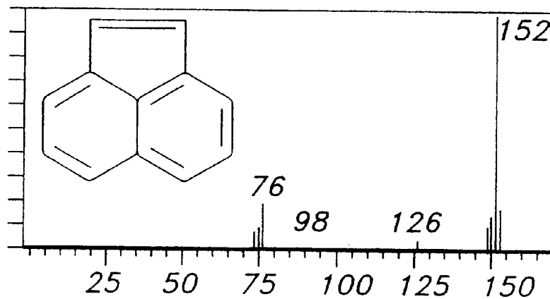
ACENAPHTHYLENE
