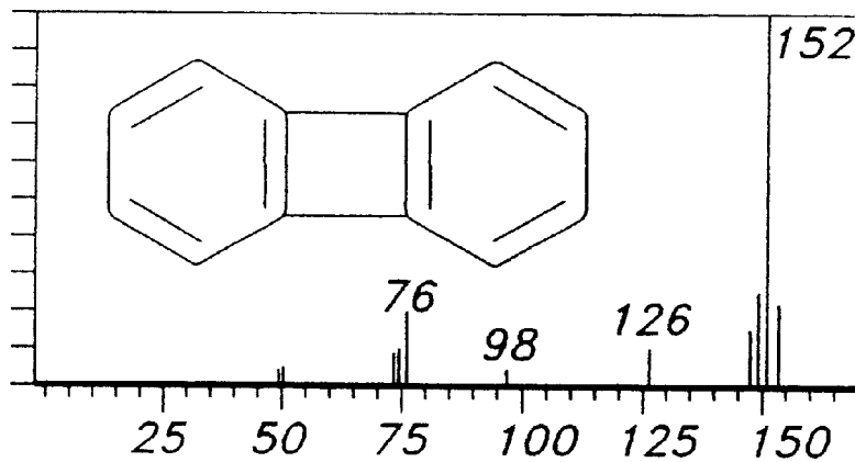
1,1'BIPHENYLENE
