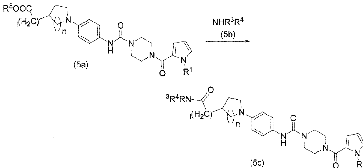
Reaction Scheme 5
