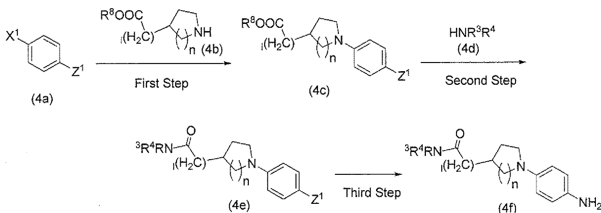
Reaction Scheme 4
