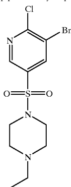
3-Bromo-2-chloro-5-(4-ethylpiperazin-1-ylsulphonyl)pyridine
