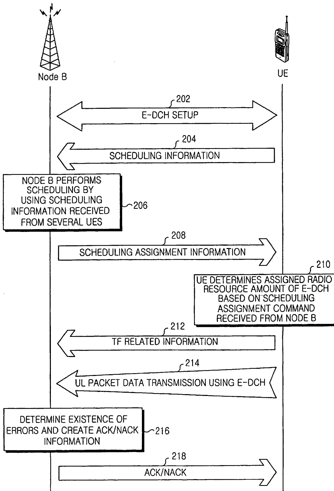
FIG. 2 (RELATED ART)
