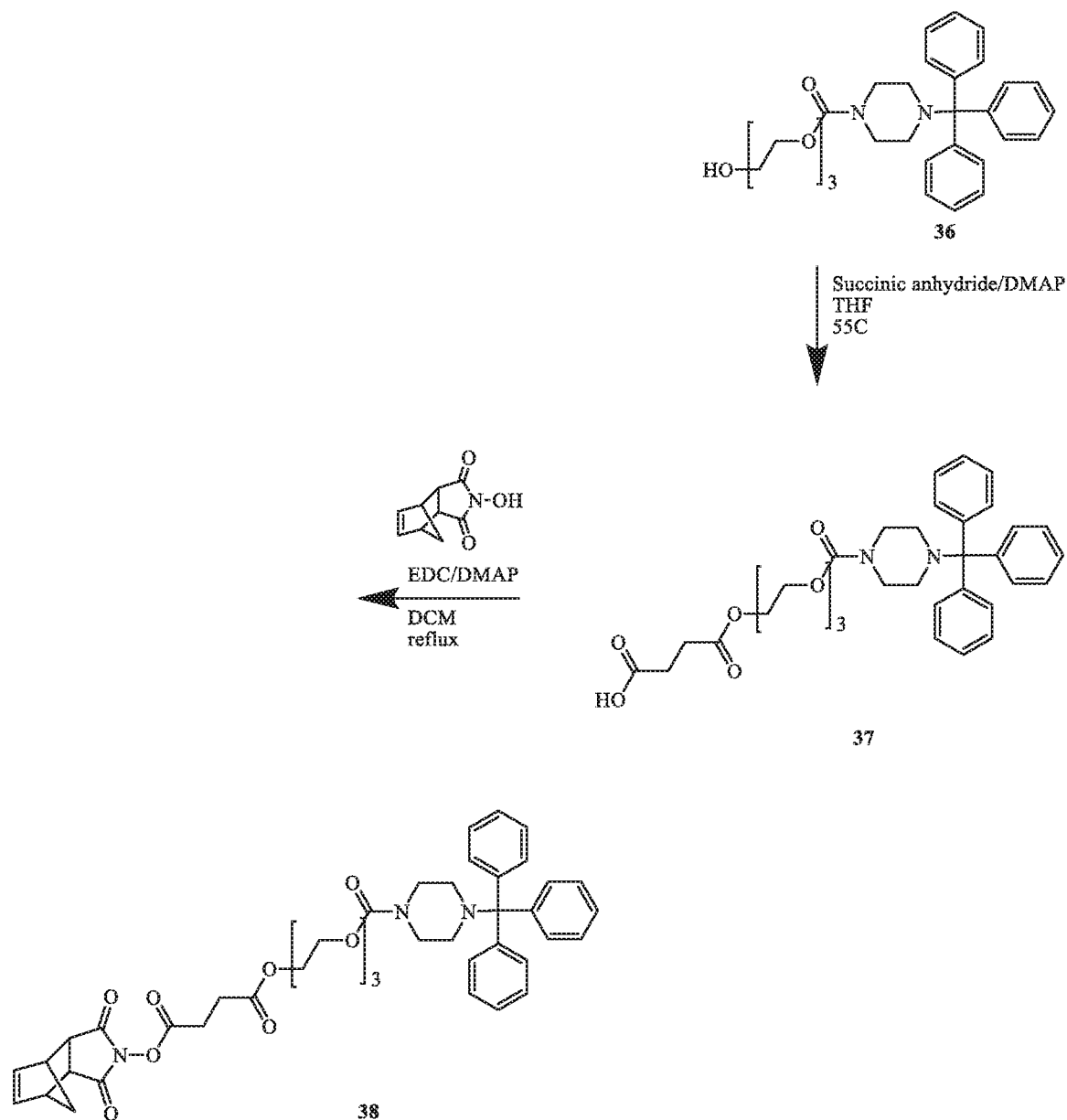
Scheme 2: Preparation of Activated Tail Acid
