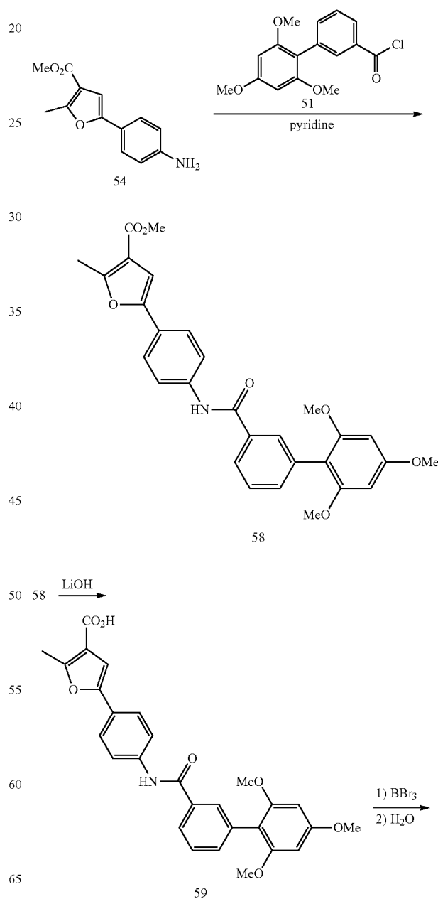
SCHEME 13
