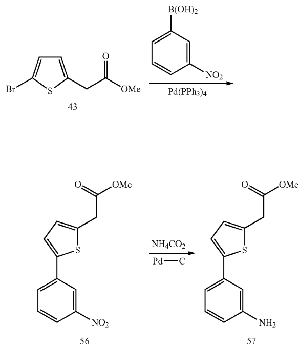
SCHEME 12
