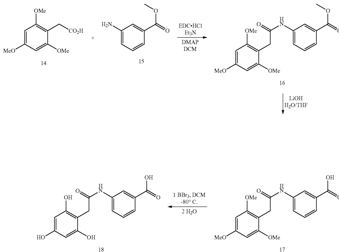
SCHEME 4
