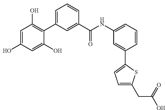
SCHEME 17
