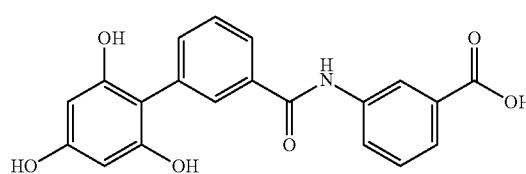
SCHEME 20
