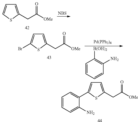
SCHEME 7
