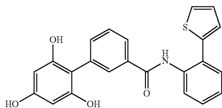
SCHEME 18
