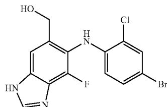
[6-(4-Bromo-2-chloro-phenylamino)-7-fluoro-3H-benzimidazol-5-yl]-methanol(10e)
