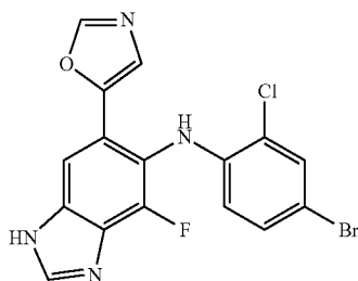
(4-Bromo-2-chloro-phenyl)-(4-fluoro-6-oxazol-5-yl)-1H-benzimidazol-5-yl-amine (10x)
