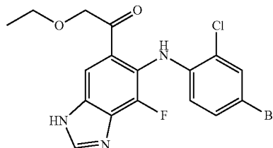
1-[6-(4-Bromo-2-chloro-phenylamino)-7-fluoro-3H-benzimidazol-5-yl]-2-ethoxy-ethanone (10n)
