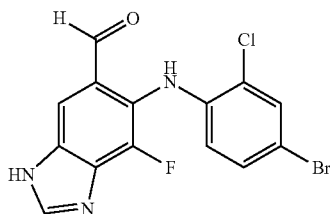
6-(4-Bromo-2-chloro-phenylamino)-7-fluoro-3H-benzimidazole-5-carbaldehyde (10f)
