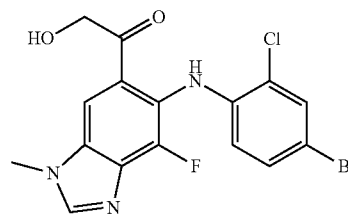
1-[6-(4-Bromo-2-chloro-phenylamino)-7-fluoro-3-methyl-3H-benzimidazol-5-yl]-2-hydroxyethanone (10 g)
