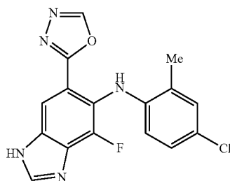
(4-Chloro-2-methyl-phenyl)-(4-fluoro-6-[1,3,4]oxadiazol-2-yl)-1H-benzimidazol-5-yl-amine (21a)
