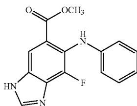
7-Fluoro-6-phenylamino-3H-benzimidazole-5-carboxylic acid methyl ester (27a)
