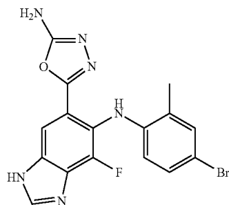
[6-(5-Amino-[1,3,4]oxadiazol-2-yl)-4-fluoro-1H-benzimidazol-5-yl]-(4-bromo-2-methyl-phenyl)-amine (24a)
