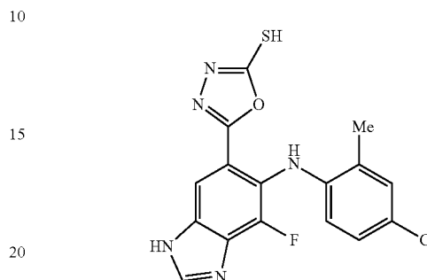
5-[6-(4-Chloro-2-methyl-phenylamino)-7-fluoro-3H-benzimidazol-5-yl]-[1,3,4]oxadiazole-2-thiol (23a)
