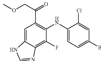
1-[6-(4-Bromo-2-chloro-phenylamino)-7-fluoro-3H-benzimidazol-5-yl]-2-methoxy-ethanone (10p)
