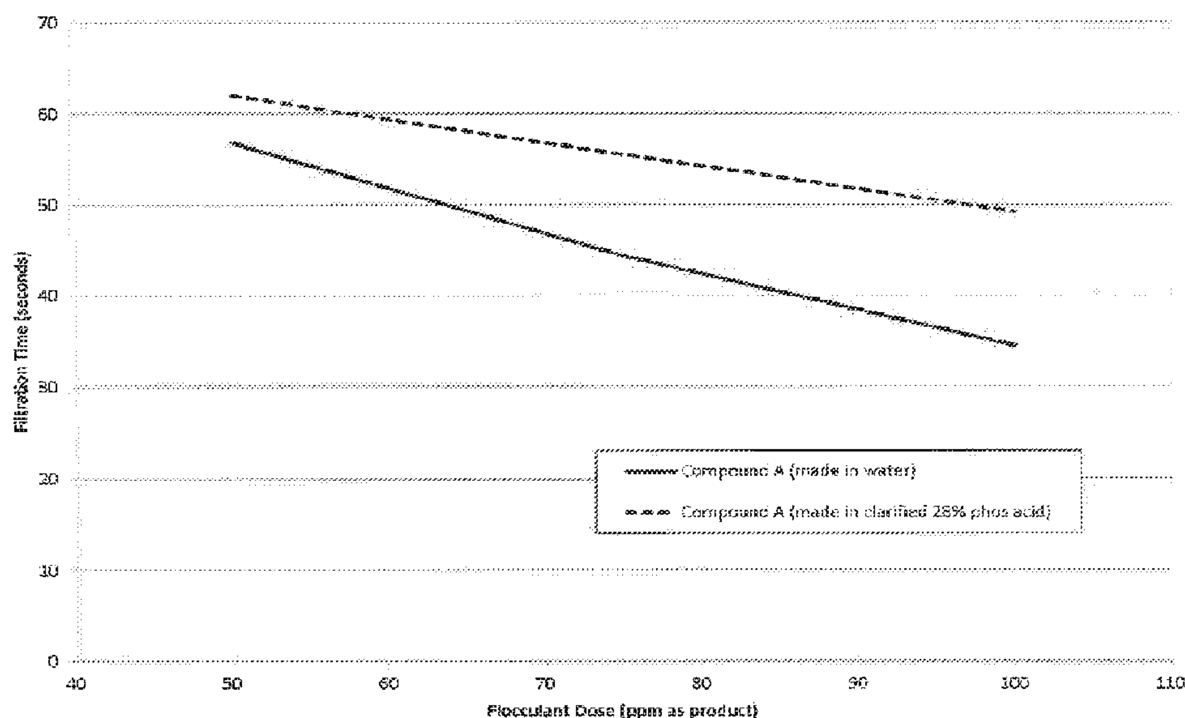
Gypsum slurry filtration using flocculant diluted with water and with clarified phosphoric acid filtrate
