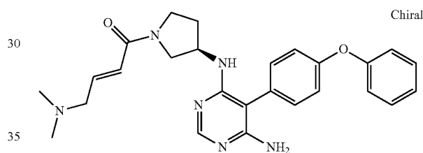
(R,E)-1-(3-(((6-amino-5-(4-phenoxyphenyl)pyrimidin-4-yl)amino)pyrrolidin-1-yl)-4-(dimethylamino)but-2-en-1-one (A73)
