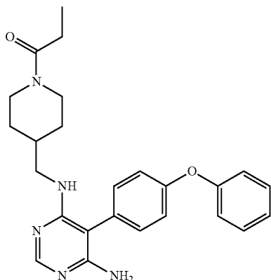
1-(4-(((6-amino-5-(4-phenoxyphenyl)pyrimidin-4-yl)amino)methyl)piperidin-1-yl)propan-1-one (A333)
