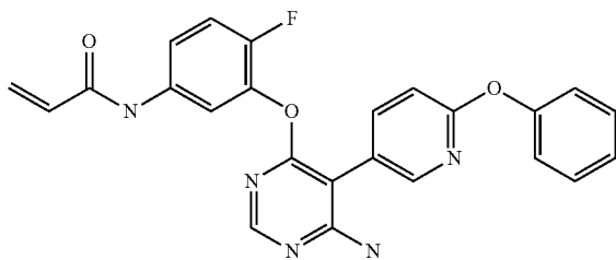
N-(3-((6-amino-5-(6-phenoxyphenyl)pyrimidin-4-yl)oxy)-4-fluorophenyl)acrylamide (A161)
