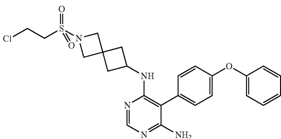
N^4 -(2-((2-chloroethyl)sulfonyl)-2-azaspiro[3.3]heptan-6-yl)-5-(4-phenoxyphenyl)pyrimidine-4,6-diamine (A119)
