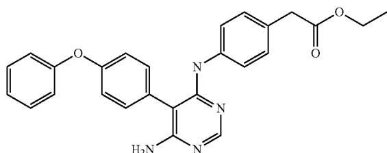
(4-(6-Amino-5-(4-phenoxyphenyl)-pyrimidin-4-ylamino)-phenyl)-acetic acid ethyl ester
