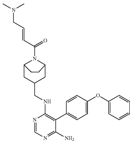
(E)-1-(3-(((6-amino-5-(4-phenoxyphenyl)pyrimidin-4-yl)amino)methyl)-8-azabicyclo[3.2.1]octan-8-yl)-4-(dimethylamino)but-2-en-1-one (A71)
