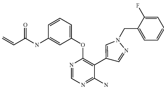
N-(3-((6-amino-5-(1-(2-fluorobenzyl)-1H-pyrazol-4-yl)pyrimidin-4-yl)oxy)phenyl)acrylamide (A184)
