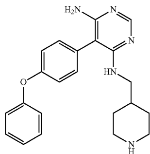
5-(4-phenoxyphenyl)-N-(piperidin-4-ylmethyl)pyrimidine-4,6-diamine
