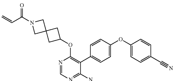
4-(4-(4-((2-acryloyl-2-azaspiro[3.3]heptan-6-yl)oxy)-6-aminopyrimidin-5-yl)phenoxy)benzonitrile (A202)
