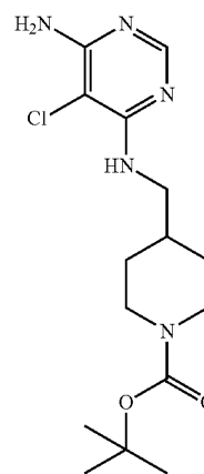
tert-butyl 4-(((6-amino-5-chloropyrimidin-4-yl)amino)methyl)piperidine-1-carboxylate
