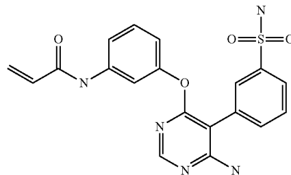
N-(3-((6-amino-5-(3-sulfamoylphenyl)pyrimidin-4-yl)oxy)phenyl)acrylamide (A163)
