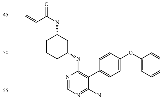
N-((1S,3R)-3-(((6-amino-5-(4-phenoxyphenyl)pyrimidin-4-yl)amino)cyclohexyl)acrylamide (A173)
