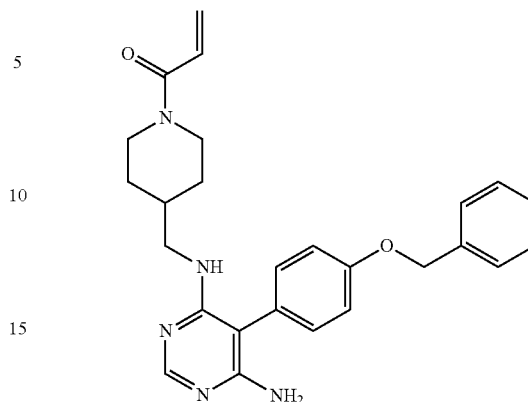
1-(4-((6-amino-5-(4-(benzyloxy)phenyl)pyrimidin-4-yl)amino)methyl)piperidin-1-yl)prop-2-en-1-one (A292)
