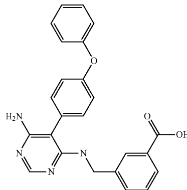
3-((6-Amino-5-(4-phenoxy-phenyl)-pyrimidin-4-ylamino)-methyl)-benzoic acid (134)
