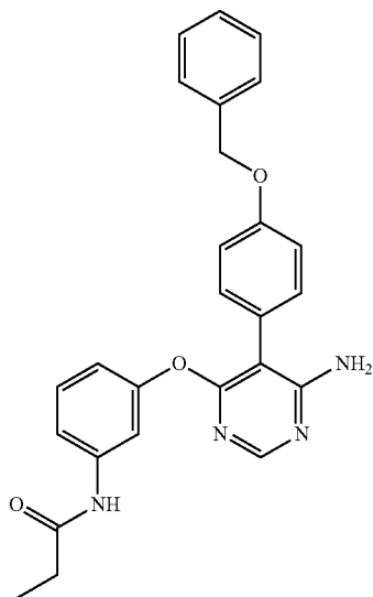
N-{3-[6-Amino-5-(4-benzyloxy-phenyl)-pyrimidin-4-yloxy]-phenyl}-propionamide (A346)
