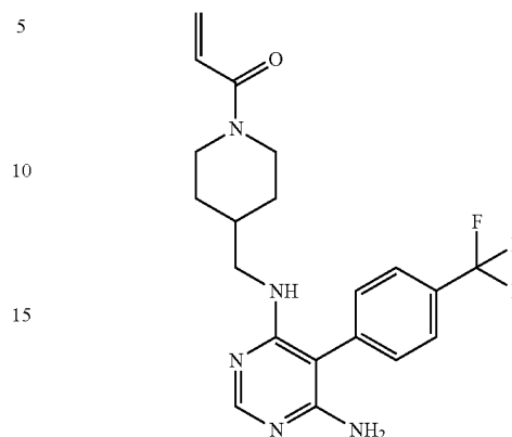
1-(4-(((6-amino-5-(4-(4-(trifluoromethyl)phenyl)pyrimidin-4-yl)amino)methyl)piperidin-1-yl)prop-2-en-1-one (A81)
