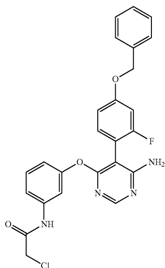
N-{3-[6-Amino-5-(4-benzyloxy-2-fluoro-phenyl)-pyrimidin-4-yloxy]-phenyl}-2-chloro-acetamide (A350)
