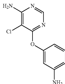
6-(3-aminophenoxy)-5-chloropyrimidin-4-amine
