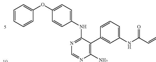
N-(3-(4-amino-6-((4-phenoxyphenyl)amino)pyrimidin-5-yl)phenyl)acrylamide (A241)
