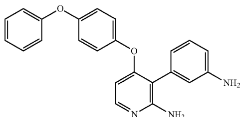
3-(3-aminophenyl)-4-(4-phenoxyphenoxy)pyridin-2-amine (A300)
