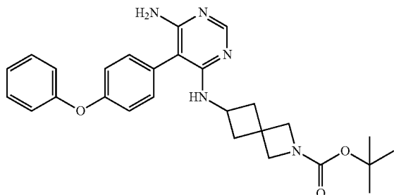
tert-butyl 6-((6-amino-5-(4-phenoxyphenyl)pyrimidin-4-yl)amino)-2-azaspiro[3.3]heptane-2-carboxylate
