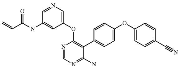
N-(5-((6-amino-5-(4-(4-cyanophenoxy)phenyl)pyrimidin-4-yl)oxy)pyridin-3-yl)acrylamide (A197)
