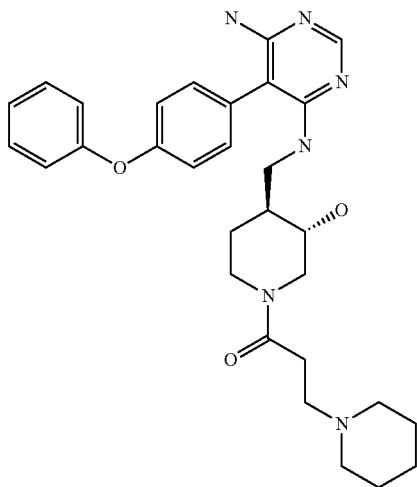
1-((3S,4S)-4-(((6-amino-5-(4-phenoxyphenyl)pyrimidin-4-yl)amino)methyl)-3-hydroxypiperidin-1-yl)-3-(piperidin-1-yl)propan-1-one (A233)
