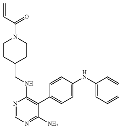
1-(4-(((6-amino-5-(4-(phenylamino)phenyl)pyrimidin-4-yl)amino)methyl)piperidin-1-yl)prop-2-en-1-one (A39)
