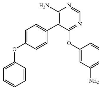
6-(3-aminophenoxy)-5-(4-phenoxyphenyl)pyrimidin-4-amine
