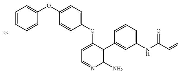
N-(3-(2-amino-4-(4-phenoxyphenoxy)pyridin-3-yl)phenyl)acrylamide (A243)
