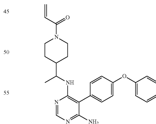
1-(4-(1-((6-amino-5-(4-phenoxyphenyl)pyrimidin-4-yl) amino)ethyl)piperidin-1-yl)prop-2-en-1-one (A332)
