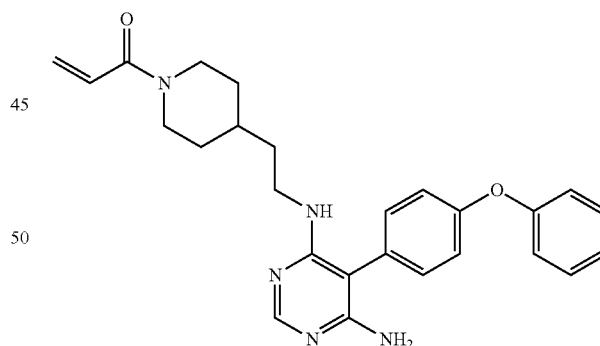
1-(4-(2-(((6-amino-5-(4-phenoxyphenyl)pyrimidin-4-yl)amino)ethyl)piperidin-1-yl)prop-2-en-1-one (A16)
