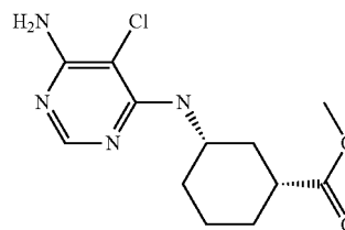
(1R,3S)-3-(6-Amino-5-chloro-pyrimidin-4-ylamino)-cyclohexanecarboxylic acid methyl ester (A130)
