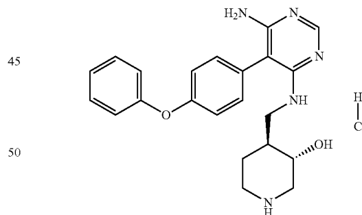
(3S,4S)-4-(((6-amino-5-(4-(phenoxyphenyl)pyrimidin-4-yl)amino)methyl)piperidin-3-ol) hydrochloride (A101)
