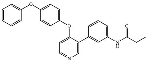
N-(3-(4-(4-phenoxyphenoxy)pyridin-3-yl)phenyl)propionamide (A319)
