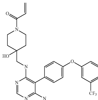
1-(4-(((6-amino-5-(4-(3-(trifluoromethyl)phenoxy)phenyl)pyrimidin-4-yl)amino)methyl)-4-hydroxypiperidin-1-yl)prop-2-en-1-one (A169)
