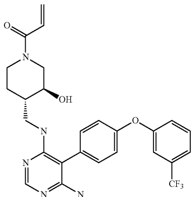
1-((3S,4S)-4-(((6-amino-5-(4-(3-(trifluoromethyl)phenoxy)phenyl)pyrimidin-4-yl)amino)methyl)-3-hydroxypiperidin-1-yl)prop-2-en-1-one (A170)
