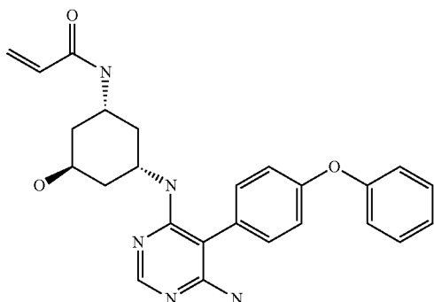
N-((1R,3S,5R)-3-((6-amino-5-(4-phenoxyphenyl)pyrimidin-4-yl)amino)-5-hydroxycyclohexyl)acrylamide (racemic) (A188)
