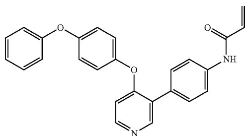
N-(4-(4-(4-phenoxyphenoxy)pyridin-3-yl)phenyl)acrylamide (A281)
