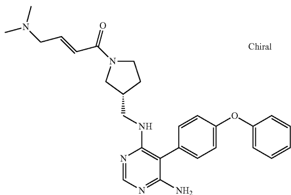
(R,E)-1-(3-(((6-amino-5-(4-phenoxyphenyl)pyrimidin-4-yl)amino)methyl)pyrrolidin-1-yl)-4-(dimethylamino)but-2-en-1-one (A62)
