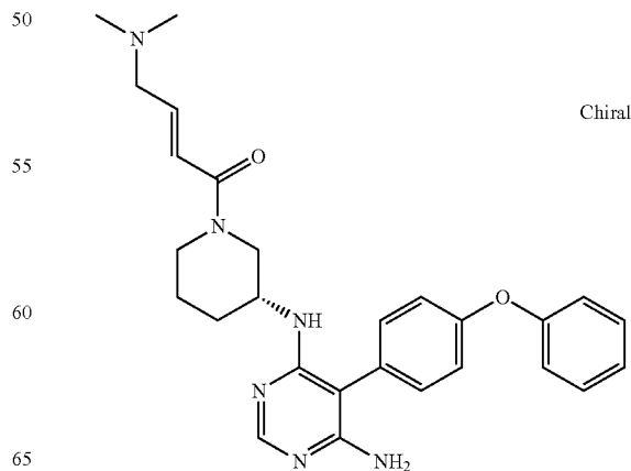
(E)-1-(3-(((6-amino-5-(4-phenoxyphenyl)pyrimidin-4-yl)amino)methyl)-8-azabicyclo[3.2.1]octan-8-yl)-4-(dimethylamino)but-2-en-1-one (A71)
