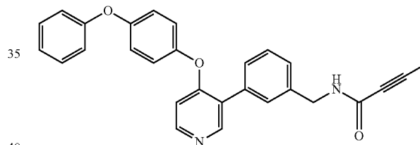
N-(3-(4-(4-phenoxyphenoxy)pyridin-3-yl)benzyl)but-2-enamide (A304)
