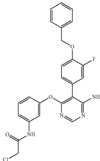
N-{3-[6-Amino-5-(4-benzyloxy-3-fluoro-phenyl)-pyrimidin-4-yloxy]-phenyl}-2-chloro-acetamide (A351)
