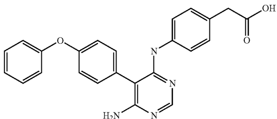
(4-(6-Amino-5-(4-phenoxyphenyl)-pyrimidin-4-ylamino)-phenyl)-acetic acid
