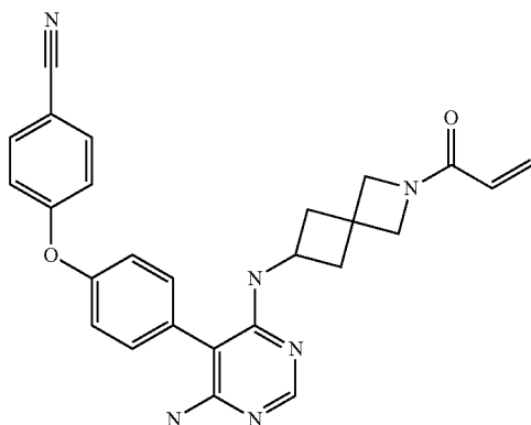
4-(4-(4-((2-acryloyl-2-azaspiro[3.3]heptan-6-yl)amino)-6-aminopyrimidin-5-yl)phenoxy)benzonitrile (A207)
