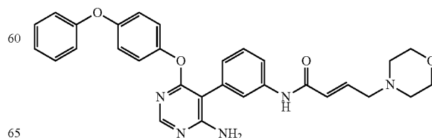
N-(3-((2-amino-5-(4-phenoxyphenyl)pyrimidin-4-yl)oxy)phenyl)acrylamide (A271)
