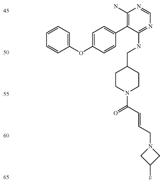
1-acryloyl-4-(((6-amino-5-(4-phenoxyphenyl)pyrimidin-4-yl)amino)methyl)piperidine-4-carboxylic acid (A216)
