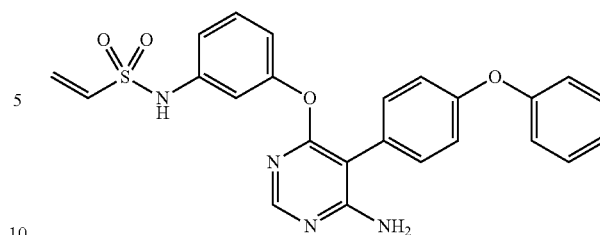
N-(3-((6-amino-5-(4-phenoxyphenyl)pyrimidin-4-yl)oxy)phenyl)ethanesulfonamide (A58)
