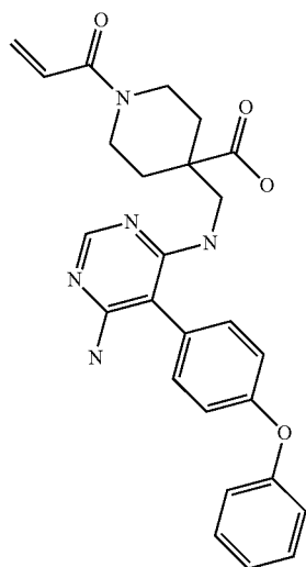
1-acryloyl-4-(((6-amino-5-(4-phenoxyphenyl)pyrimidin-4-yl)amino)methyl)piperidine-4-carboxylic acid (A216)
