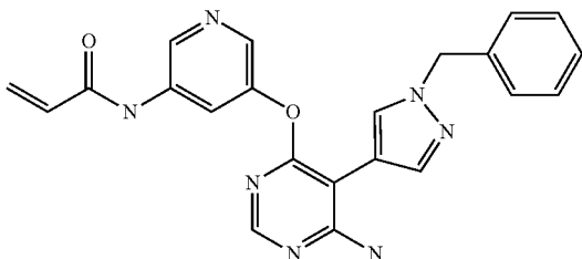
N-((1R,3S,5R)-3-((6-amino-5-(4-phenoxyphenyl)pyrimidin-4-yl)amino)-5-hydroxycyclohexyl)acrylamide (racemic) (A188)
