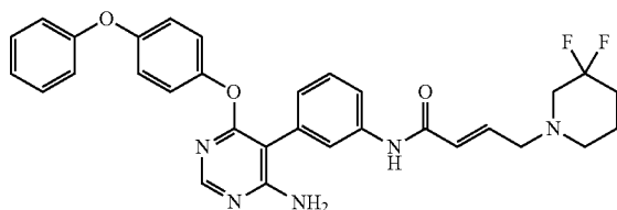
(E)-N-(3-(4-amino-6-(4-phenoxyphenoxy)pyrimidin-5-yl)phenyl)-4-(3,3-difluoropiperidin-1-yl)but-2-enamide (A301)
