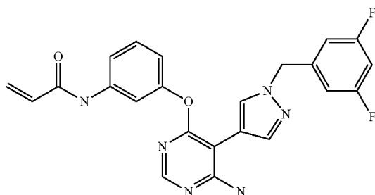
N-(3-((6-amino-5-(1-(3,5-difluorobenzyl)-1H-pyrazol-4-yl)pyrimidin-4-yl)oxy)phenyl)acrylamide (A183)
