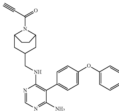
1-(3-(((6-amino-5-(4-phenoxyphenyl)pyrimidin-4-yl)amino)methyl)-8-azabicyclo[3.2.1]octan-8-yl)prop-2-yn-1-one (A68)
