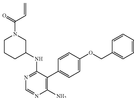
1-(3-((6-amino-5-(4-(benzyloxy)phenyl)pyrimidin-4-yl)amino)piperidin-1-yl)prop-2-en-1-one (A269)
