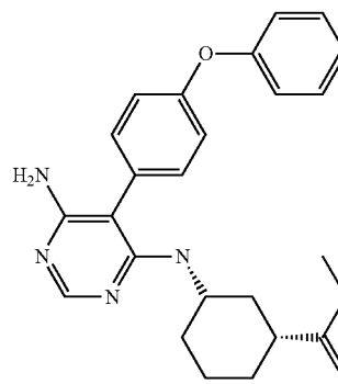
(1R,3S)-3-(6-Amino-5-(4-phenoxyphenyl)-pyrimidin-4-ylamino)-cyclohexanecarboxylic acid methyl ester (A133)
