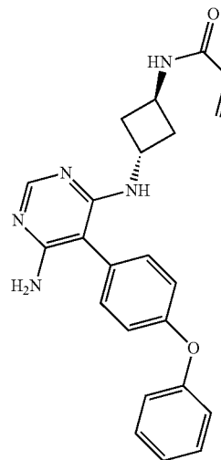
N-(1,3-trans-3-((6-amino-5-(4-phenoxyphenyl)pyrimidin-4-yl)amino)cyclobutyl)acrylamide (A117)
