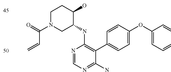
1-((3R,4R)-3-(((6-amino-5-(4-phenoxyphenyl)pyrimidin-4-yl)amino)-4-hydroxypiperidin-1-yl)prop-2-en-1-one (racemic) (A210)
