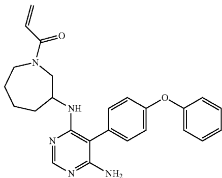
1-(3-((6-amino-5-(4-phenoxyphenyl)pyrimidin-4-yl)amino)azepan-1-yl)prop-2-en-1-one (A52)
