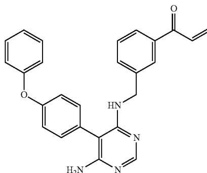
1-(3-((Amino-5-(4-phenoxyphenyl)-pyrimidin-4-ylamino)-methyl)-phenyl)-propenone
