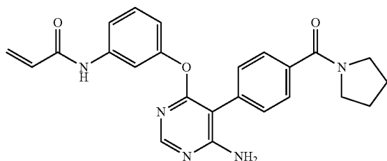
N-(3-((6-amino-5-(4-(pyrrolidine-1-carbonyl)phenyl)pyrimidin-4-yl)oxy)phenyl)acrylamide (A285)
