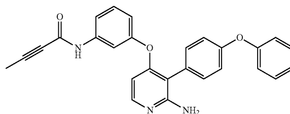
N-(3-(((2-amino-3-(4-phenoxyphenyl)pyridin-4-yl)oxy)phenyl)but-2-ynamide (A340)
