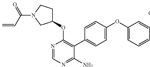
(R)-1-(3-(((6-amino-5-(4-phenoxyphenyl)pyrimidin-4-yl)oxy)methyl)pyrrolidin-1-yl)prop-2-en-1-one (A19)
