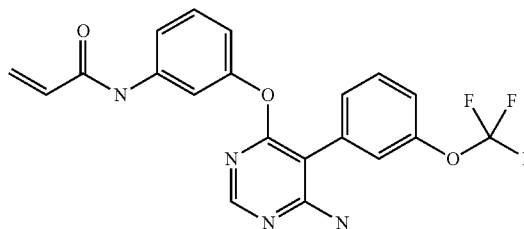
N-(3-((6-amino-5-(3-(trifluoromethoxy)phenyl)pyrimidin-4-yl)oxy)phenyl)acrylamide (A164)
