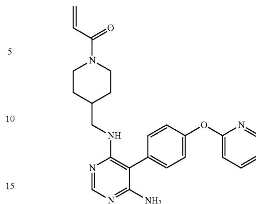
1-(4-(((6-amino-5-(4-(pyridin-2-yloxy)phenyl)pyrimidin-4-yl)amino)methyl)piperidin-1-yl)prop-2-en-1-one (A335)
