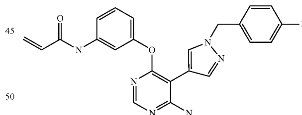
N-(3-((6-amino-5-(1-(4-fluorobenzyl)-1H-pyrazol-4-yl)pyrimidin-4-yl)oxy)phenyl)acrylamide (A187)
