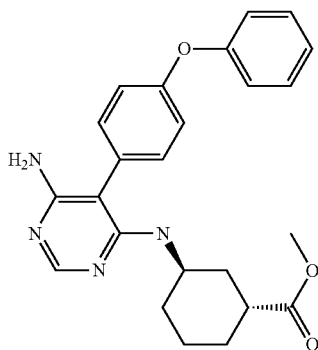
Trans-3-(6-amino-5-(4-phenoxyphenyl)-pyrimidin-4-ylamino)-cyclohexanecarboxylic acid methyl ester (A132)
