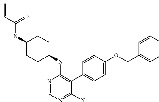
N-cis-4-((6-amino-5-(4-(benzyloxy)phenyl)pyrimidin-4-yl)amino)cyclohexylacrylamide (A154)
