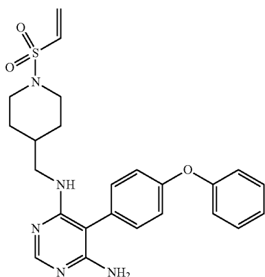
5-(4-phenoxyphenyl)-N4-((1-(vinylsulfonyl)piperidin-4-yl)methyl)pyrimidine-4,6-diamine (A10)
