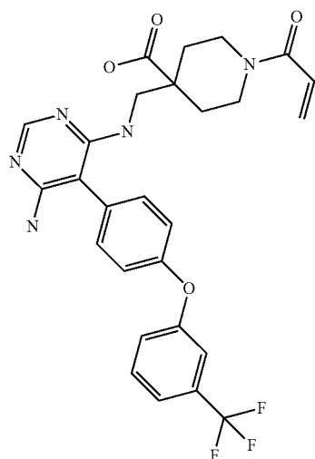
1-acryloyl-4-(((6-amino-5-(4-(3-(trifluoromethyl)phenoxy)phenyl)pyrimidin-4-yl)amino)methyl)piperidine-4-carboxylic acid (A239)
