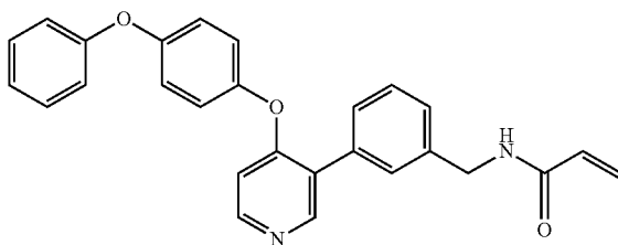
N-(3-(4-(4-phenoxyphenoxy)pyridin-3-yl)benzyl)acrylamide (A302)
