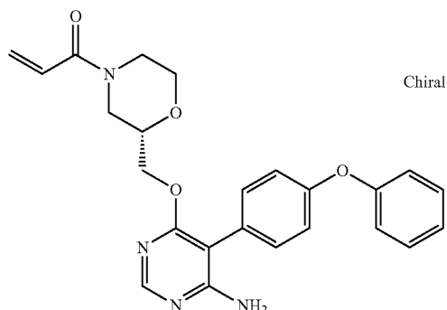
(S)-1-(2-(((6-amino-5-(4-phenoxyphenyl)pyrimidin-4-yl)oxy)methyl)morpholino)prop-2-en-1-one (A65)
