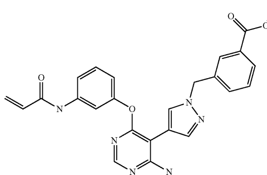
methyl 3-((4-(4-(3-acrylamidophenoxy)-6-aminopyrimidin-5-yl)-1H-pyrazol-1-yl)methyl)benzoate (A206)
