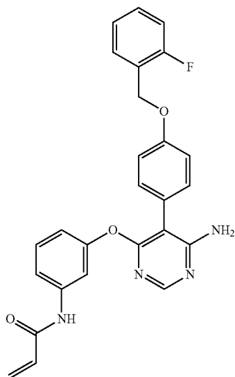
N-(3-{6-Amino-5-[4-(2-fluorobenzyloxy)-phenyl]-pyrimidin-4-yloxy}-phenyl)-acrylamide (A343)
