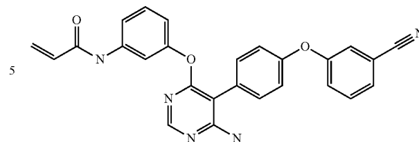
N-(3-((6-amino-5-(4-(3-cyanophenoxy)phenyl)pyrimidin-4-yl)oxy)phenyl)acrylamide (A213)
