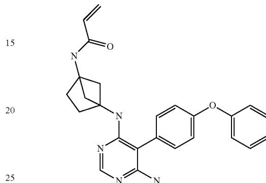
N-((1R,3S)-3-((6-amino-5-(4-phenoxyphenyl)pyrimidin-4-yl)amino)bicyclo[2.1.1]hexan-1-yl)acrylamide (A177)
