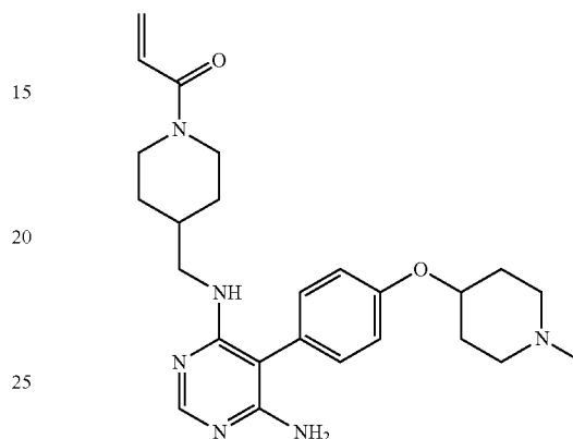
1-(4-(((6-amino-5-(4-((1-methylpiperidin-4-yl)oxy)phenyl)pyrimidin-4-yl)amino)methyl)piperidin-1-yl)prop-2-en-1-one (A89)
