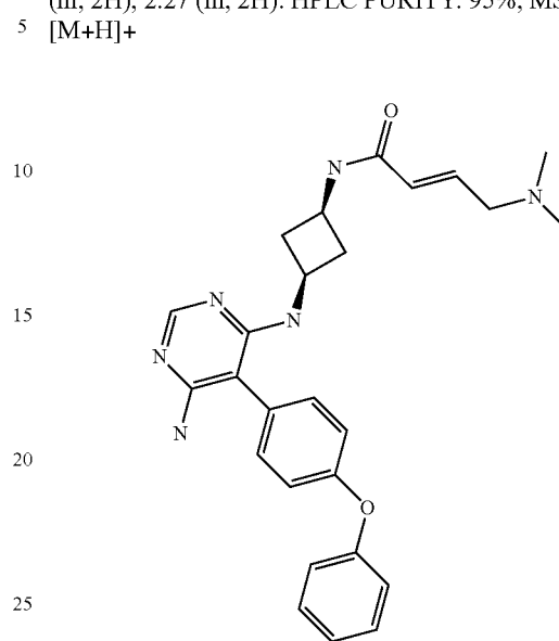
(E)-N-(1,3-cis-3-(((6-amino-5-(4-phenoxyphenyl)pyrimidin-4-yl)amino)cyclobutyl)-4-(dimethylamino)but-2-enamide (A224)
