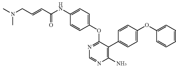
(E)-N-(4-((6-amino-5-(4-phenoxyphenyl)pyrimidin-4-yl)oxy)phenyl)-4-(dimethylamino)but-2-enamide (A290)
