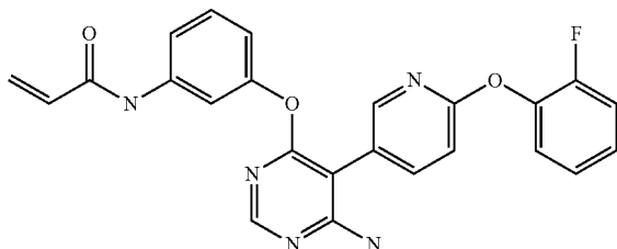
N-(3-((6-amino-5-(6-(2-fluorophenoxy)pyridin-3-yl)pyrimidin-4-yl)oxy)phenyl)acrylamide (A165)
