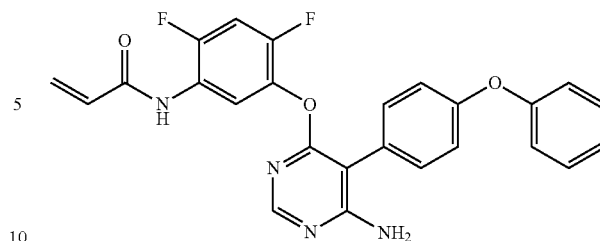
N-(5-(((6-amino-5-(4-phenoxyphenyl)pyrimidin-4-yl)oxy)-2,4-difluorophenyl)acrylamide (A251)
