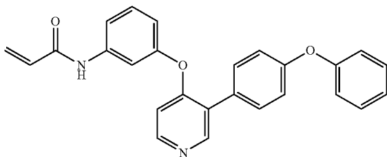
N-(3-((3-(4-phenoxyphenyl)pyridin-4-yl)oxy)phenyl)acrylamide (A270)
