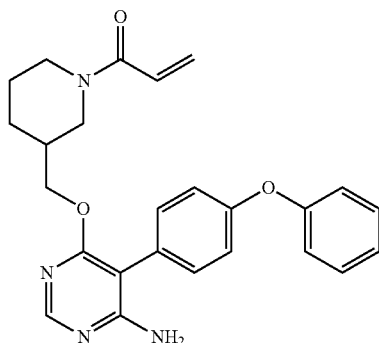
1-(3-(((6-amino-5-(4-phenoxyphenyl)pyrimidin-4-yl)oxy)methyl)piperidin-1-yl)prop-2-en-1-one (A17)
