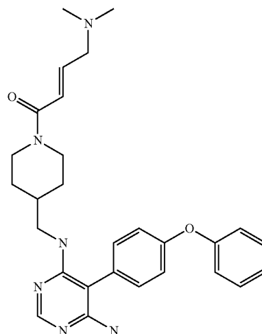
(E)-1-(4-(((6-amino-5-(4-phenoxyphenyl)pyrimidin-4-yl)amino)methyl)piperidin-1-yl)-4-(dimethylamino)but-2-en-1-one (A153)
