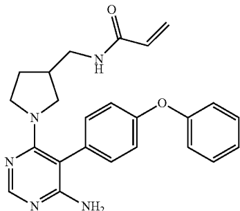
N-((1-(6-amino-5-(4-phenoxyphenyl)pyrimidin-4-yl)piperidin-3-yl)methyl)acrylamide (A5)
