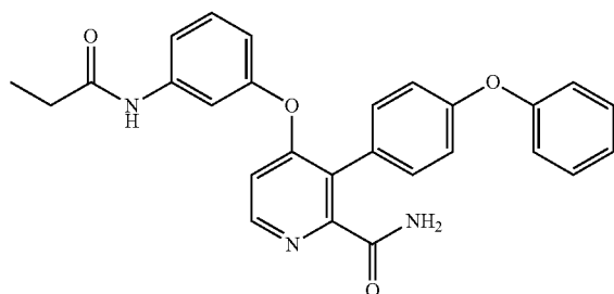
3-(4-phenoxyphenyl)-4-(3-propionamidophenoxy) picolinamide (A328)
