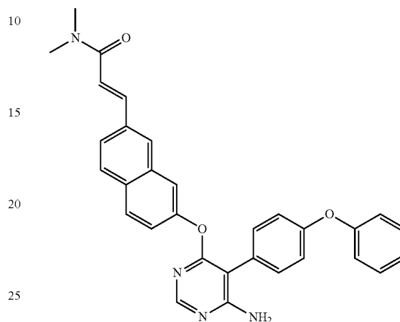
(E)-3-(7-((6-amino-5-(4-phenoxyphenyl)pyrimidin-4-yl) oxy)naphthalen-2-yl)-N,N-dimethylacrylamide (A331)
