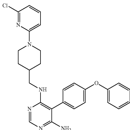
N4-((1-(6-chloropyridin-2-yl)piperidin-4-yl)methyl)-5-(4-phenoxyphenyl)pyrimidine-4,6-diamine (A337)
