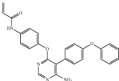
N-(4-((6-amino-5-(4-phenoxyphenyl)pyrimidin-4-yl)oxy)phenyl)acrylamide (A280)
