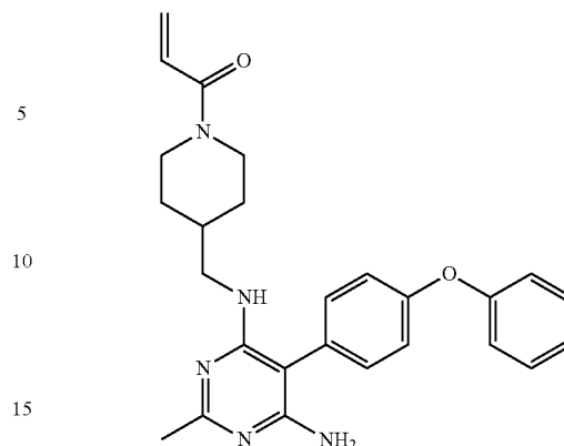
1-(4-(((6-amino-2-methyl-5-(4-phenoxyphenyl)pyrimidin-4-yl)amino)methyl)piperidin-1-yl)prop-2-en-1-one (A36)
