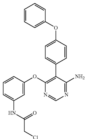
N-{3-[6-Amino-5-(4-phenoxy-phenyl)-pyrimidin-4-yloxy]-phenyl}-2-chloroacetamide (A342)
