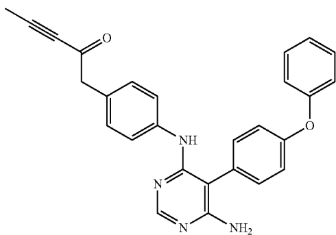
1-(4-(6-Amino-5-(4-phenoxyphenyl)-pyrimidin-4-ylamino)-phenyl)-pent-3-yn-2-one
