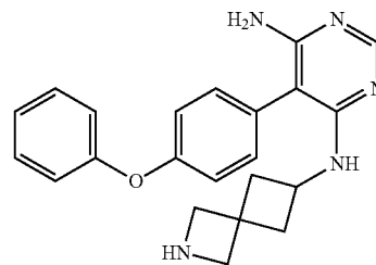
5-(4-phenoxyphenyl)-N 4 -(2-azaspiro[3.3]heptan-6-yl)pyrimidine-4,6-diamine
