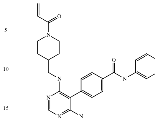
4-(4-(((1-acryloylpiperidin-4-yl)methyl)amino)-6-aminopyrimidin-5-yl)-N-phenylbenzamide (A157)
