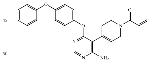
1-(4-(4-amino-6-(4-phenoxyphenoxy)pyrimidin-5-yl)-5,6-dihydropyridin-1(2H)-yl)prop-2-en-1-one (A263)
