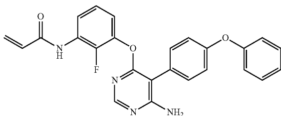
N-(3-((6-amino-5-(4-phenoxyphenyl)pyrimidin-4-yl)oxy)-2-fluorophenyl)acrylamide (A240)
