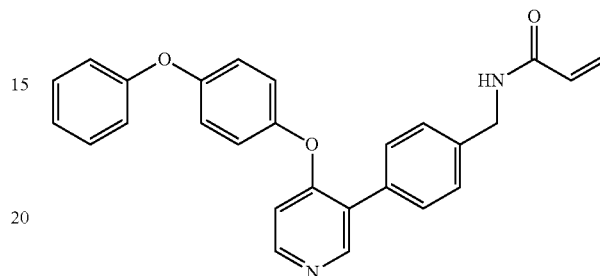
1-(3-((5-(4-phenoxyphenyl)pyrimidin-4-yl)amino)piperidin-1-yl)prop-2-en-1-one (A284)
