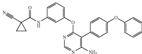
N-(3-((6-amino-5-(4-phenoxyphenyl)pyrimidin-4-yl) oxy)phenyl)-1-cyanocyclopropanecarboxamide (A329)
