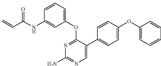
N-(3-((2-amino-5-(4-phenoxyphenyl)pyrimidin-4-yl)oxy)phenyl)acrylamide (A271)
