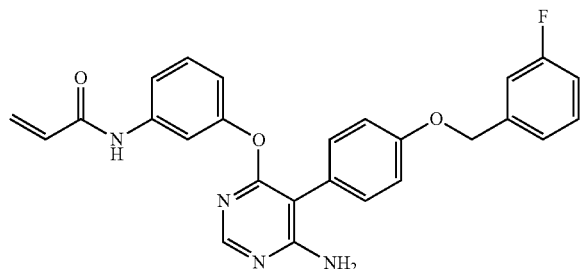
N-(3-(((6-amino-5-(4-(3-fluorobenzyl)oxy)phenyl)pyrimidin-4-yl)oxy)phenyl)acrylamide (A260)
