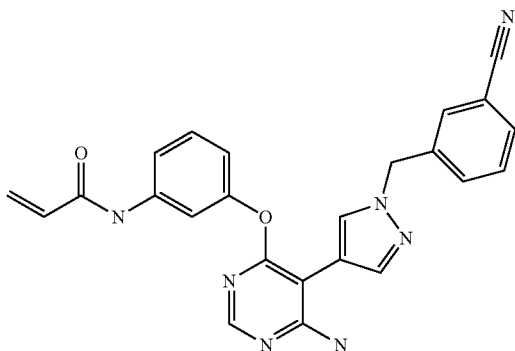
N-(3-((6-amino-5-(1-(3-cyanobenzyl)-1H-pyrazol-4-yl)pyrimidin-4-yl)oxy)phenyl)acrylamide (A203)
