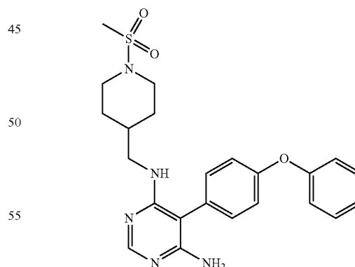
N4-((1-(methylsulfonyl)piperidin-4-yl)methyl)-5-(4-phenoxyphenyl)pyrimidine-4,6-diamine (A55)
