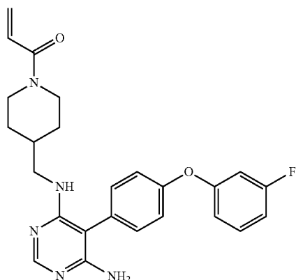
1-(4-(((6-amino-5-(4-(3-fluorophenoxy)phenyl)pyrimidin-4-yl)amino)methyl)piperidin-1-yl)prop-2-en-1-one (A34)
