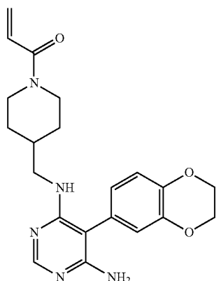
1-(4-(((6-amino-5-(2,3-dihydrobenzo[b][1,4]dioxin-6-yl)pyrimidin-4-yl)amino)methyl)piperidin-1-yl)prop-2-en-1-one (A84)
