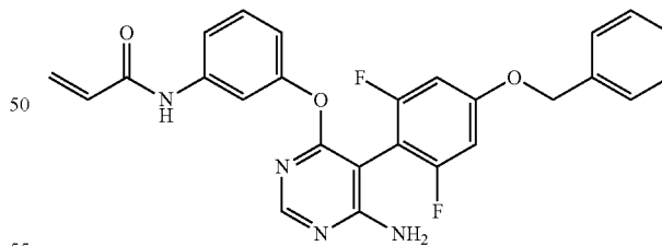
N-(3-((6-amino-5-(4-(benzyloxy)-2,6-difluorophenyl)pyrimidin-4-yl)oxy)phenyl)acrylamide (A294)
