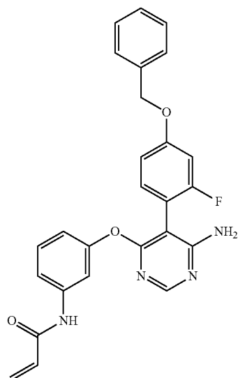
N-{3-[6-Amino-5-(4-benzyloxy-2-fluoro-phenyl)-pyrimidin-4-yloxy]-phenyl}-acrylamide (A349)
