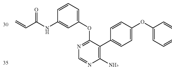
N-(3-((6-amino-5-(4-phenoxyphenyl)pyrimidin-4-yl)oxy)phenyl)acrylamide (A242)
