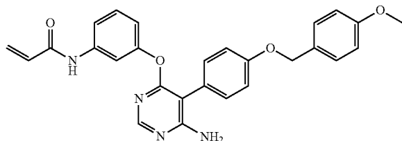
N-(3-((6-amino-5-(4-((4-methoxybenzyl)oxy)phenyl)pyrimidin-4-yl)oxy)phenyl)acrylamide (A264)
