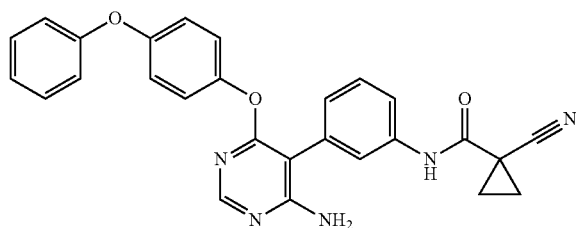
N-(3-(4-amino-6-(4-phenoxyphenoxy)pyrimidin-5-yl) phenyl)-1-cyanocyclopropanecarboxamide (A330)
