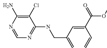
3-((6-Amino-5-chloro-pyrimidin-4-ylamino)-methyl)-benzoic acid methyl ester (A128)
