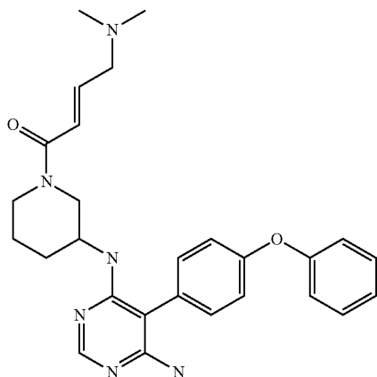
(E)-1-(3-((6-amino-5-(4-phenoxyphenyl)pyrimidin-4-yl)amino)piperidin-1-yl)-4-(dimethylamino)but-2-en-1-one (A160)
