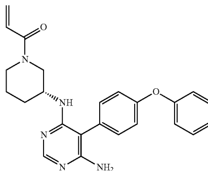
(R)-1-(3-((6-amino-5-(4-phenoxyphenyl)pyrimidin-4-yl)amino)piperidin-1-yl)prop-2-en-1-one (A247)
