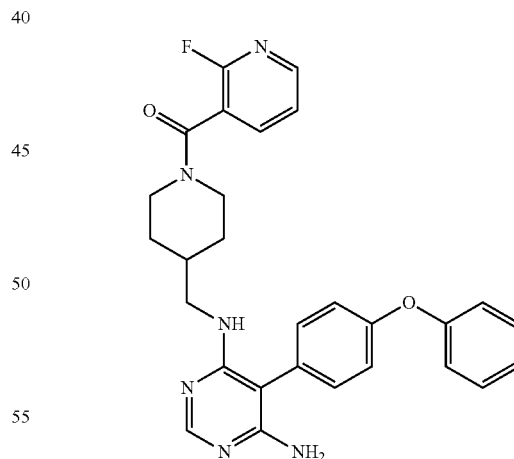
4-(((6-amino-5-(4-phenoxyphenyl)pyrimidin-4-yl)amino)methyl)piperidin-1-yl(2-fluoropyridin-3-yl)methanone (A12)
