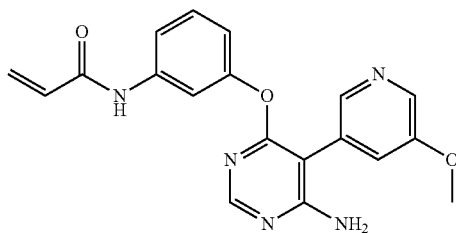
N-(3-((6-amino-5-(5-methoxypyridin-3-yl)pyrimidin-4-yl)oxy)phenyl)acrylamide (A291)
