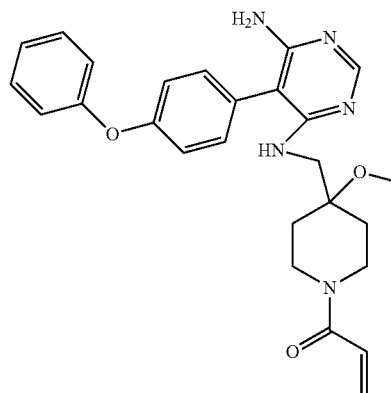
1-(4-(((6-amino-5-(4-phenoxyphenyl)pyrimidin-4-yl)amino)methyl)-4-methoxypiperidin-1-yl)prop-2-en-1-one (A121)
