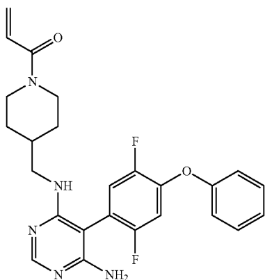
1-(4-(((6-amino-5-(2,5-difluoro-4-phenoxyphenyl)pyrimidin-4-yl)amino)methyl)piperidin-1-yl)prop-2-en-1-one (A87)
