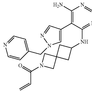
1-(6-((6-amino-5-(1-(pyridin-4-ylmethyl)-1H-pyrazol-4-yl)pyrimidin-4-yl)amino)-2-azaspiro[3.3]heptan-2-yl)prop-2-en-1-one (A116)
