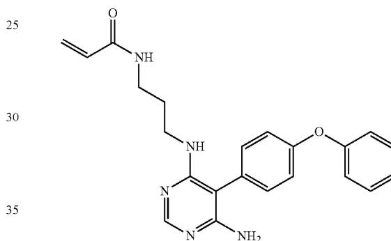
N-(3-((6-amino-5-(4-phenoxyphenyl)pyrimidin-4-yl)amino)propyl)acrylamide (A59)
