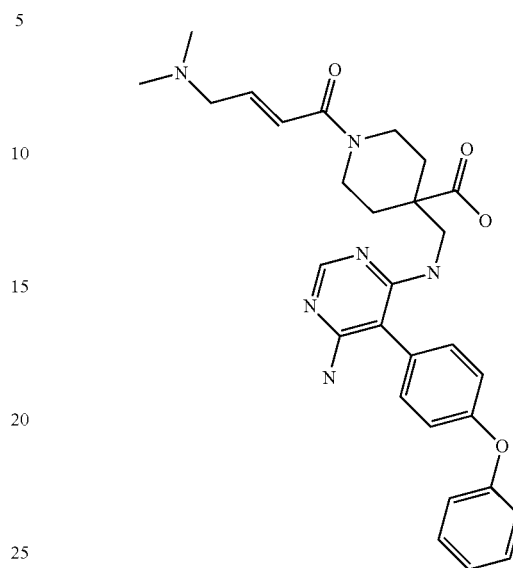
(E)-4-(((6-amino-5-(4-phenoxyphenyl)pyrimidin-4-yl)amino)methyl)-1-(4-(dimethylamino)but-2-enoyl)piperidine-4-carboxylic acid (A217)
