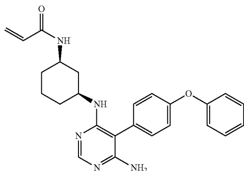
N-(cis-3-((6-amino-5-(4-phenoxyphenyl)pyrimidin-4-yl)amino)cyclohexyl)acrylamide (A51)
