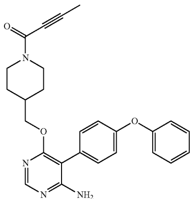
1-(4-(((6-amino-5-(4-phenoxyphenyl)pyrimidin-4-yl)oxy)methyl)piperidin-1-yl)but-2-yn-1-one (A9)
