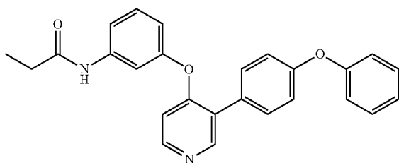
N-(3-((3-(4-phenoxyphenyl)pyridin-4-yl)oxy)phenyl)propionamide (A318)
