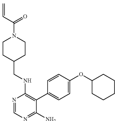
1-(4-(((6-amino-5-(4-(cyclohexyloxy)phenyl)pyrimidin-4-yl)amino)methyl)piperidin-1-yl)prop-2-en-1-one (A99)
