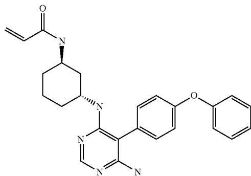
N-((1R,3R)-3-((6-amino-5-(4-phenoxyphenyl)pyrimidin-4-yl)amino)cyclohexyl)acrylamide (A175)
