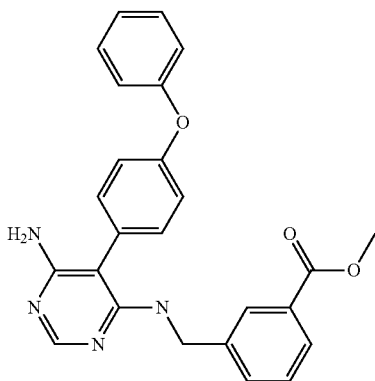
3-((6-Amino-5-(4-phenoxy-phenyl)-pyrimidin-4-ylamino)-methyl)-benzoic acid methyl ester (A131)
