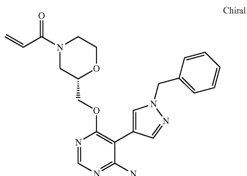
(S)-1-(2-(((6-amino-5-(1-benzyl-1H-pyrazol-4-yl)pyrimidin-4-yl)oxy)methyl)morpholino)prop-2-en-1-one (A193)
