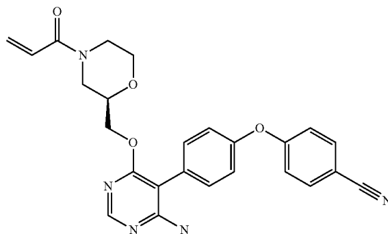
(R)-4-(4-(4-((4-acryloylmorpholin-2-yl)methoxy)-6-aminopyrimidin-5-yl)phenoxy)benzonitrile (A200)
