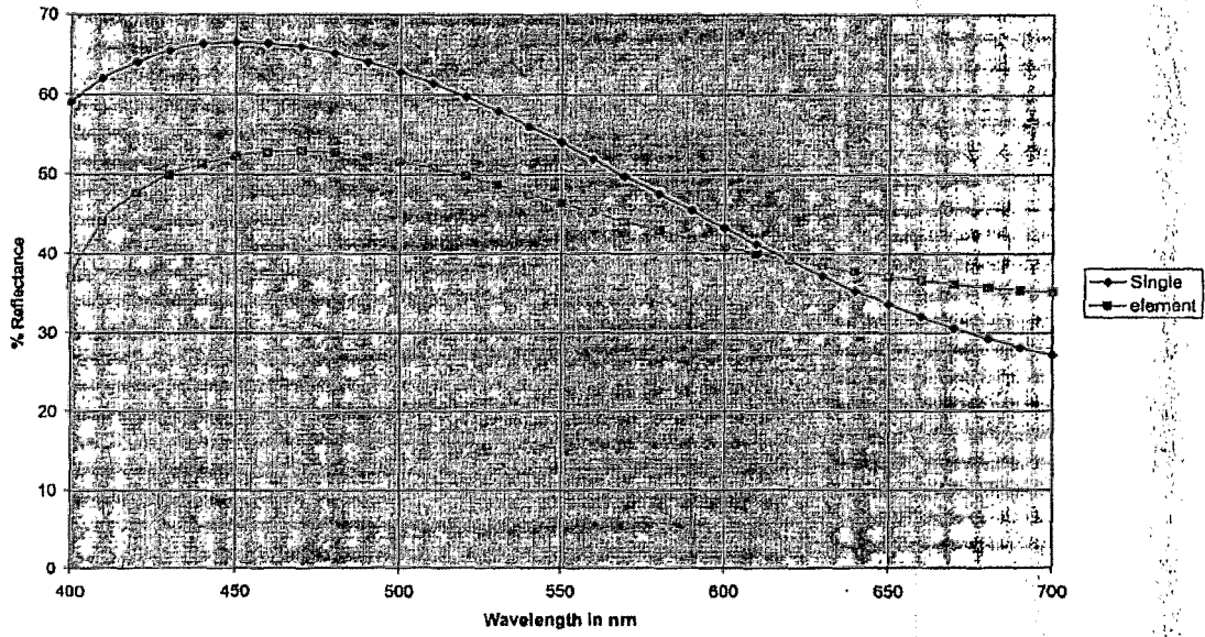
Chrome with 900 Å ITO reflectance on glass and in an element as a 3rd surface reflector electrode
